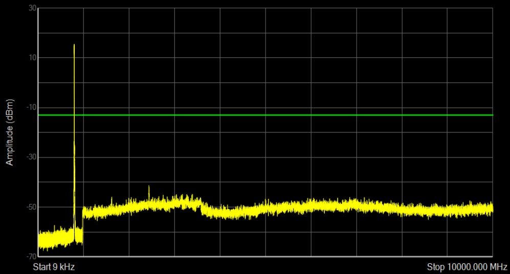
Band26(814-824) QPSK BW=5MHz Channel=26740 RB Size=25 Position=#0
