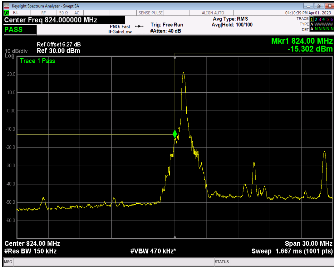
Band26(824-849) QAM16 BW=15MHz Channel=26865 RB Size=1 Position=#Max
