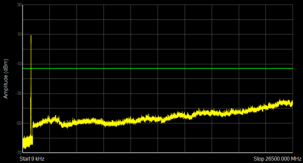
Band26(824-849) QAM16 BW=15MHz Channel=26915 RB Size=75 Position=#0
