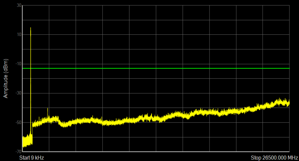
Band26(824-849) QAM16 BW=5MHz Channel=26915 RB Size=25 Position=#0
