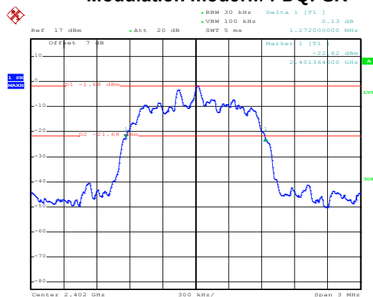
Modulation mode:π/4-DQPSK
