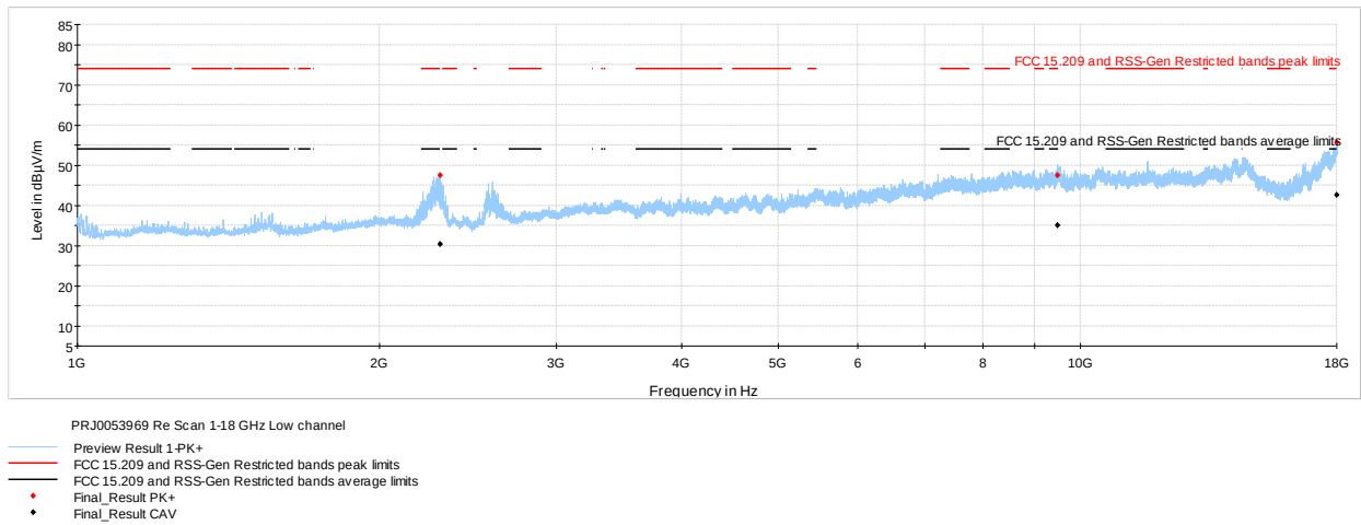
Figure 7.6-12: Radiated spurious emissions (1-18 GHz) on Low channel
