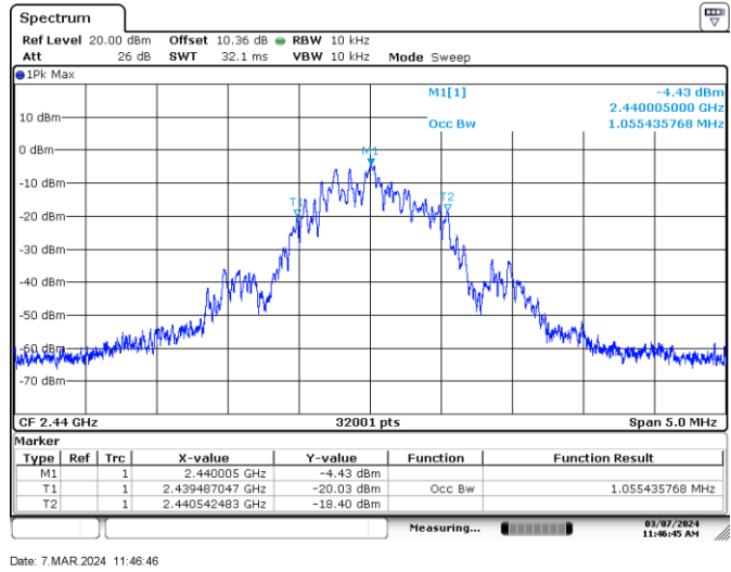
Figure 7.4-5: 99% occupied bandwidth on mid channel
