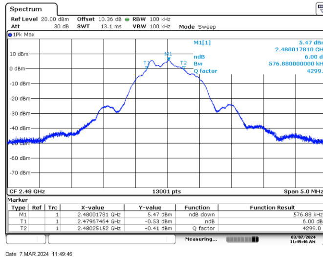
Figure 7.4-3: 6 dB bandwidth on high channel
