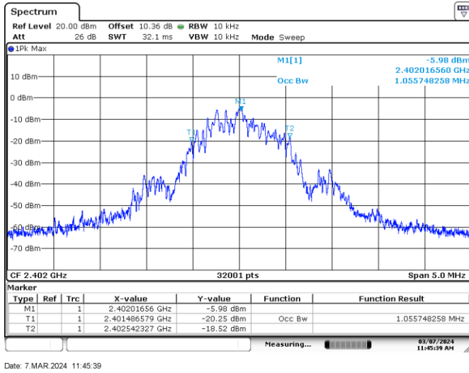
Figure 7.4-4: 99% occupied bandwidth on low channel
