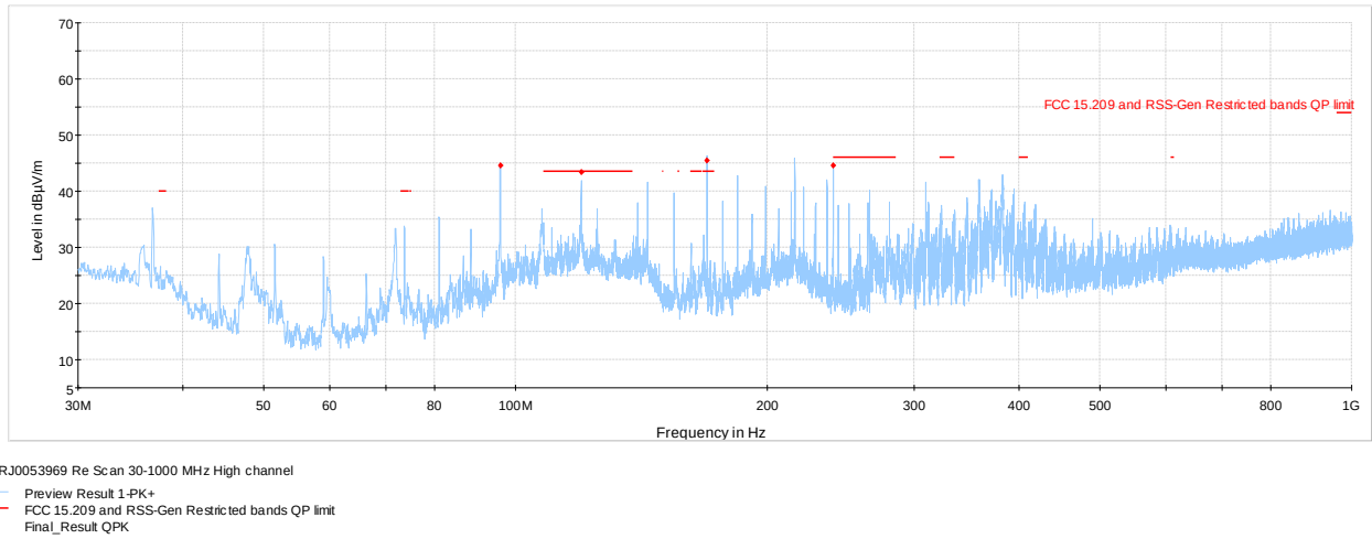
Figure 7.6-11: Radiated spurious emissions (30-1000 MHz) on High channel
