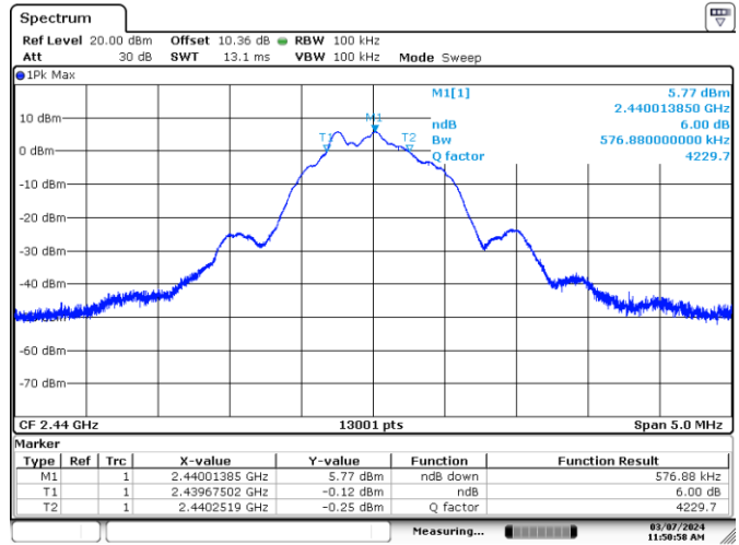
Figure 7.4-2: 6 dB bandwidth on mid channel
