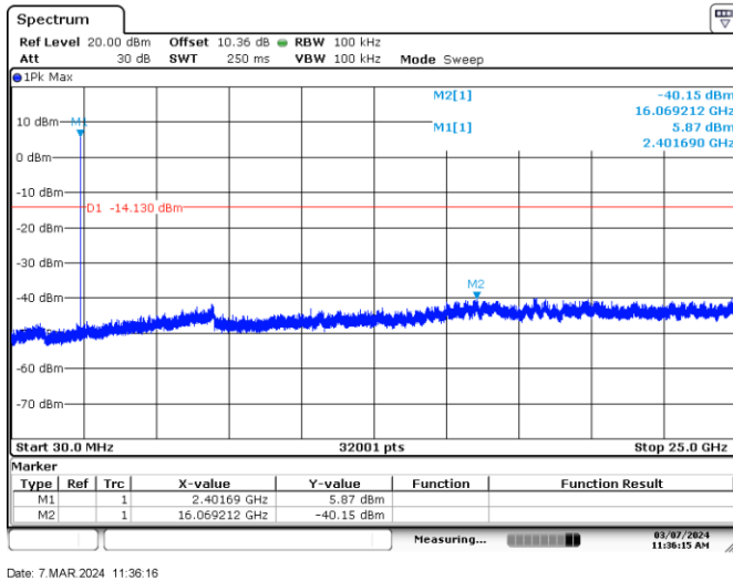
Figure 7.6-6: Conducted spurious emissions on low channel
