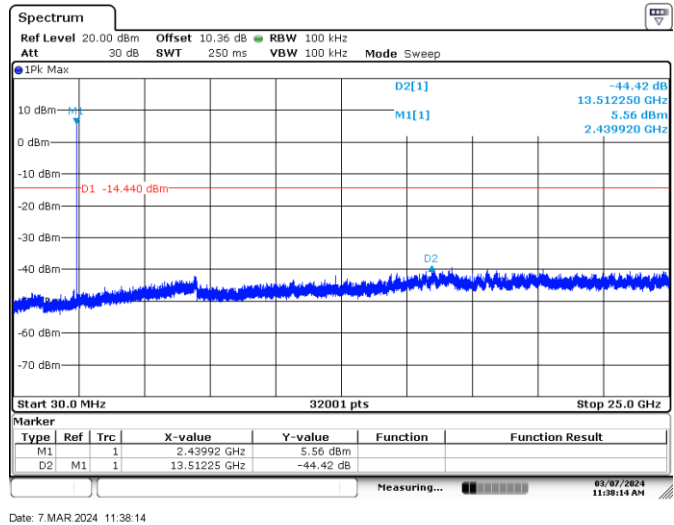
Figure 7.6-7: Conducted spurious emissions on mid channel
