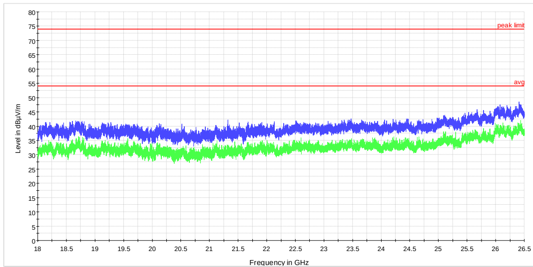
Figure 7.6-15: Radiated spurious emissions (18-26 GHz) on Low channel
