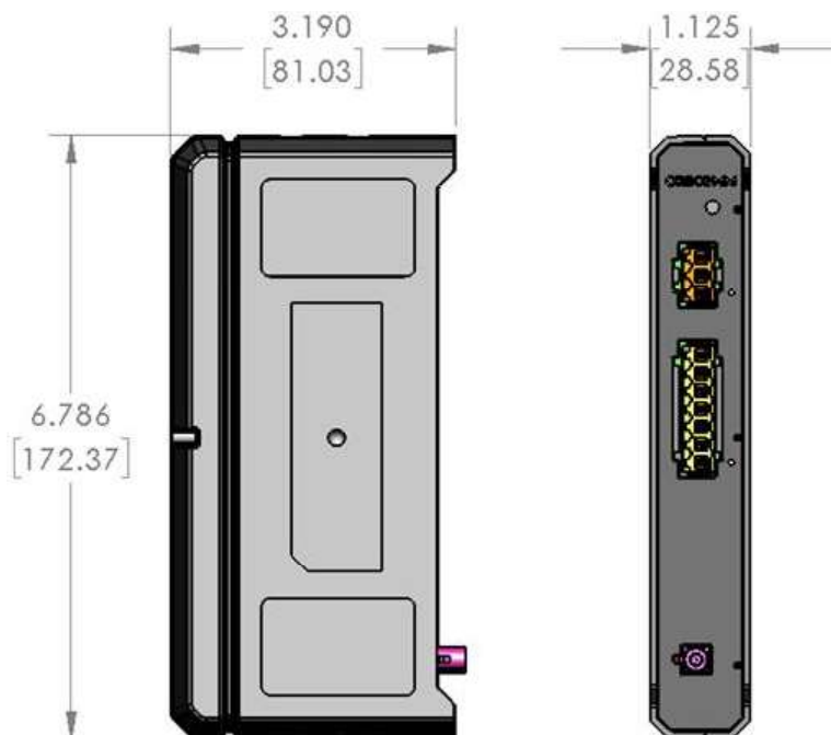
Figure 2: CT 3600 Dimensions
