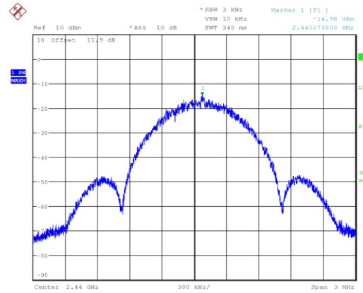
Figure 7.7-2: PSD on mid channel BLE 2 (1M)
