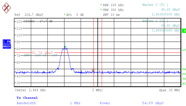
Figure 7.6-12: Radiated band edge at restricted band a 2483.5 MHz (Peak) BLE 2 (1M)
