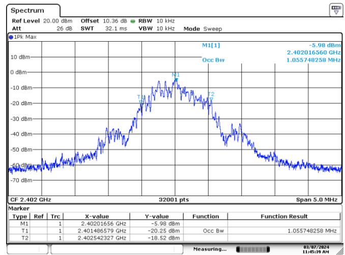
Figure 7.4-16: 99% occupied bandwidth on Low channel (1M BLE 1)
