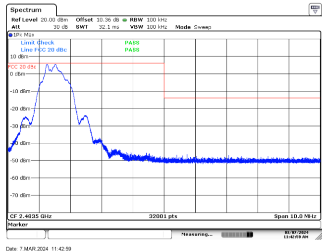
Figure 7.6-37: Conducted band edge at non-restricted band at 2483.5 MHz (BLE 1)
