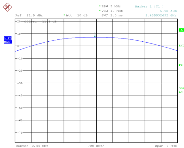
Figure 7.5-11: Output power on mid channel (2M BLE 1)
