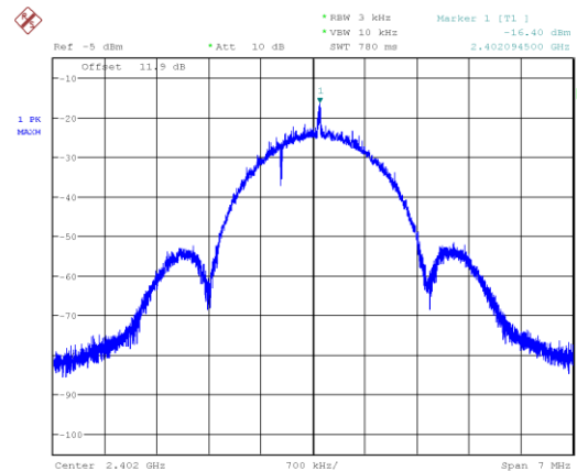
Figure 7.7-4: PSD on low channel BLE 2 (2M)
