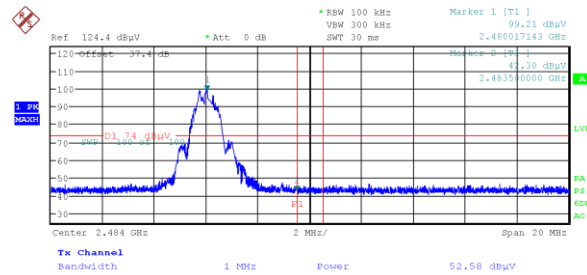
Figure 7.6-20: Radiated band edge at restricted band a 2483.5 MHz (Peak) BLE 1(1M)
