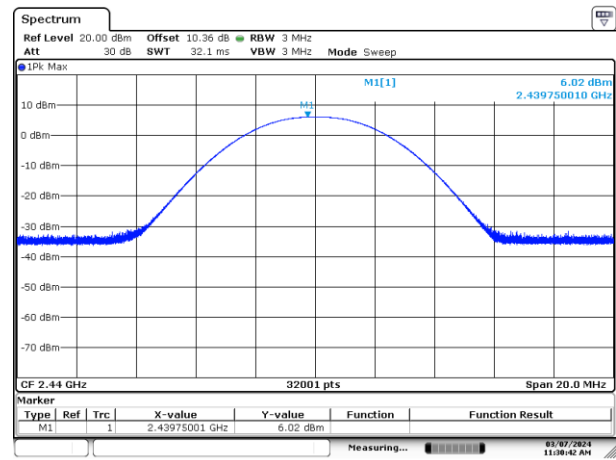
Figure 7.5-8: Output power on mid channel (1M BLE 1)
