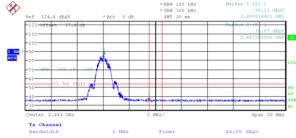
Figure 7.6-21: Radiated band edge at restricted band at 2483.5 MHz (Average) BLE 1(1M)
