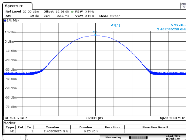
Figure 7.5-7: Output power on low channel (1M BLE 1)
