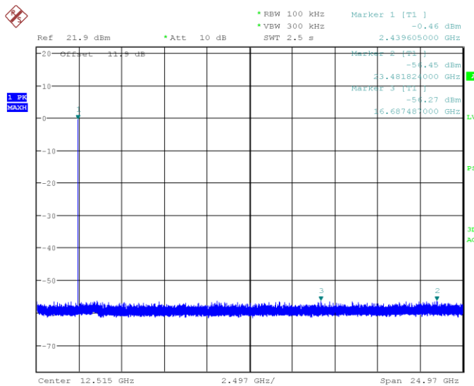
Figure 7.6-34: Conducted spurious emissions at Mid Channel (BLE 2.2M)
