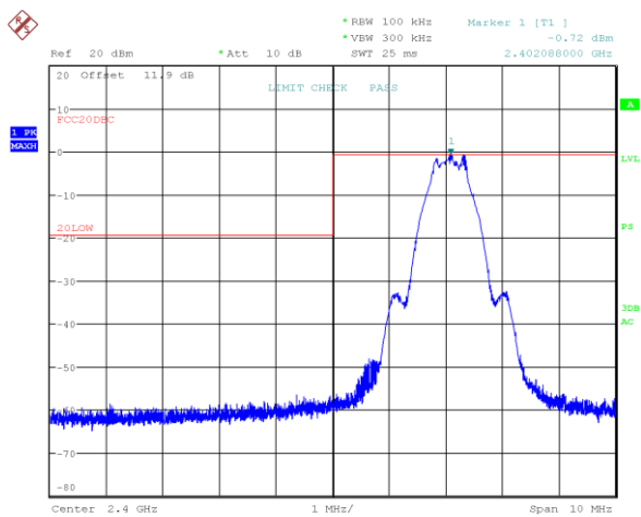
Figure 7.6-26: Conducted band edge at non-restricted band at 2400 MHz (BLE 2 1M)
