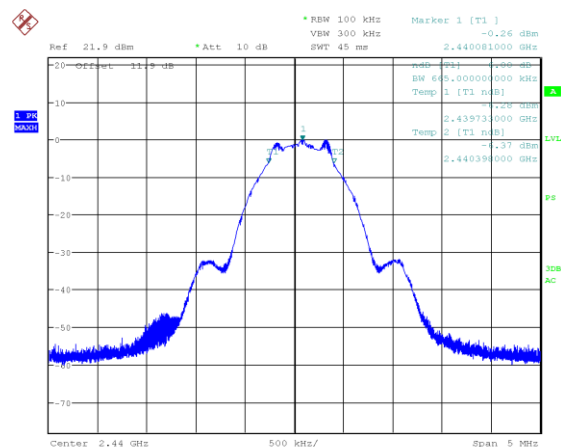
Figure 7.4-2: 6 dB bandwidth on Mid channel (1M BLE 2)
