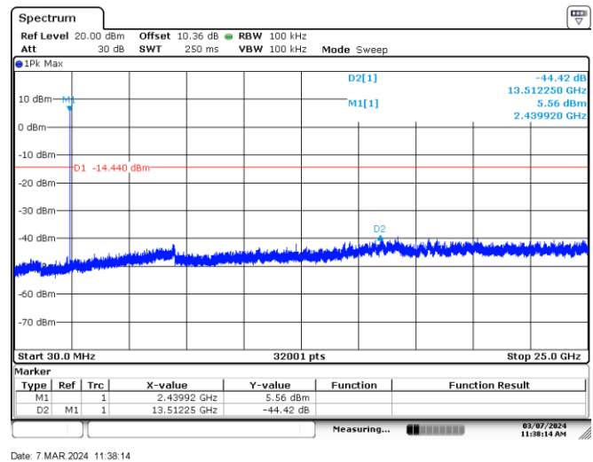
Figure 7.6-39: Conducted spurious emissions on mid channel (BLE 1)
