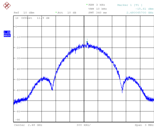
Figure 7.7-3: PSD on high channel BLE 2 (1M)
