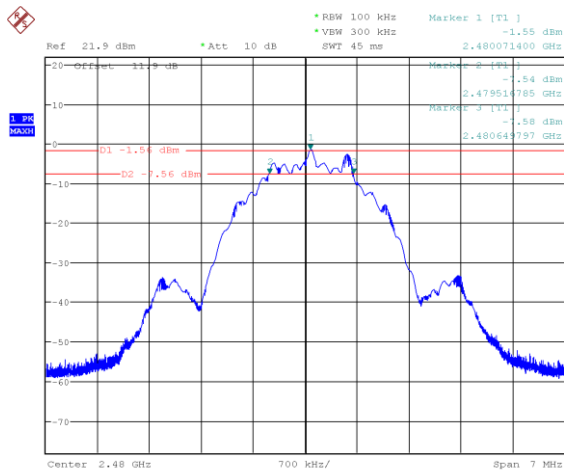
Figure 7.4-9: 6 dB bandwidth on High channel (2M BLE 2)
