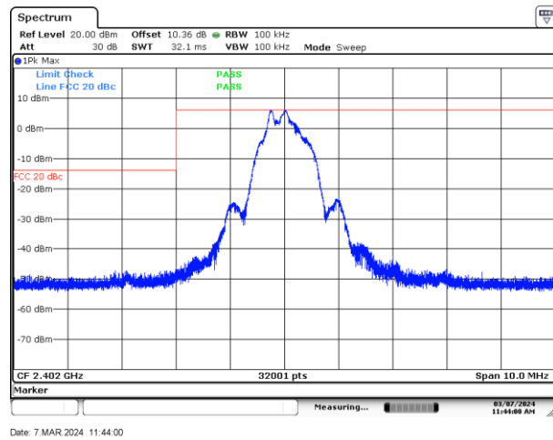
Figure 7.6-36: Conducted band edge at non-restricted band at 2400 MHz (BLE 1)
