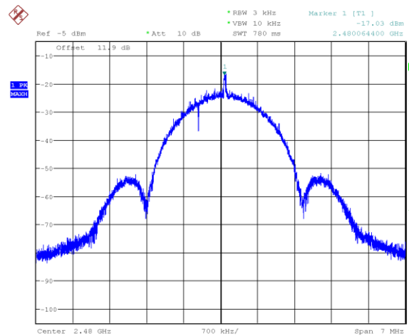
Figure 7.7-6: PSD on high channel BLE 2 (2M)
