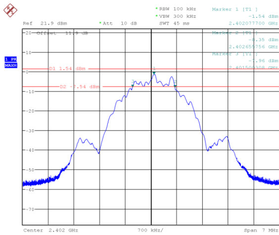
Figure 7.4-7: 6 dB bandwidth on Low channel (2M BLE 2)
