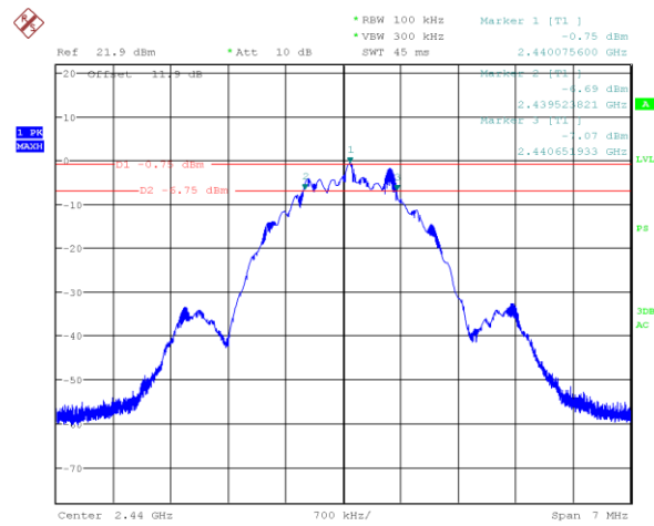
Figure 7.4-8: 6 dB bandwidth on Mid channel (2M BLE 2)
