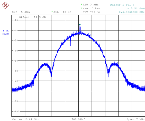
Figure 7.7-5: PSD on mid channel BLE 2 (2M)
