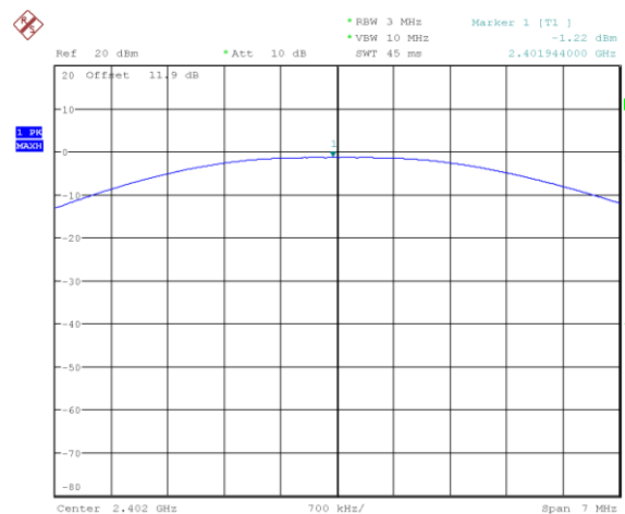
Figure 7.5-4: Output power on low channel (2M BLE 2)
