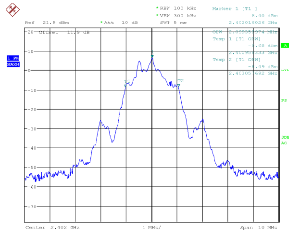
Figure 7.4-22: 99% occupied bandwidth on Low channel (1M BLE 1)
