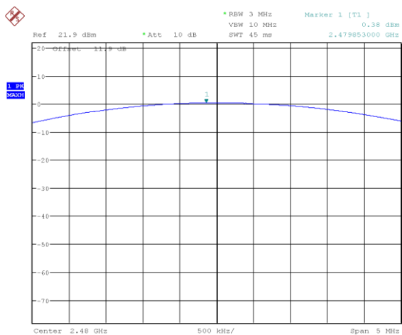
Figure 7.5-3: Output power on High channel (1M BLE 2)
