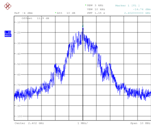
Figure 7.7-10: PSD on low channel BLE 2 (2M)
