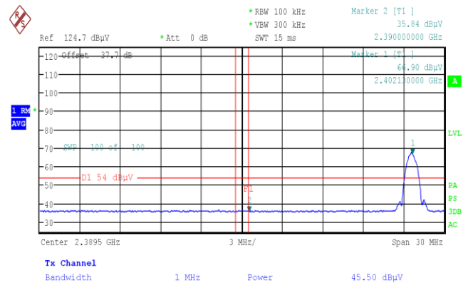
Figure 7.6-11: Radiated band edge at restricted band at 2390 MHz (Average) BLE 2 (1M)
