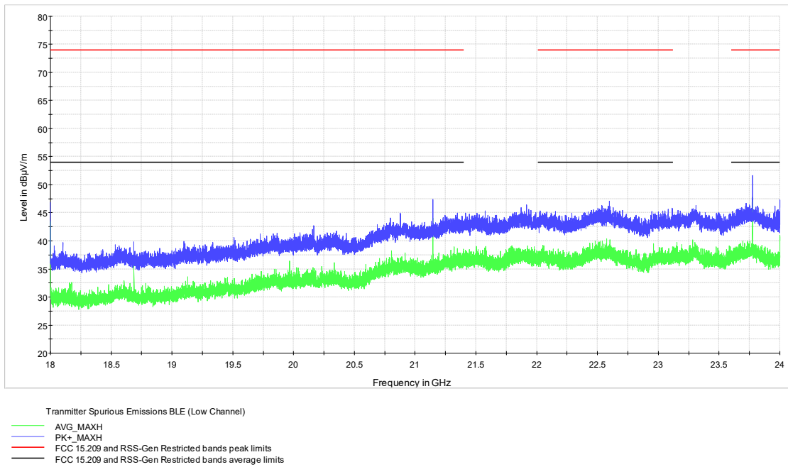
Figure 7.6-7: Radiated spurious emissions (18-24 GHz ) on Low Channel (BLE 2 and BLE 1)
