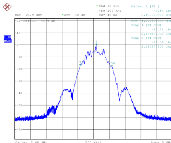
Figure 7.4-6: 99% occupied bandwidth on High channel (1M BLE 2)
