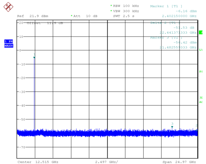
Figure 7.6-33: Conducted spurious emissions at Low Channel (BLE 2.2M)
