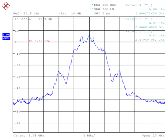
Figure 7.4-21: 6 dB bandwidth on High channel (2M BLE 1)
