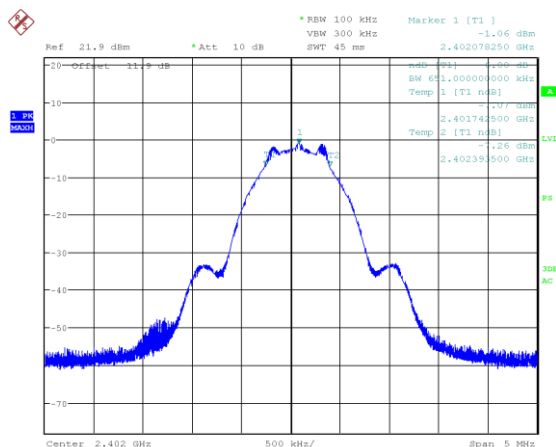
Figure 7.4-1: 6 dB bandwidth on Low channel (1M BLE 2)
