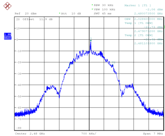
Figure 7.4-12: 99% occupied bandwidth on High channel (2M BLE 2)
