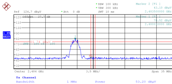
Figure 7.6-16: Radiated band edge at restricted band a 2483.5 MHz (Peak) BLE 2 (2M)
