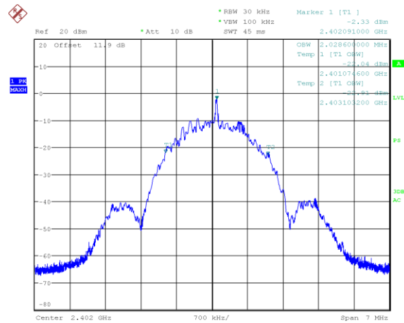
Figure 7.4-10: 99% occupied bandwidth on Low channel (2M BLE 2)
