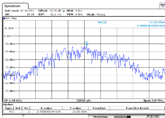
Figure 7.7-9: PSD on high channel BLE 1 (1M)
