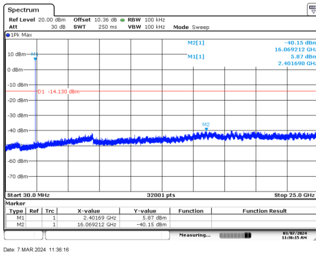
Figure 7.6-38: Conducted spurious emissions on low channel( BLE 1)
