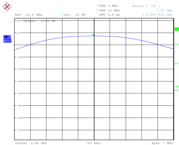
Figure 7.5-12: Output power on high channel (2M BLE 1)
