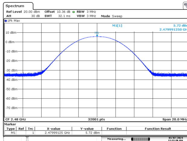
Figure 7.5-9: Output power on high channel (1M BLE 1)
