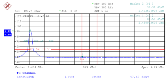
Figure 7.6-17: Radiated band edge at restricted band at 2483.5 MHz (Average) BLE 2 (2M)
