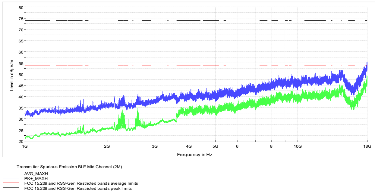
Figure 7.6-5: Radiated spurious emissions (1-18 GHz) on Mid Channel (BLE 2 and BLE 1)
