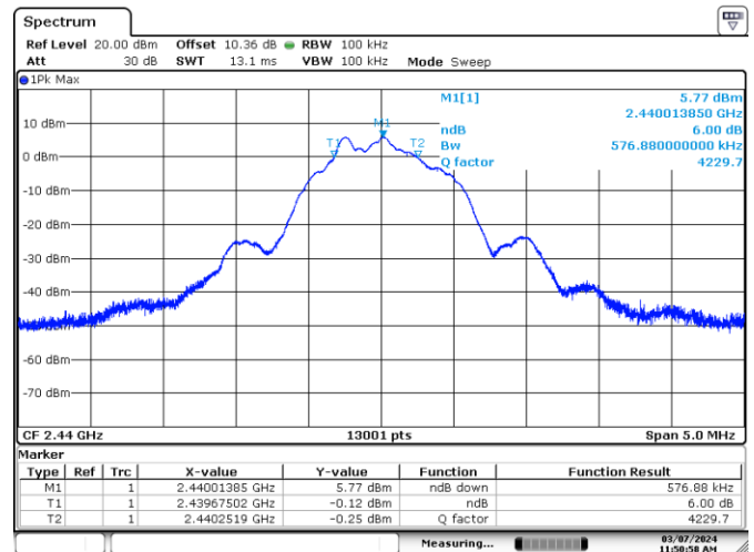
Figure 7.4-14: 6 dB bandwidth on Mid channel (1M BLE 1)
