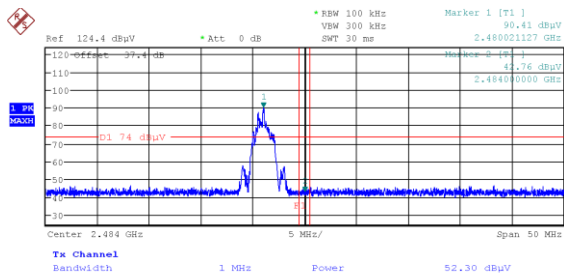
Figure 7.6-24: Radiated band edge at restricted band a 2483.5 MHz (Peak) BLE 1(2M)
