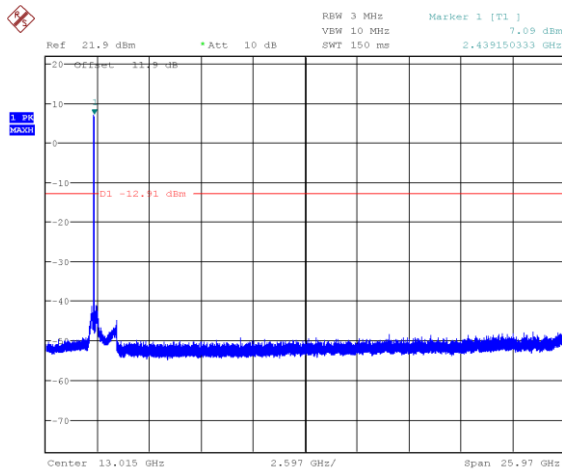
Figure 7.6-40: Conducted spurious emissions on High channel (BLE 1) 1M
