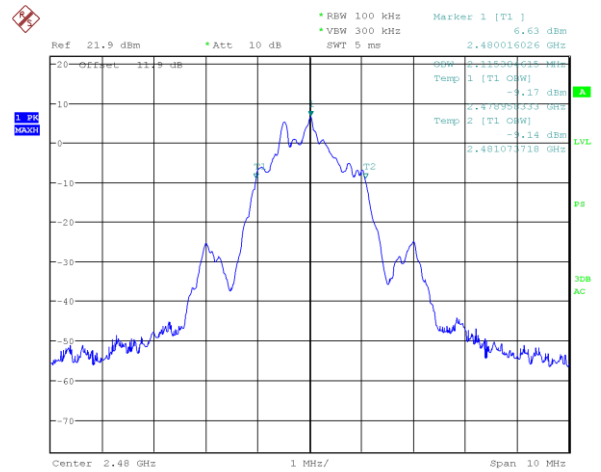
Figure 7.4-24: 99% occupied bandwidth on High channel (2M BLE 1)
