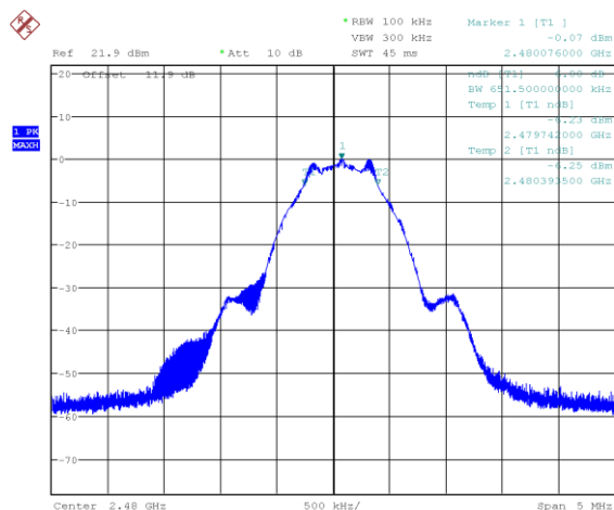
Figure 7.4-3: 6 dB bandwidth on High channel (1M BLE 2)
