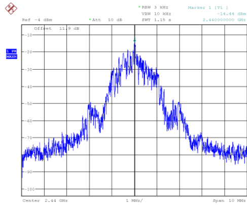
Figure 7.7-11: PSD on mid channel BLE 1 (2M)
