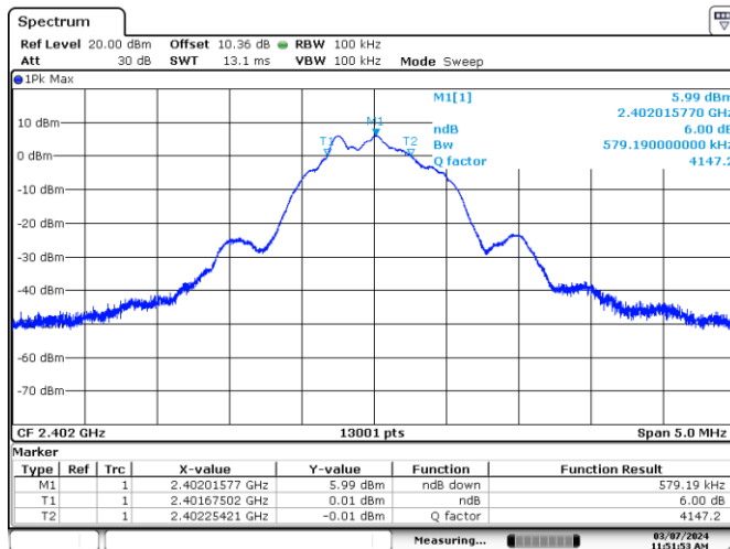
Figure 7.4-13: 6 dB bandwidth on Low channel (1M BLE 1)
