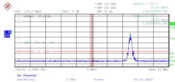
Figure 7.6-19: Radiated band edge at restricted band at 2390 MHz (Average) BLE 1(1M)
