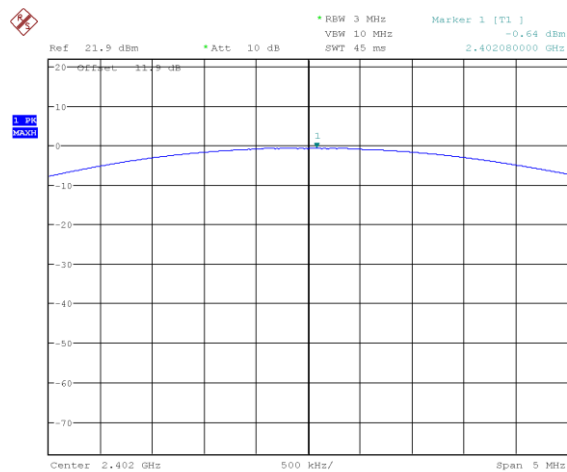
Figure 7.5-1: Output power on low channel (1M BLE 2)
