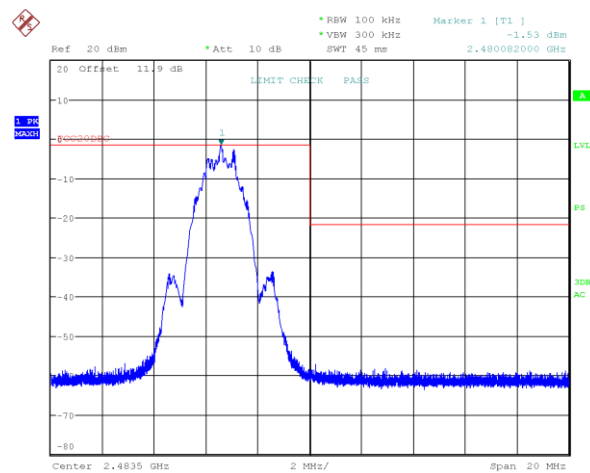
Figure 7.6-29: Conducted band edge at non-restricted band at 2483.5 MHz (BLE 2 2M)
