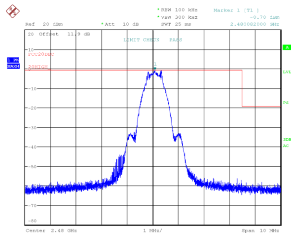
Figure 7.6-27: Conducted band edge at non-restricted band at 2483.5 MHz (BLE 2 1M)
