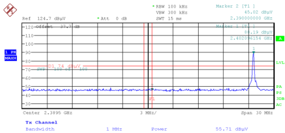
Figure 7.6-14: Radiated band edge at restricted band a 2390 MHz (Peak) BLE 2 (2M)
