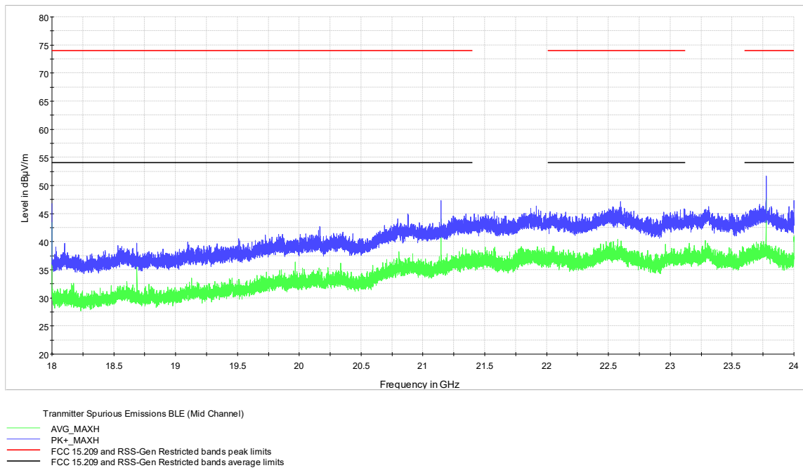
Figure 7.6-8: Radiated spurious emissions (18-24 GHz ) on Mid Channel (BLE GHz) BLE 1)
