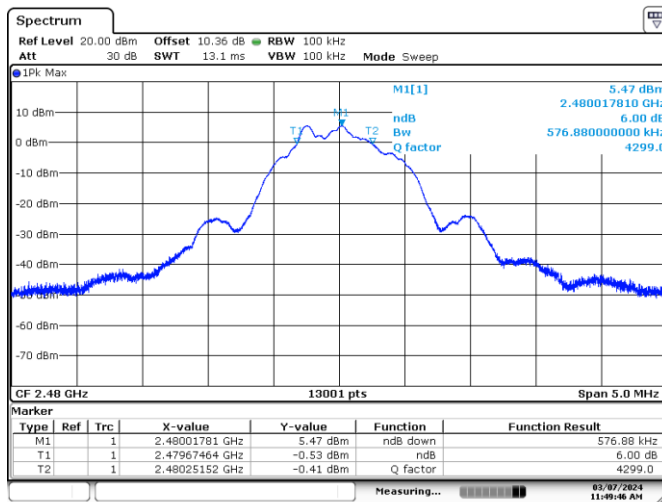
Figure 7.4-15: 6 dB bandwidth on High channel (1M BLE 1)
