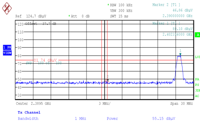
Figure 7.6-10: Radiated band edge at restricted band a 2390 MHz (Peak) BLE 2 (1M)
