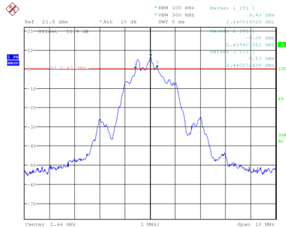
Figure 7.4-20: 6db bandwidth on Mid channel (2M BLE 1)
