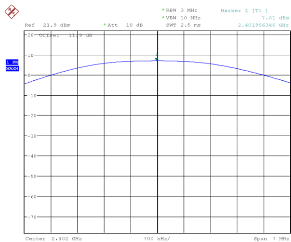
Figure 7.5-10: Output power on low channel (2M BLE 1)
