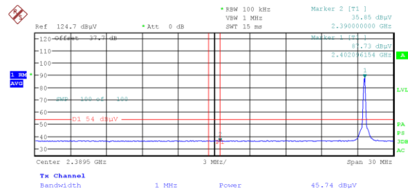
Figure 7.6-15: Radiated band edge at restricted band at 2390 MHz (Average) BLE 2 (2M)
