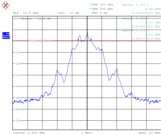
Figure 7.4-19: 6 dB bandwidth on Low channel (2M BLE 1)
