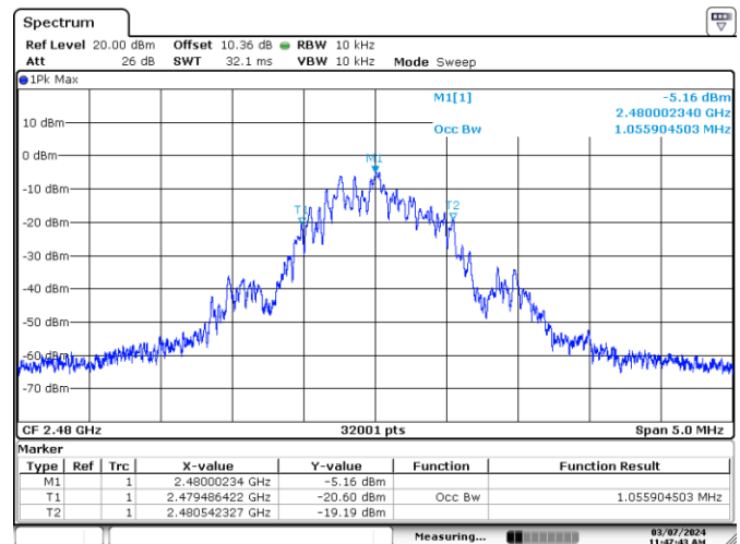
Figure 7.4-18: 99% occupied bandwidth on High channel (1M BLE 1)
