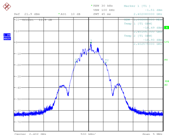
Figure 7.4-4: 99% occupied bandwidth on Low channel (1M BLE 2)
