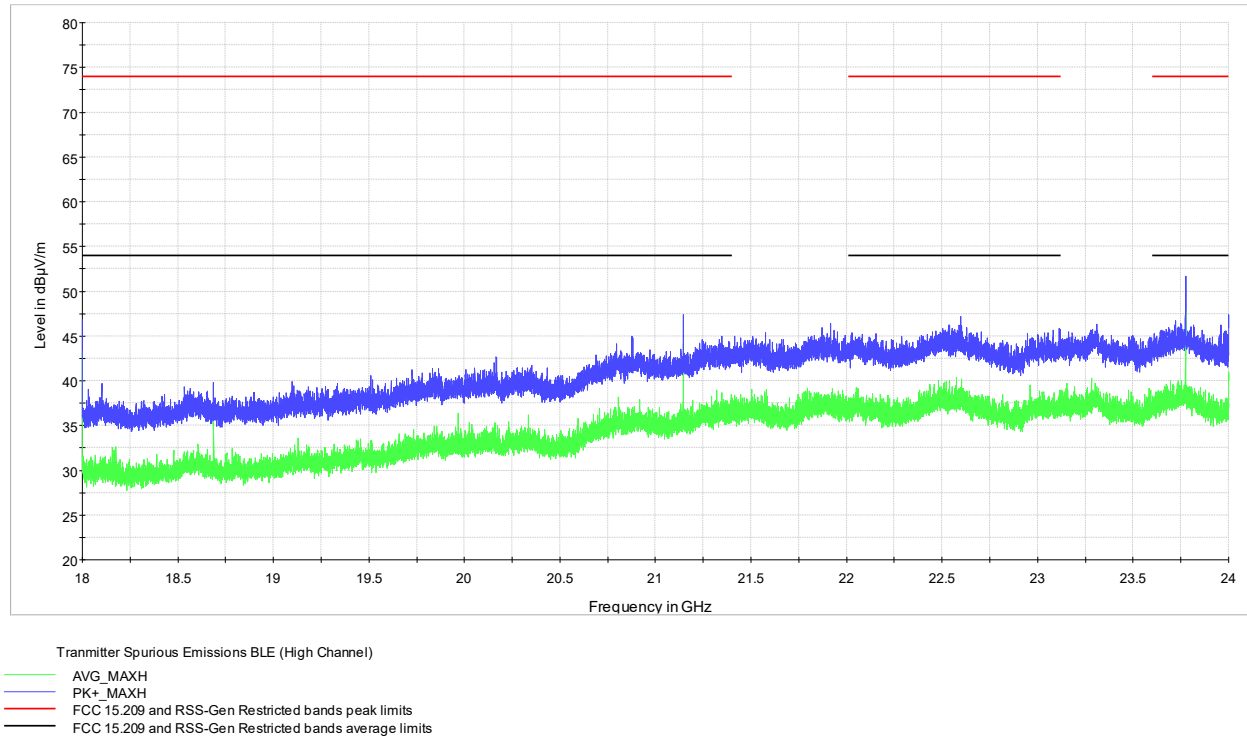
Figure 7.6-9: Radiated spurious emissions (18-24 GHz ) on high Channel (BLE 2 and BLE 1)
