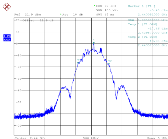
Figure 7.4-5: 99% occupied bandwidth on Mid channel (1M BLE 2)
