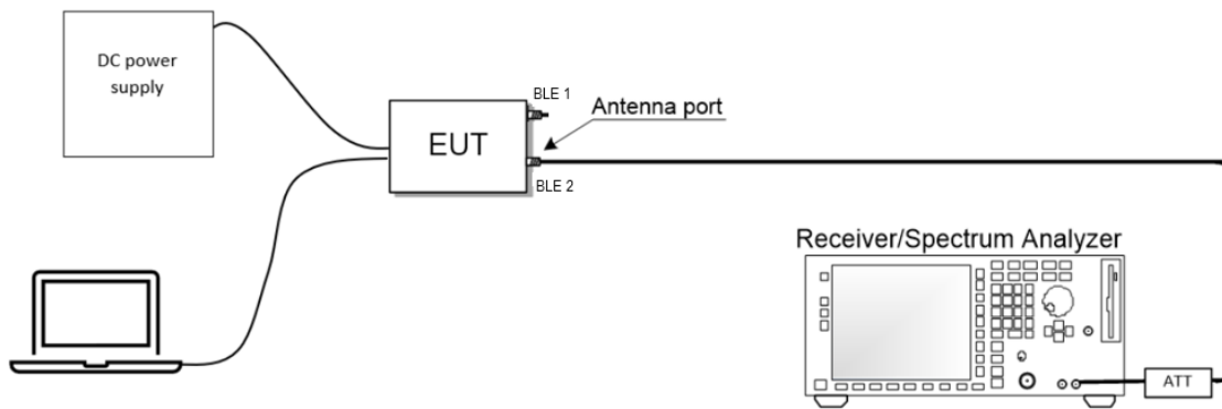
Figure 4.5-2: Antenna port testing block diagram
