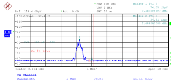
Figure 7.6-25: Radiated band edge at restricted band at 2483.5 MHz (Average) BLE 1(2M)
