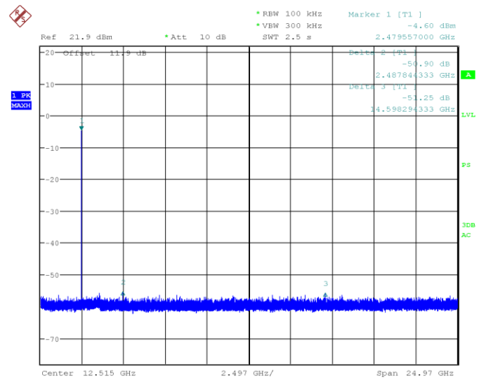
Figure 7.6-35: Conducted spurious emissions at High Channel (BLE 2.2M)
