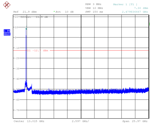
Figure 7.6-41: Conducted spurious emissions on High channel (BLE 1) 2M
