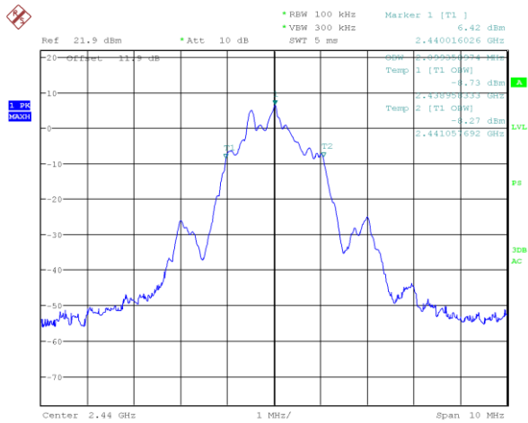
Figure 7.4-23: 99% occupied bandwidth on Mid channel (2M BLE 1)
