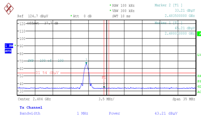
Figure 7.6-13: Radiated band edge at restricted band at 2483.5 MHz (Average) BLE 2 (1M)
