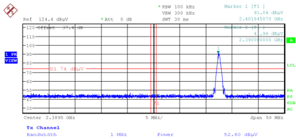
Figure 7.6-18: Radiated band edge at restricted band a 2390 MHz (Peak) BLE 1(1M)
