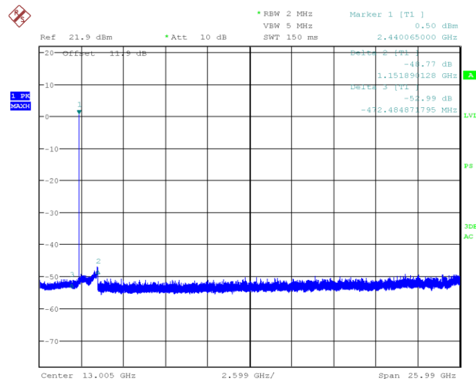
Figure 7.6-31: Conducted spurious emissions at Mid Channel (BLE 2 1M)
