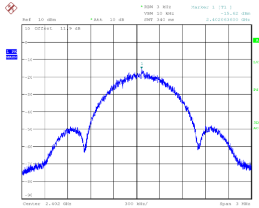
Figure 7.7-1: PSD on low channel BLE 2 (1M)
