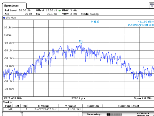
Figure 7.7-7: PSD on low channel BLE 1 (1M)
