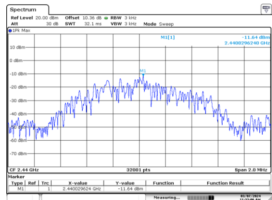
Figure 7.7-8: PSD on mid channel BLE 1
