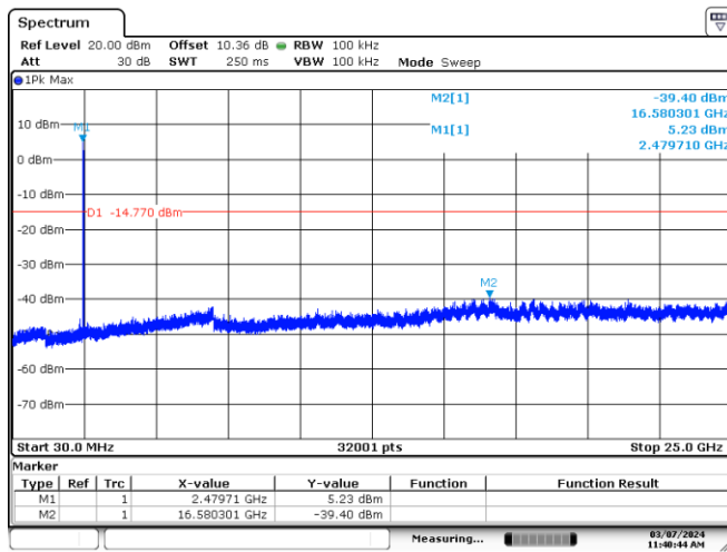
Figure 7.6-40: Conducted spurious emissions on High channel (BLE 1) 1M
