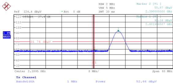
Figure 7.6-22: Radiated band edge at restricted band a 2390 MHz (Peak) BLE 1 (2M)
