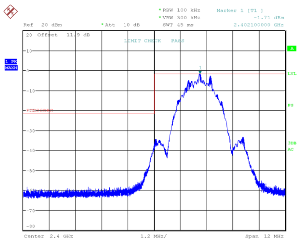
Figure 7.6-28: Conducted band edge at non-restricted band at 2400 MHz (BLE 2 2M)
