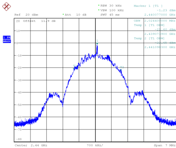
Figure 7.4-11: 99% occupied bandwidth on Mid channel (2M BLE 2)
