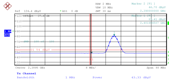
Figure 7.6-23: Radiated band edge at restricted band at 2390 MHz (Average) BLE 1(2M)
