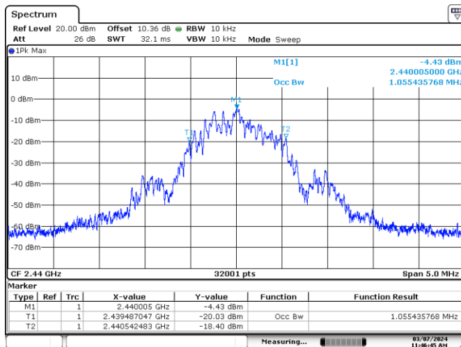
Figure 7.4-17: 99% occupied bandwidth on Mid channel (1M BLE 1)
