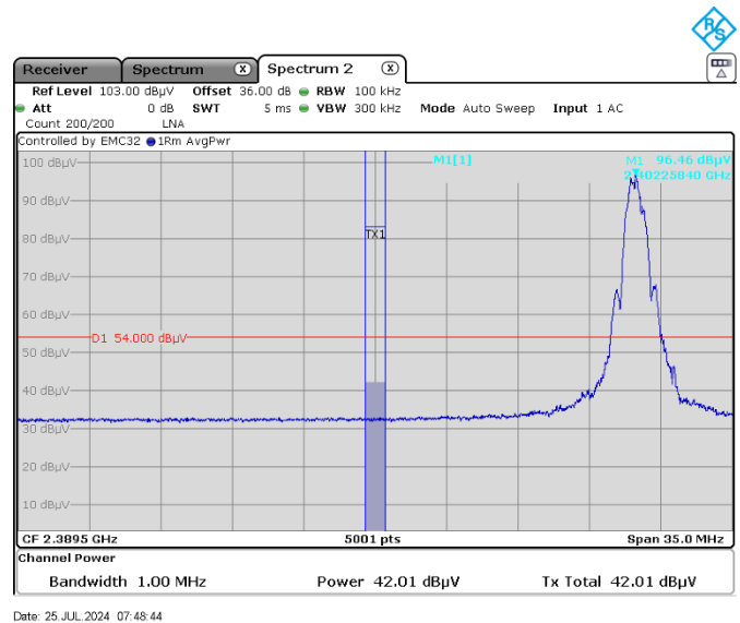
Figure 7.6-14: Radiated band edge at restricted band at 2390 MHz, Average
