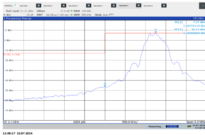
Figure 7.6-8: Conducted band edge at non-restricted band at 2400 MHz
