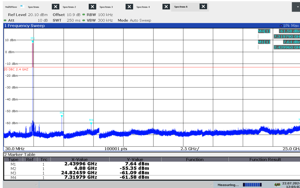
Figure 7.6-11: Conducted spurious emissions mid channel
