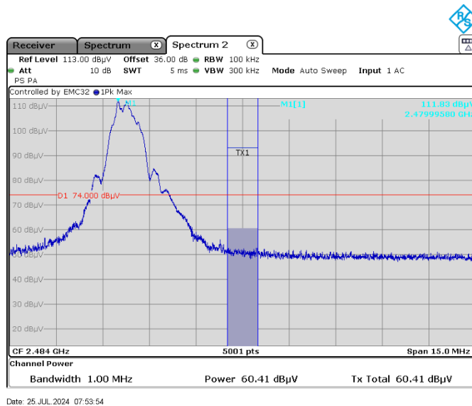
Figure 7.6-15: Radiated band edge at restricted band at 2483.5 MHz, Peak
