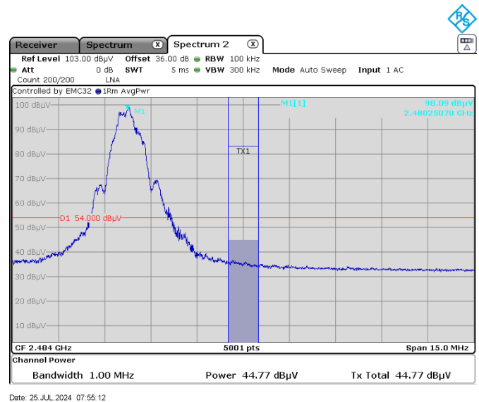
Figure 7.6-16: Radiated band edge at restricted band at 2483.5 MHz, Average
