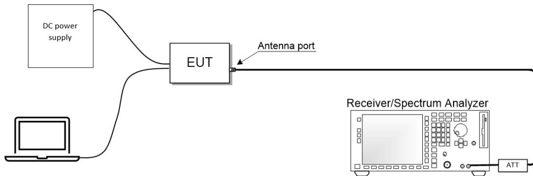
Figure 4.5-2: Antenna port testing block diagram
