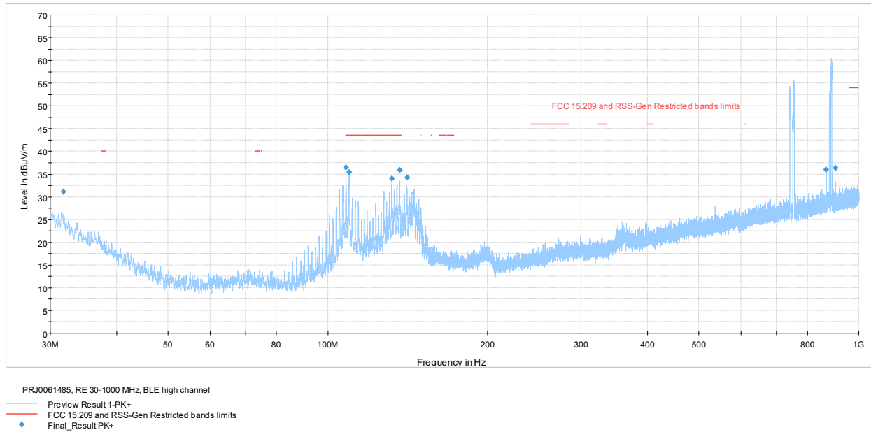
Figure 7.6-3: Radiated spurious emissions 30-1000 MHz high channel
