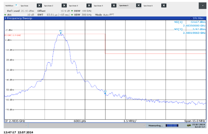
Figure 7.6-9: Conducted band edge at non-restricted band at 2483.5 MHz
