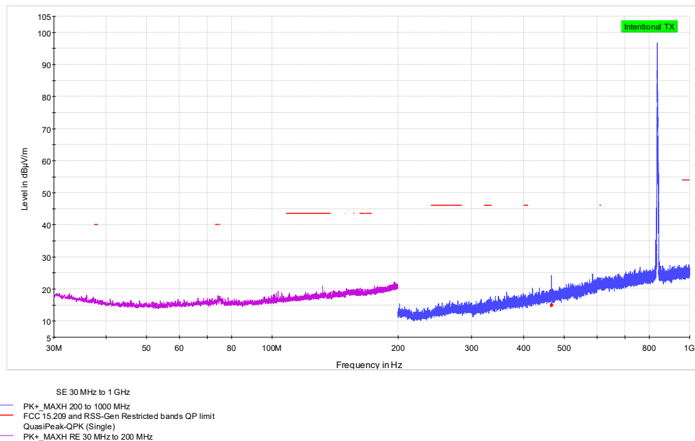
Figure 7.6-19: Radiated spurious emissions 30 – 1000 MHz, LTE Band 5 and BLE mid channel
