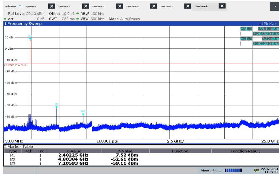
Figure 7.6-10: Conducted spurious emissions low channel
