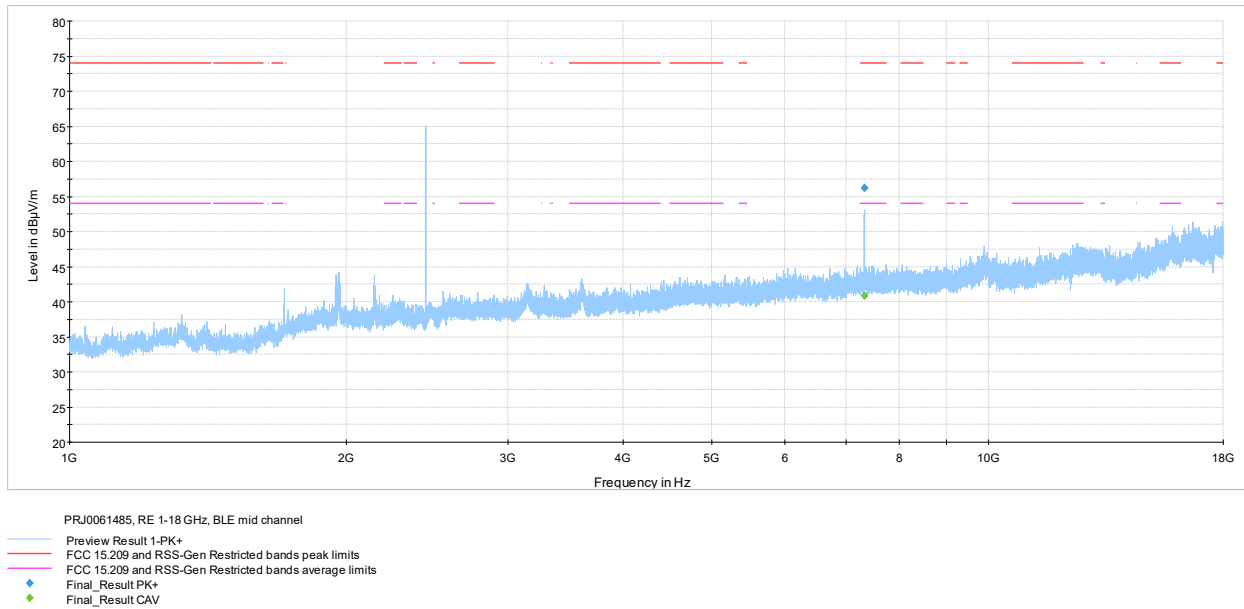
Figure 7.6-5: Radiated spurious emissions 1-18 GHz mid channel
