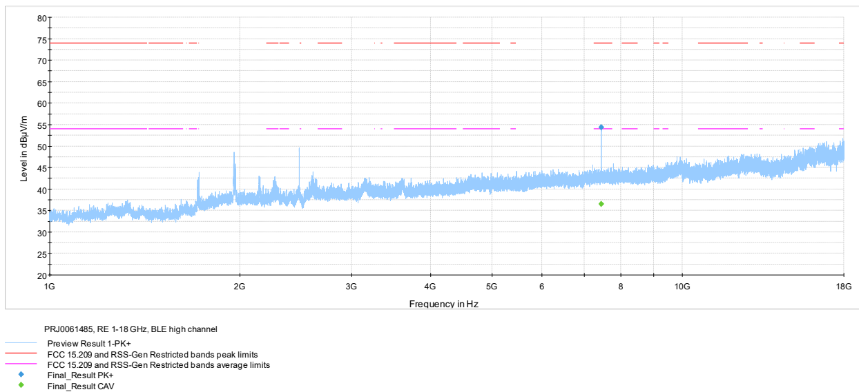
Figure 7.6-6: Radiated spurious emissions 1-18 GHz high channel
