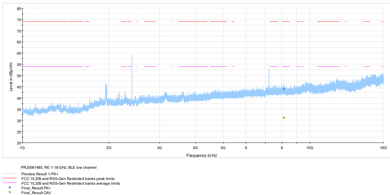
Figure 7.6-4: Radiated spurious emissions 1-18 GHz low channel
