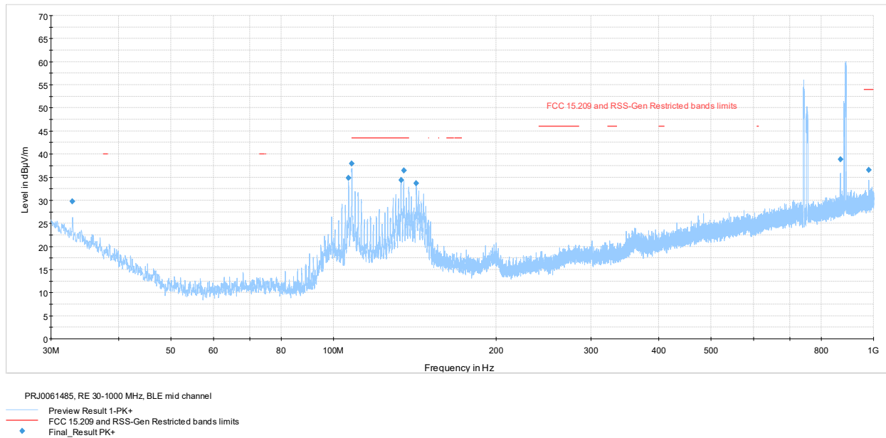
Figure 7.6-2: Radiated spurious emissions 30-1000 MHz mid channel
