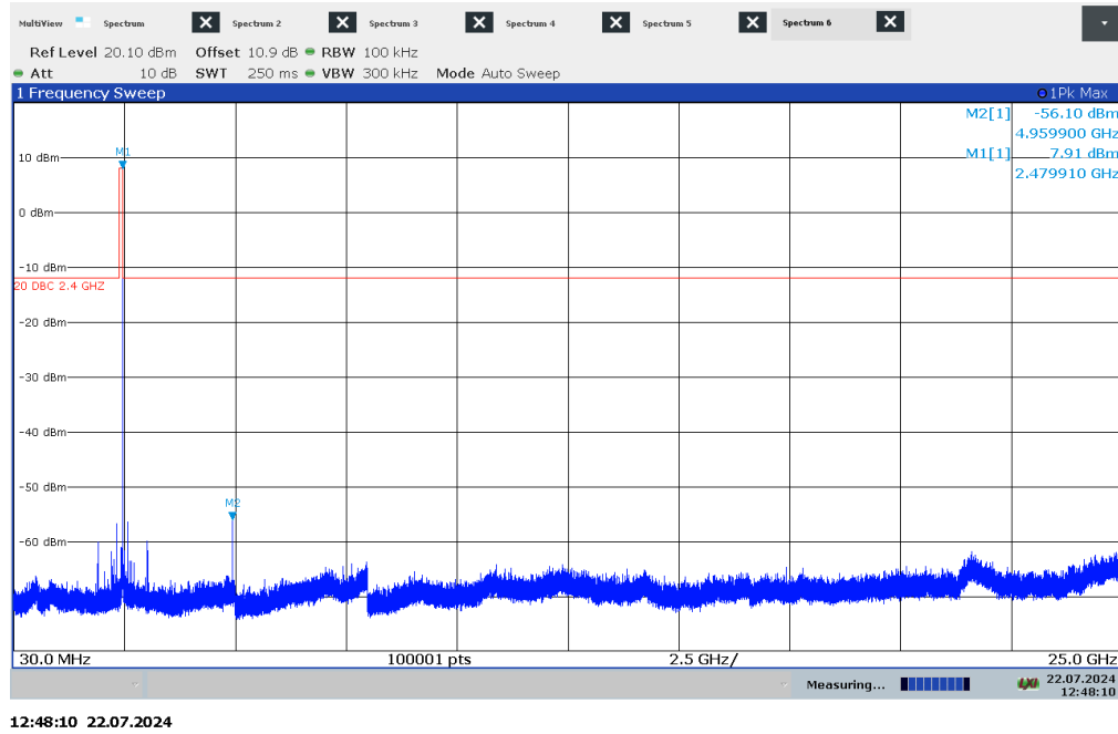
Figure 7.6-12: Conducted spurious emissions high channel
