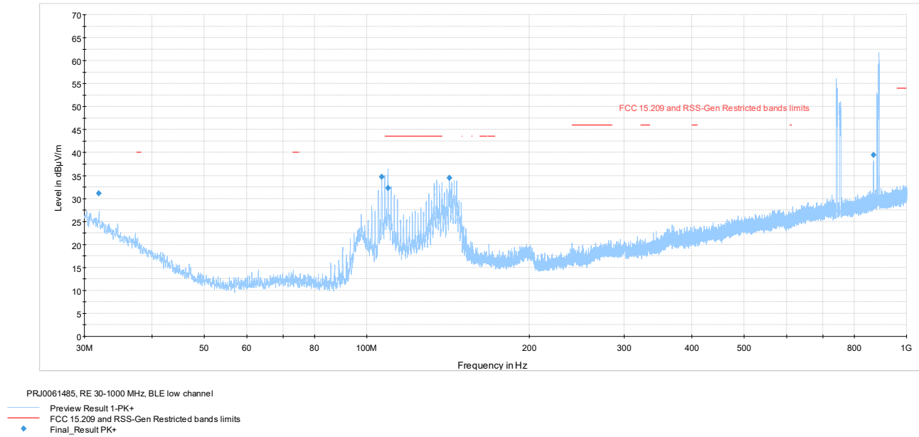
Figure 7.6-1: Radiated spurious emissions 30-1000 MHz low channel
