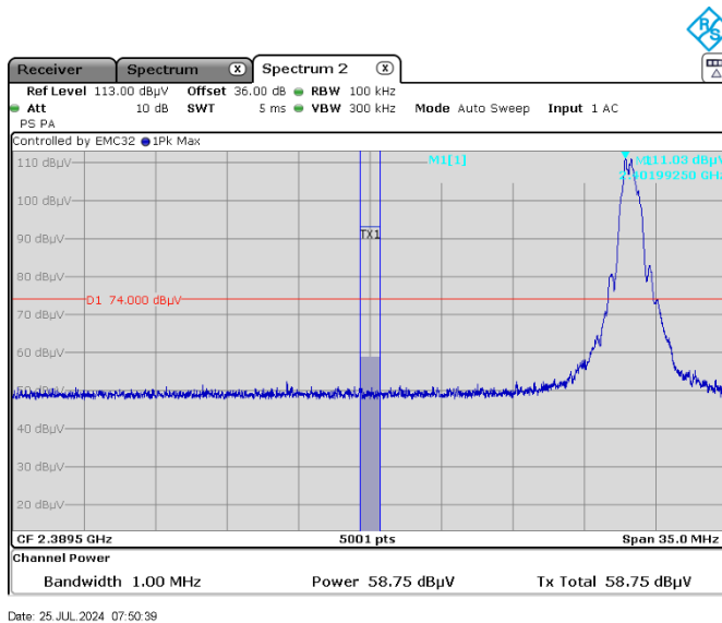
Figure 7.6-13: Radiated band edge at restricted band at 2390 MHz, Peak
