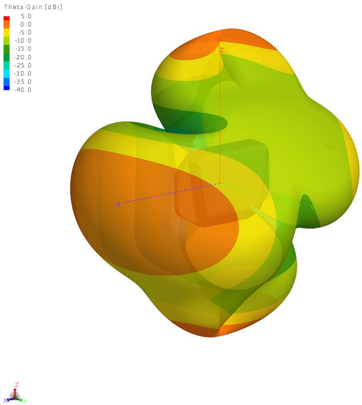
Theta Polarization
