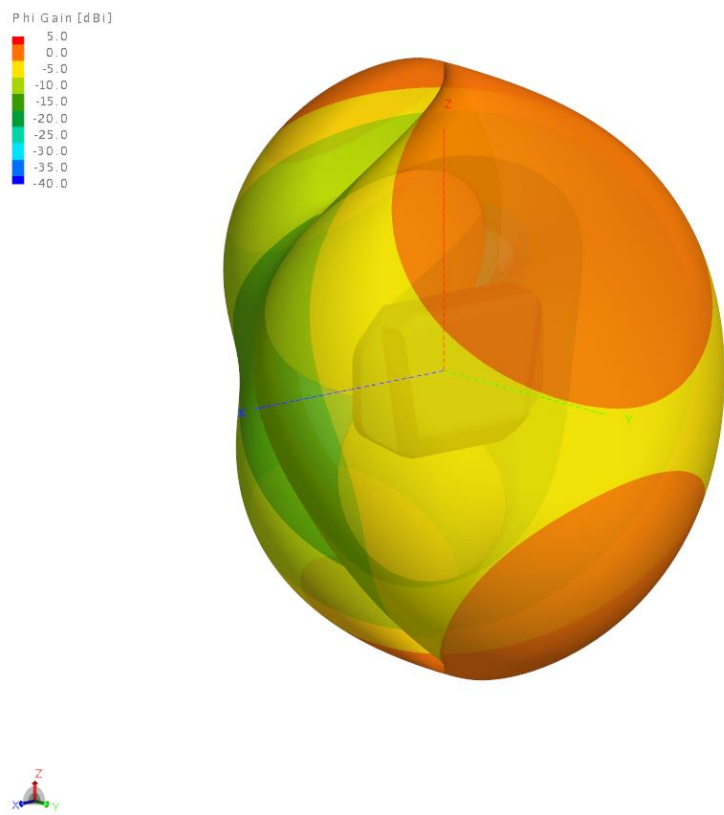
Phi Polarization
