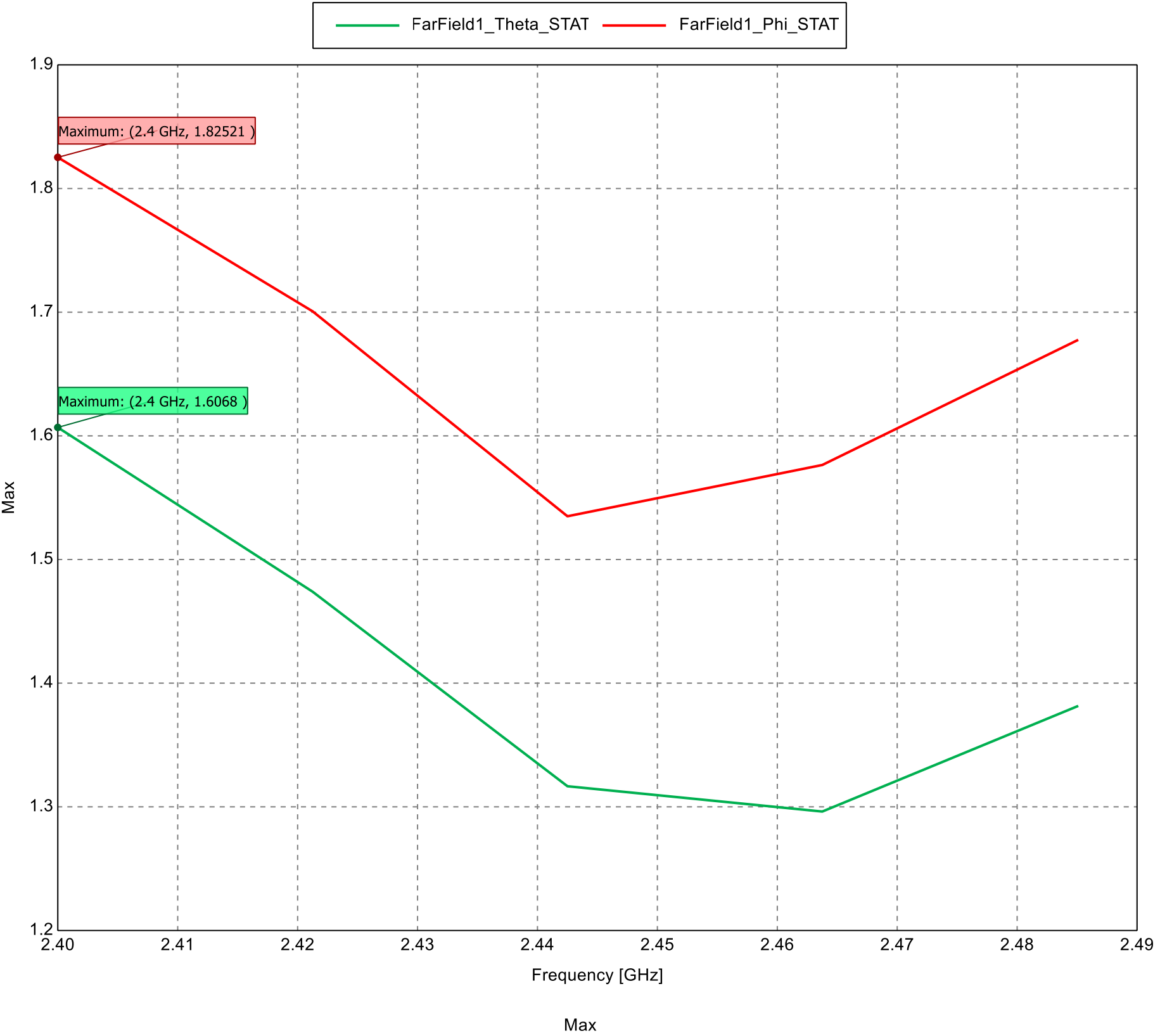
Max Gain (dBi)
