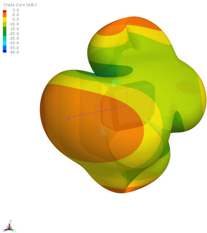
Theta Polarization
