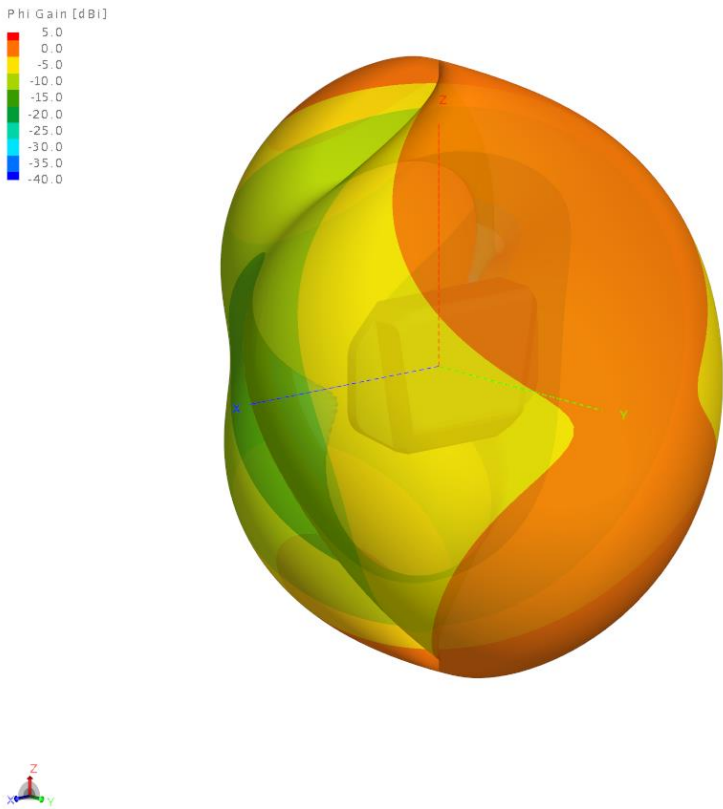
Phi Polarization
