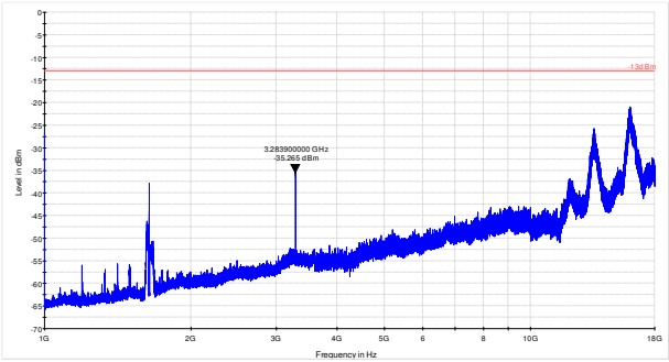
Figure 8.3-4: Spurious emissions above 1 GHz, Patch antenna, mid channel
