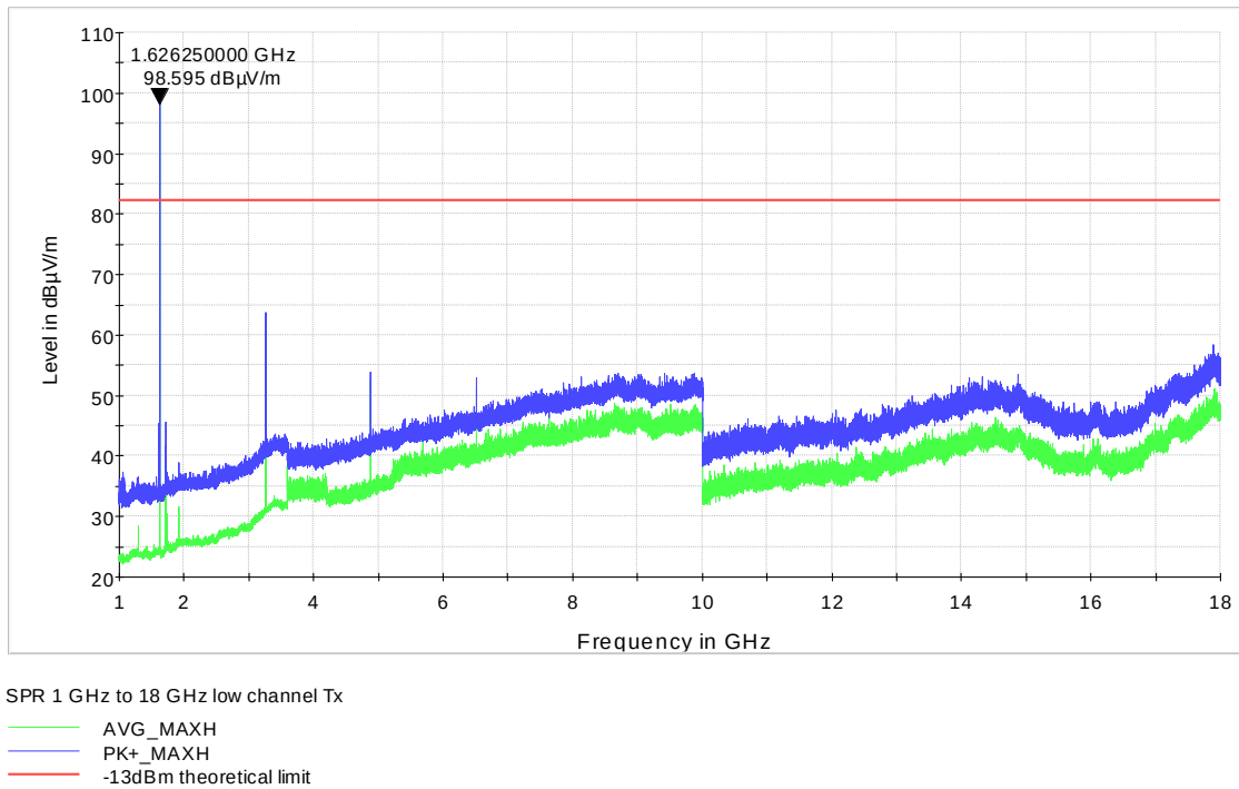
Figure 7.3-20: Radiated spurious emissions 1 – 18 GHz for sub-band 1, low channel waveform Y
