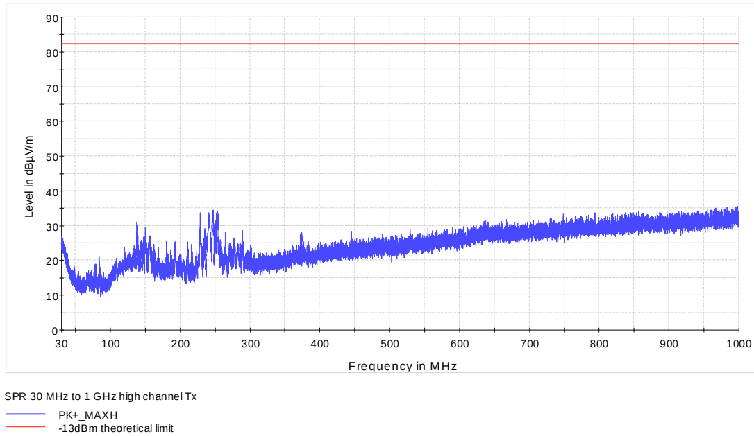
Figure 7.3-17: Radiated spurious emissions below 1 GHz for sub-band 1, high channel waveform T
