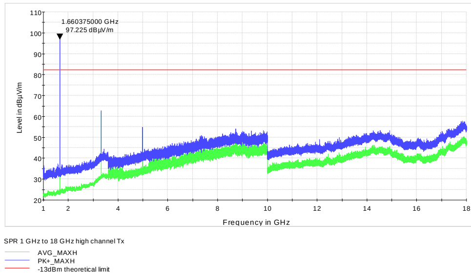
Figure 7.3-12: Radiated spurious emissions 1 – 18 GHz for sub-band 1, high channel waveform K
