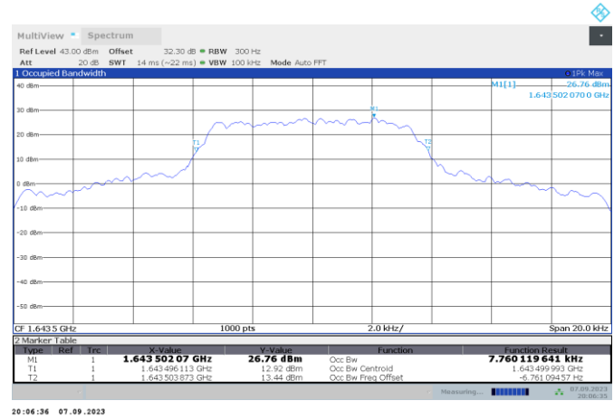
Figure 7.1-20: 99 % bandwidth on mid channel for waveform Y
