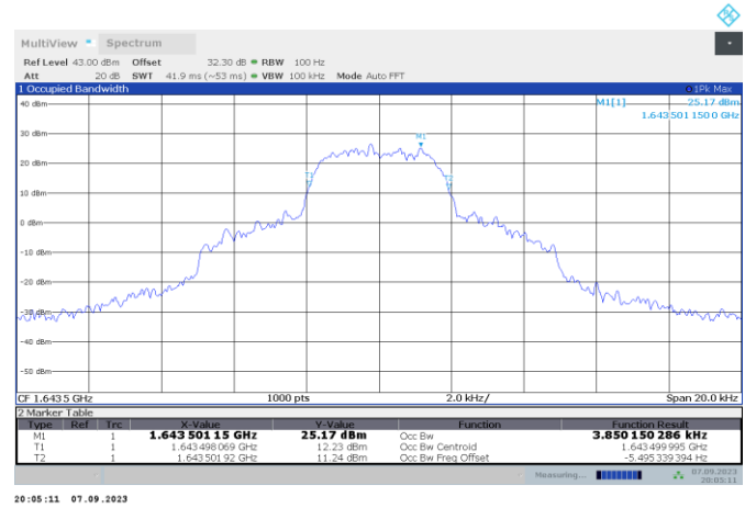
Figure 7.1-14: 99 % bandwidth on mid channel for waveform T
