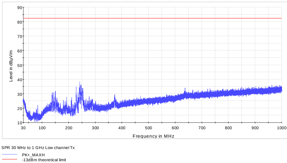
Figure 7.3-1: Radiated spurious emissions below 1 GHz for sub-band 1, low channel for waveform J
