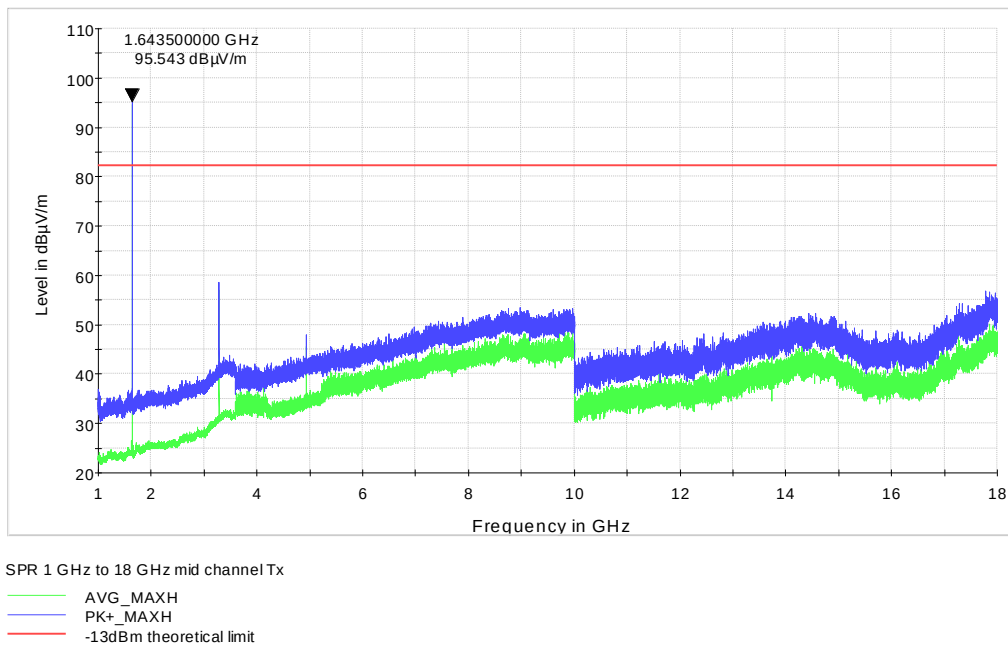
Figure 7.3-4: Radiated spurious emissions 1 – 18 GHz for sub-band 1, mid channel waveform J
