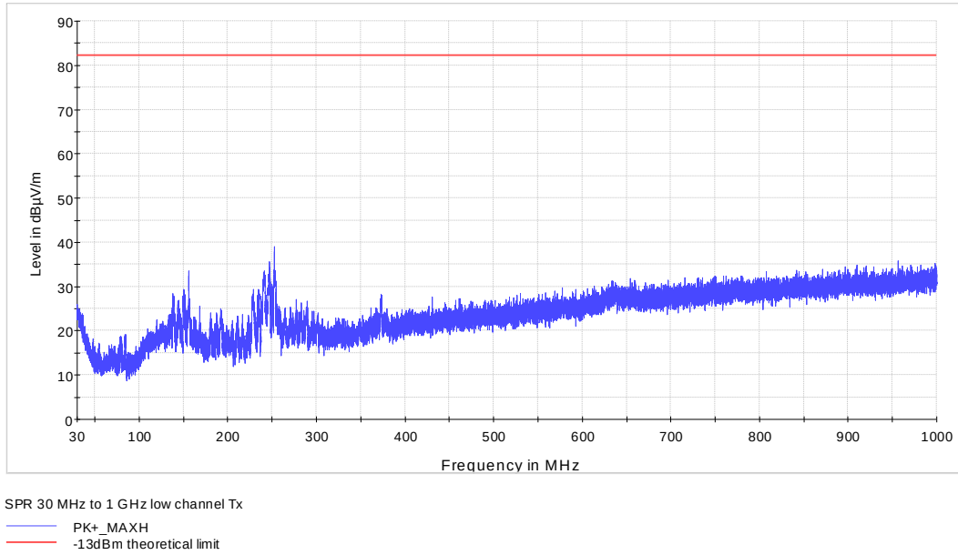
Figure 7.3-19: Radiated spurious emissions below 1 GHz for sub-band 1, low channel waveform Y
