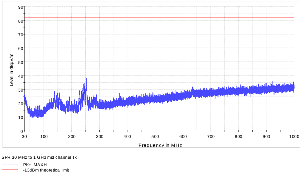
Figure 7.3-3: Radiated spurious emissions below 1 GHz for sub-band 1, mid channel waveform J
