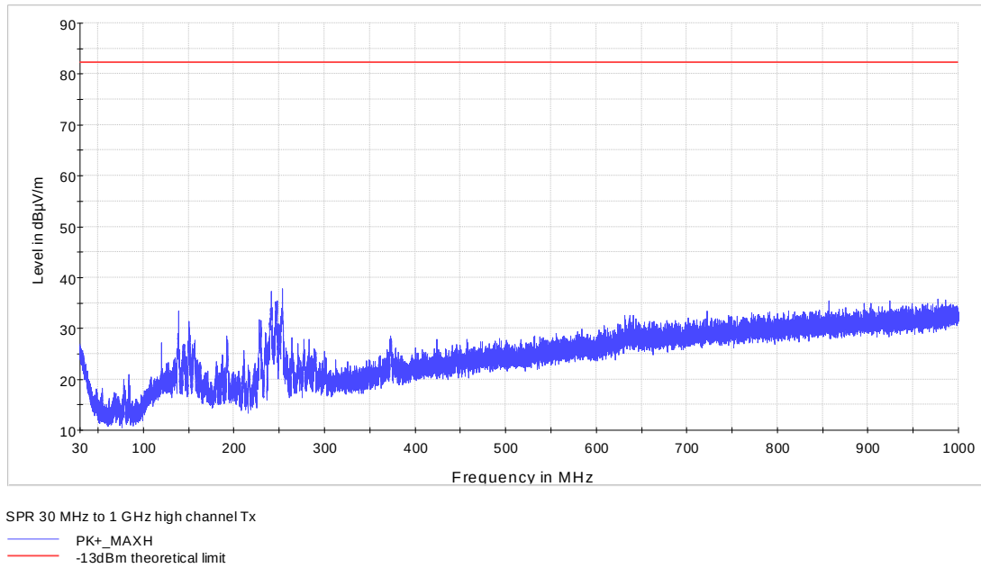
Figure 7.3-11: Radiated spurious emissions below 1 GHz for sub-band 1, high channel waveform K
