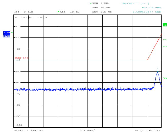
Figure 8.5-4: Emissions within 1559–1610 MHz, low channel, ISD limits
