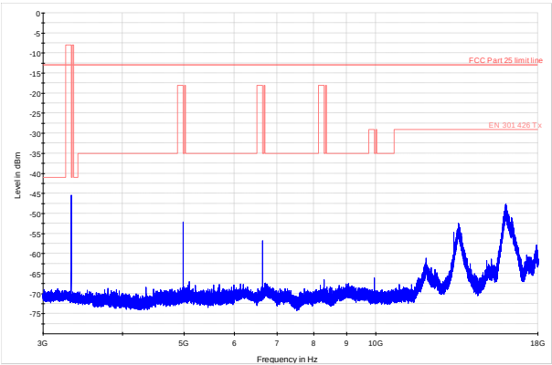
Figure 8.3-9: Spurious emissions above 3 GHz, high channel
