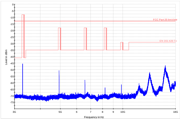
Figure 8.3-8: Spurious emissions above 3 GHz, mid channel
