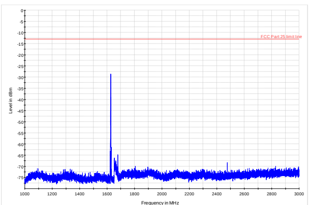
Figure 8.3-4: Spurious emissions within 1–3 GHz, low channel
