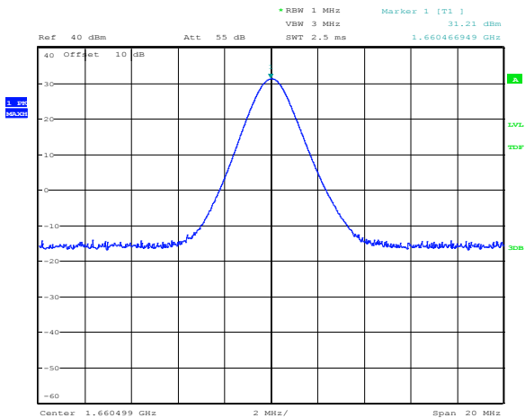
Figure 8.2-1: POP on low channel
