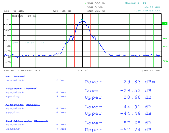
Figure 8.3-11: Emissions Mask, mid channel
