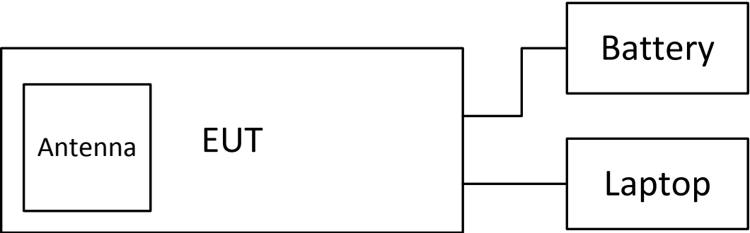
Figure 3.6-1: Setup diagram
