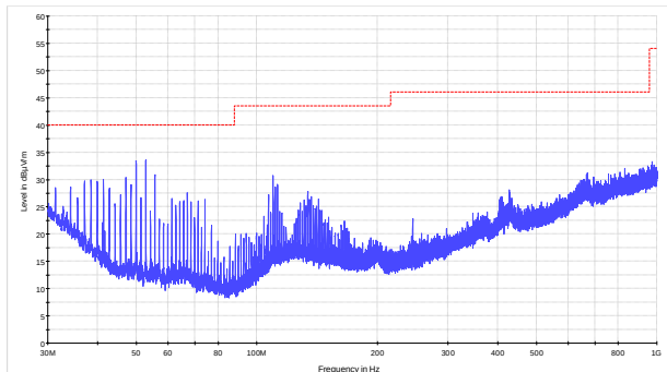
Figure 8.3-1: Spurious emissions below 1 GHz, low channel
