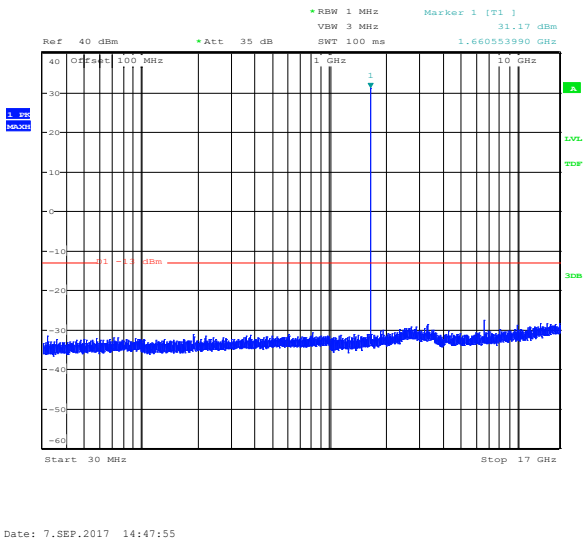
Figure 8.3-16: Conducted spurious emissions, high channel
