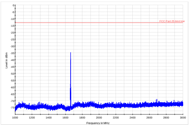
Figure 8.3-6: Spurious emissions within 1–3 GHz, high channel
