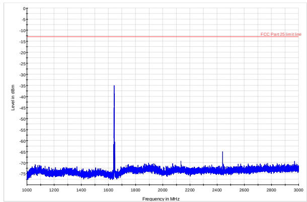
Figure 8.3-5: Spurious emissions within 1–3 GHz, mid channel
