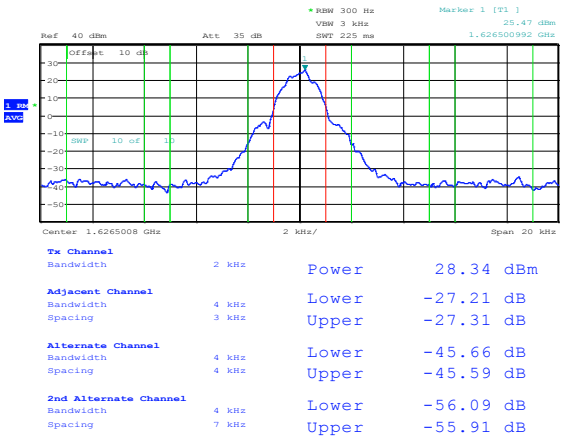
Figure 8.3-10: Emissions Mask, low channel
