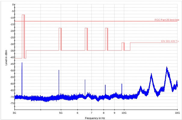
Figure 8.3-7: Spurious emissions above 3 GHz, low channel
