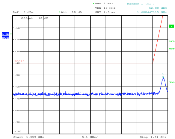
Figure 8.5-1: Emissions within 1559–1610 MHz, low channel, FCC limits
