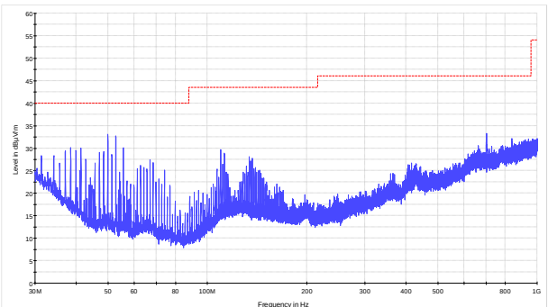
Figure 8.3-2: Spurious emissions below 1 GHz, mid channel
