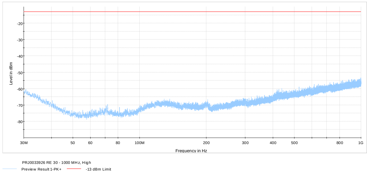
Figure 7.3-4: Radiated Spurious emissions 30 – 1000 MHz, high channel
