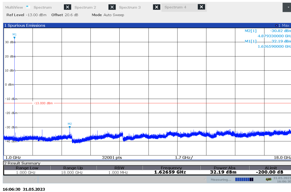
Figure 7.3-9: Conducted spurious emissions 1 – 18 GHz (worst case)
