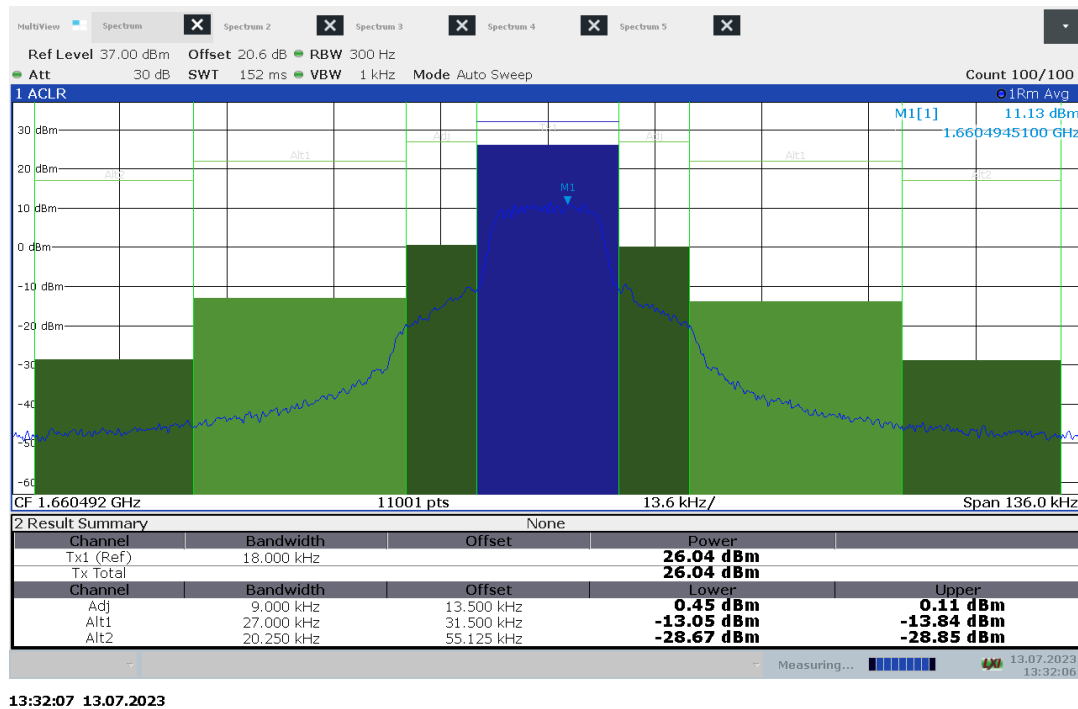
Figure 7.3-4: Conducted band edge spurious emissions outside assigned bandwidth – Waveform Z, high channel
