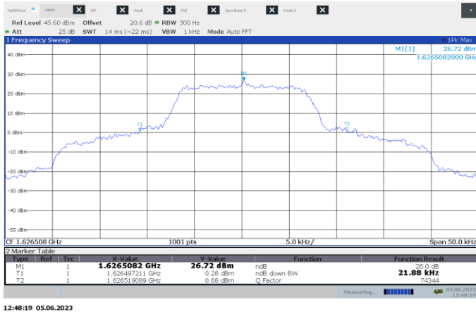
Figure 7.1-28: 26 dB bandwidth on low channel – Waveform Z
