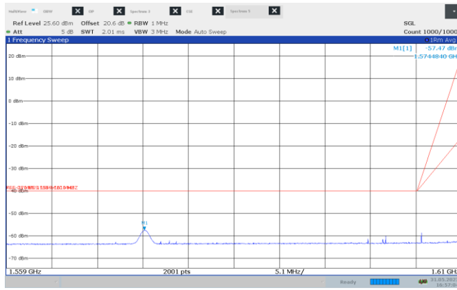
Figure 7.4-1: spurious emissions 1559–1610 MHz, Waveform R, low channel
