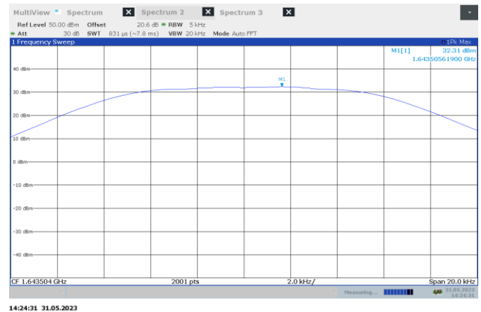
Figure 7.2-11: Conducted peak output power on mid channel – Waveform Y
