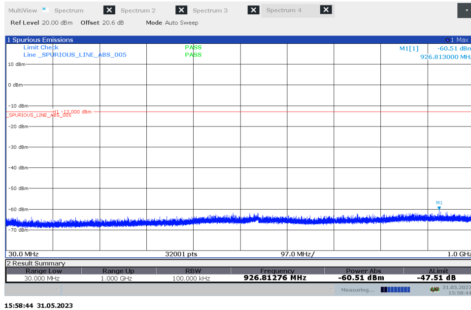
Figure 7.3-9: Conducted spurious emissions 30 – 1000 MHz (worst case)
