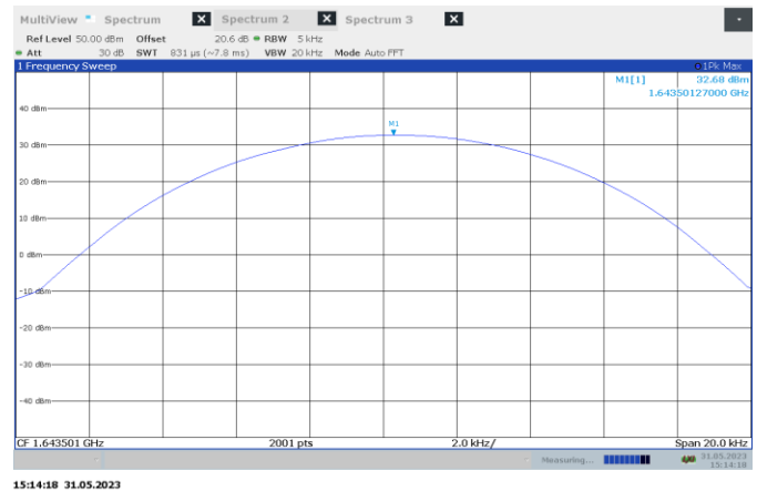
Figure 7.2-5: Conducted peak output power on mid channel – Waveform S
