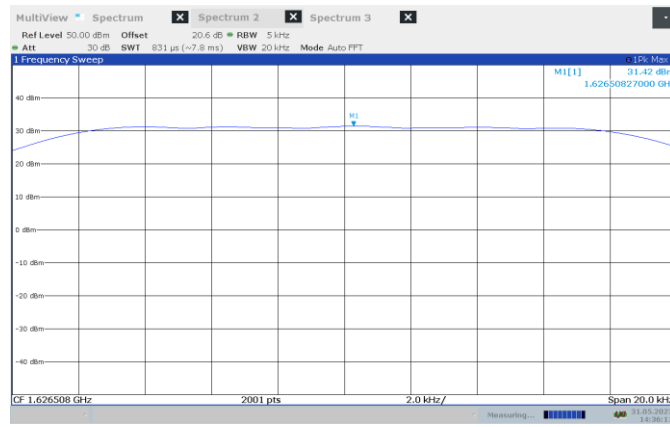
Figure 7.2-13: Conducted peak output power on low channel – Waveform Z
