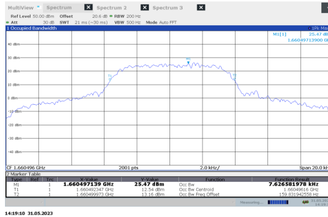
Figure 7.1-21: 99 % bandwidth on high channel – Waveform Y
