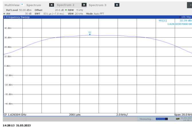
Figure 7.2-10: Conducted peak output power on low channel – Waveform Y
