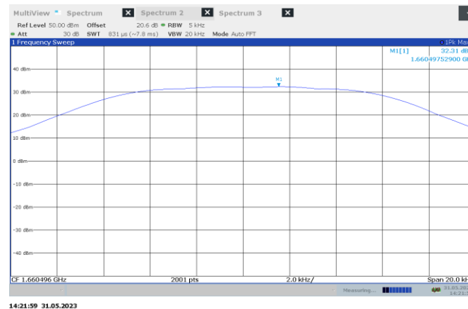
Figure 7.2-12: Conducted peak output power on high channel – Waveform Y
