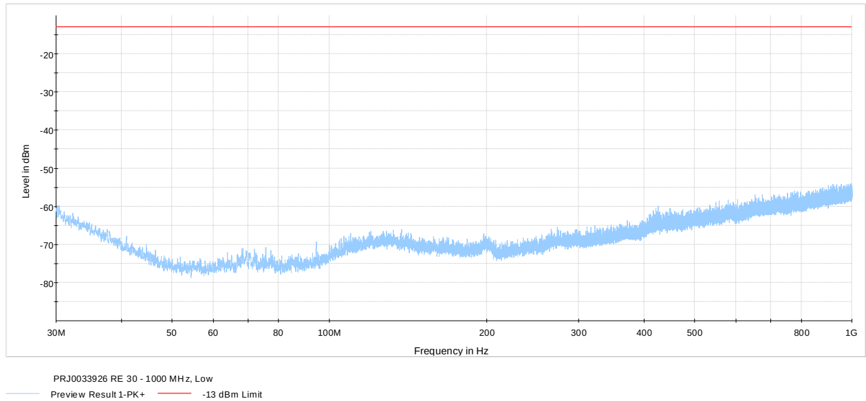
Figure 7.3-3: Radiated Spurious emissions 30 – 1000 MHz, low channel
