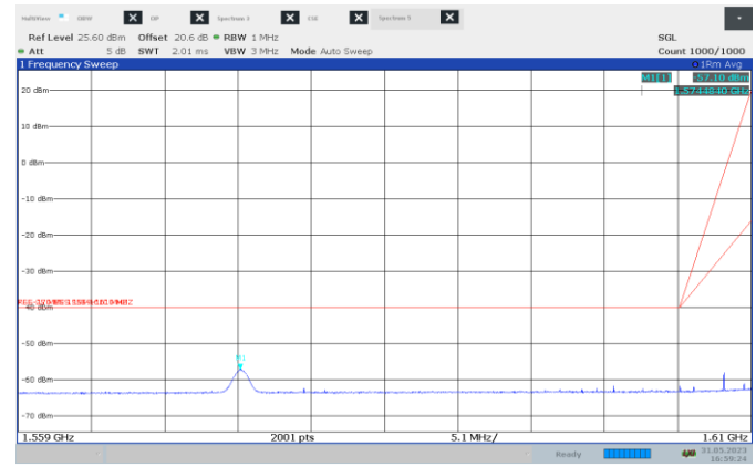
Figure 7.4-2: spurious emissions 1559–1610 MHz, Waveform S, low channel
