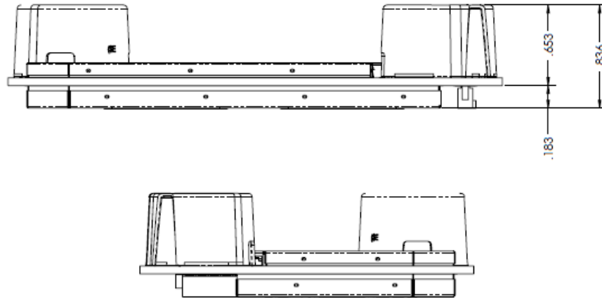
Figure 7: Side View Dimensions (in.)
