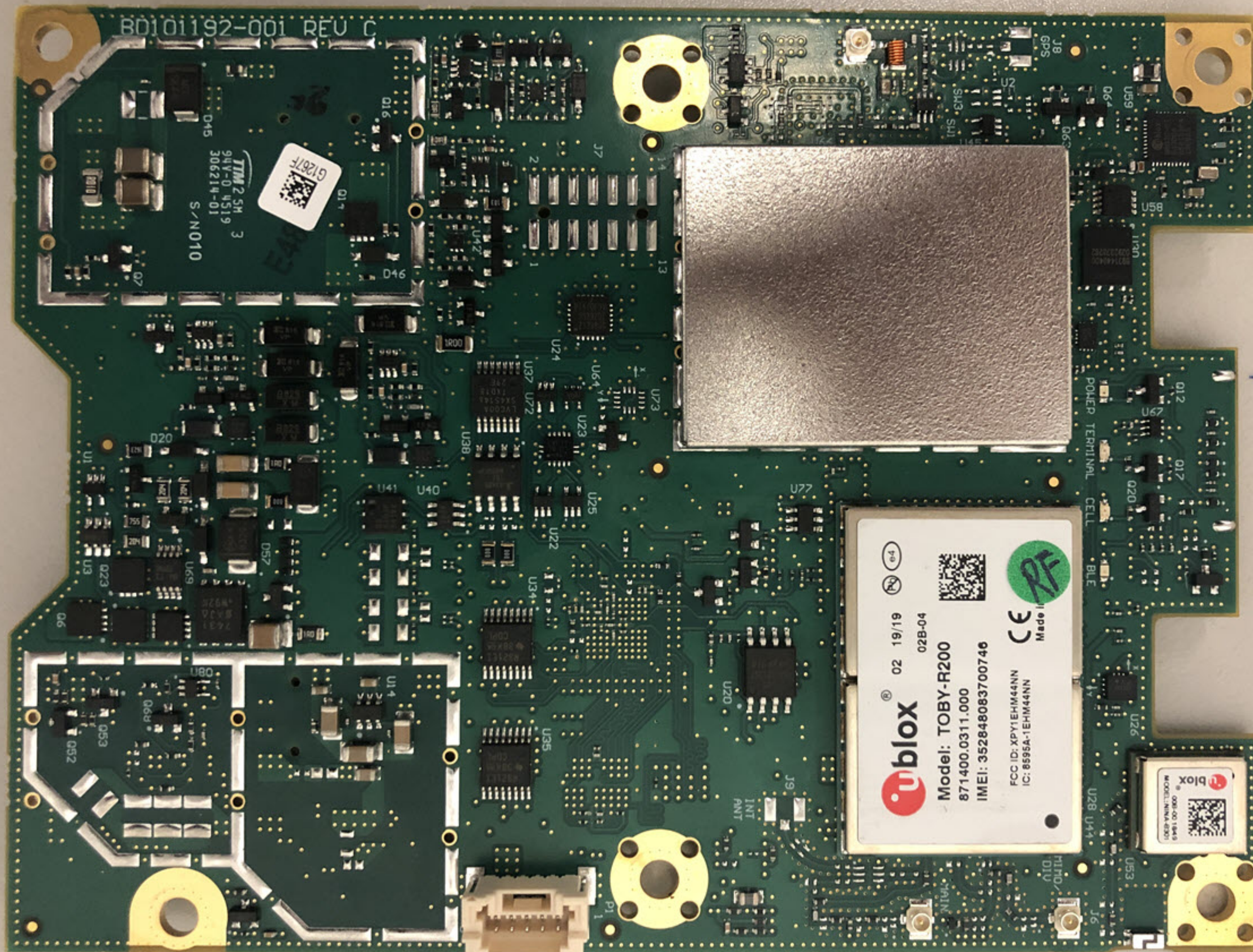
PCB top with shield
