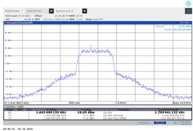
Figure 7.1-8: 99 % bandwidth on mid channel for waveform K
