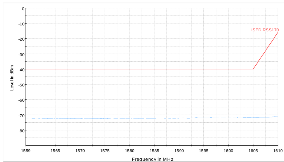
Figure 8.5-3: Radiated spurious emissions 1559–1610 MHz, low channel, ISED limit
