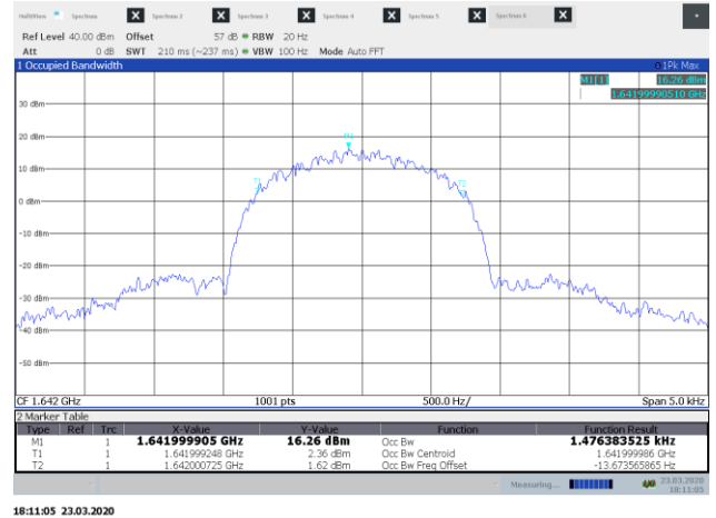
Figure 8.1-2: 99 % bandwidth on mid channel
