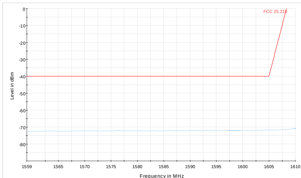
Figure 8.5-1: Radiated spurious emissions 1559–1610 MHz, low channel, FCC limit
