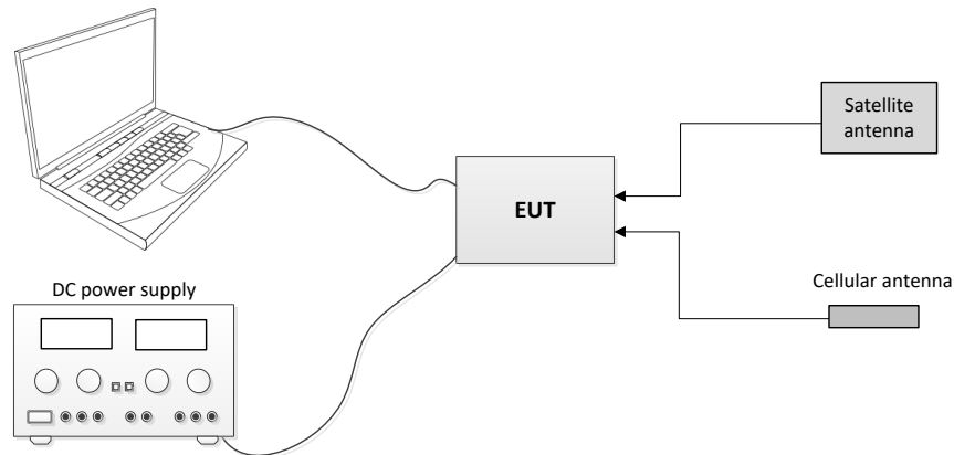
Figure 3.6-1: Setup diagram
