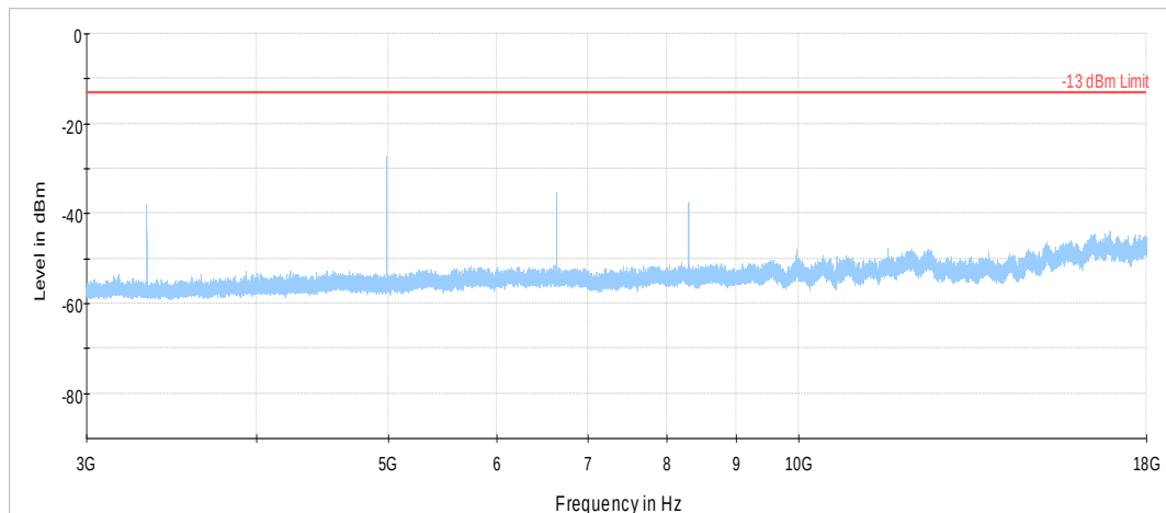
Figure 8.3-6: Radiated spurious emissions 3 – 18 GHz, low channel
