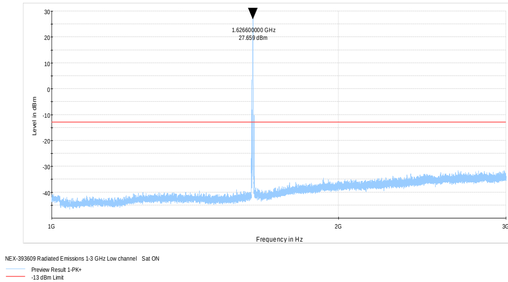
Figure 8.3-4: Radiated spurious emissions 1–3 GHz, low channel
