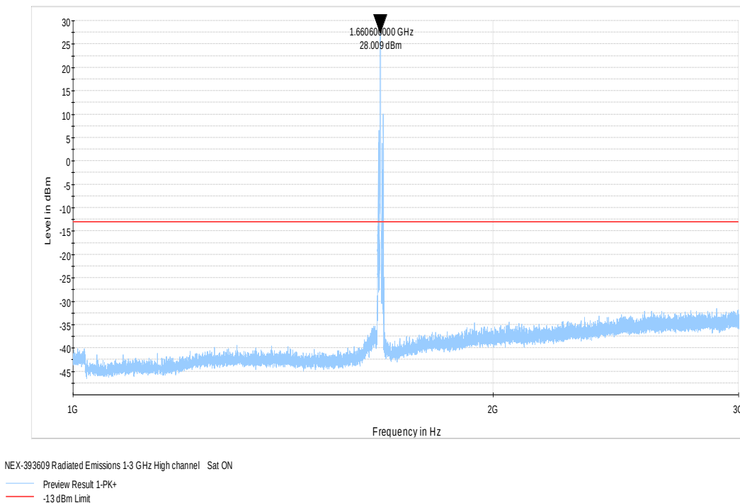
Figure 8.3-5: Radiated spurious emissions 1–3 GHz, high channel
