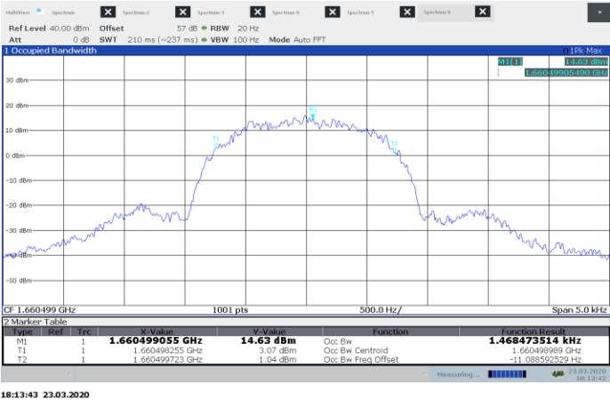
Figure 8.1-3: 99 % bandwidth on high channel
