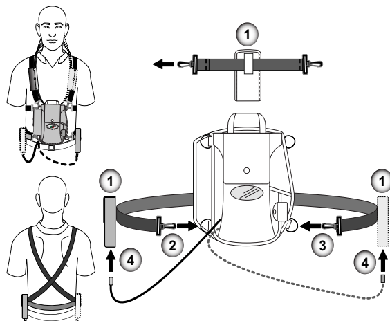
Figure 2: Optional second battery.
