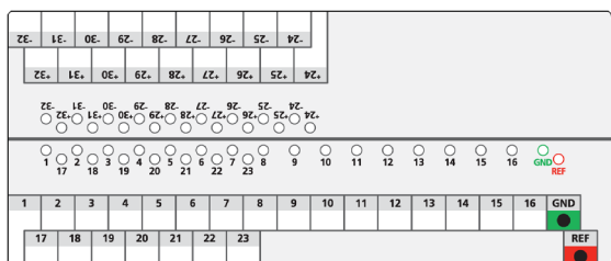
Figure 1: 32 channel electrode label.
