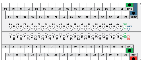
Figure 2: 64 channel electrode label.
