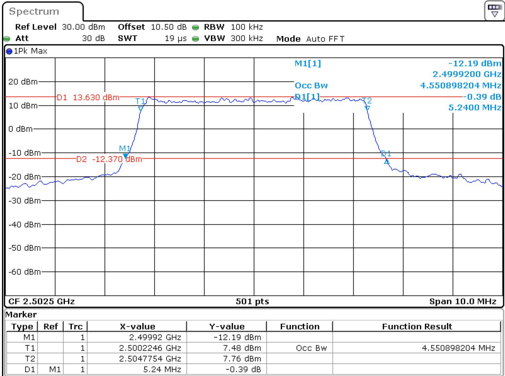
Band 7_5 MHz_Low_16QAM_RB25#0
