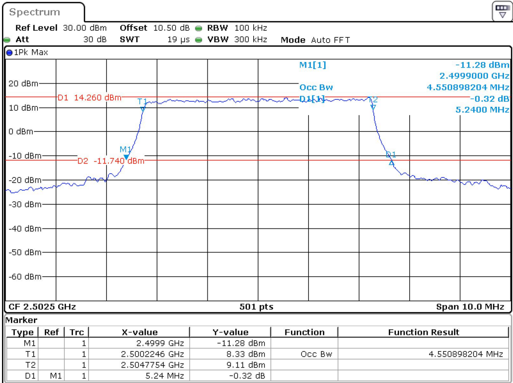
Band 7_5 MHz_Low_QPSK_RB25#0
