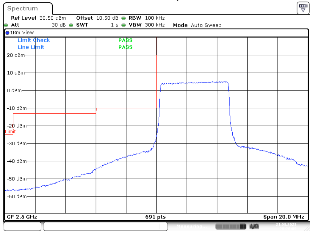
Band 7_5 MHz_Low_16QAM_RB25#0
