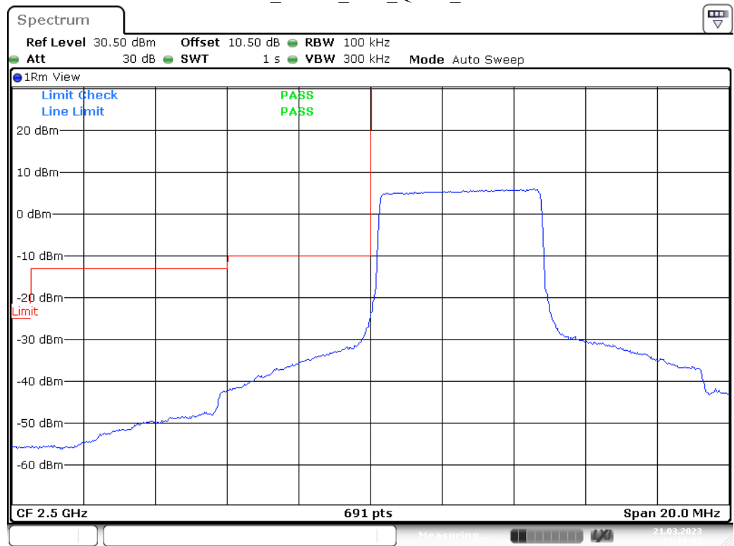
Band 7_5 MHz_Low_QPSK_RB25#0
