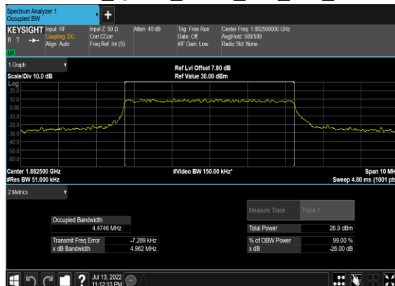
N25(5M)_DFT-s- OFDM_QPSK_Outer_Full_Mid_CH
