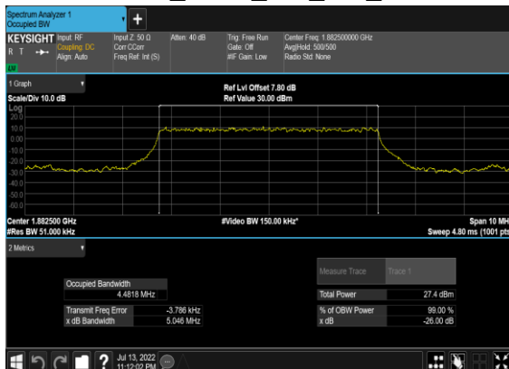
N25(5M)_DFT-s-OFDM_PI_2- BPSK_Outer_Full_Mid_CH
