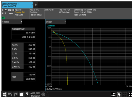
N71(20M)_DFT-s-OFDM_QPSK_Outer_Full_High_CH
