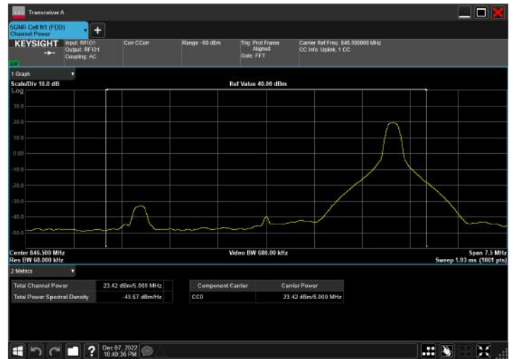
n5_5MHz_15kHz_846.5MHz_CP-OFDM 16 QAM_RB25@0
