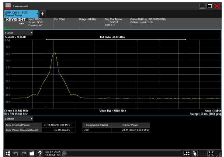
n5_10MHz_15kHz_836.5MHz_CP-OFDM QPSK_RB1@1
