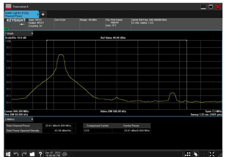
n5_5MHz_15kHz_846.5MHz_CP-OFDM QPSK_RB1@1
