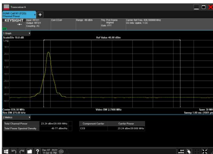
n5_20MHz_15kHz_836.5MHz_DFT-s-OFDM QPSK_RB1@1
