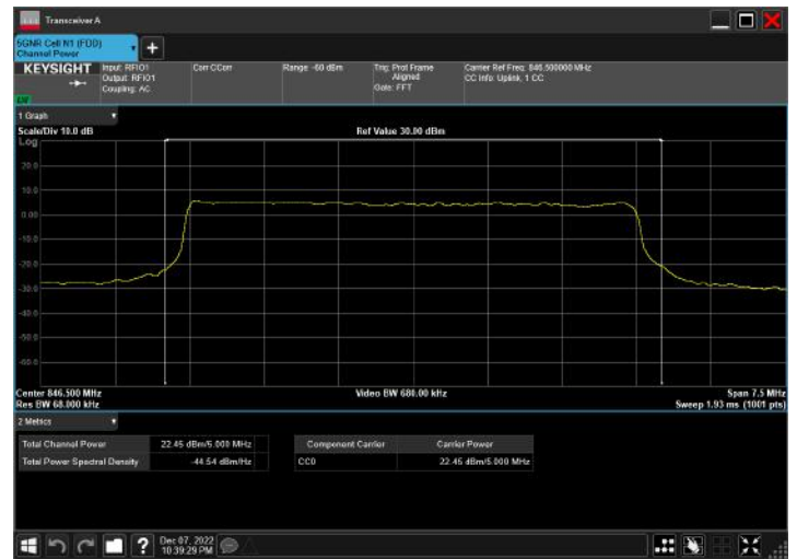
n5_5MHz_15kHz_846.5MHz_DFT-s-OFDM 64 QAM_RB25@0
