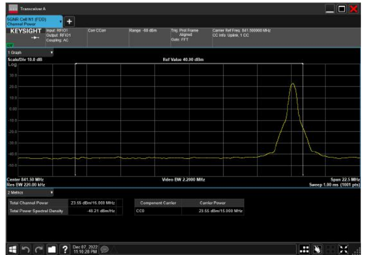
n5_15MHz_15kHz_841.5MHz_CP-OFDM 16 QAM_RB79@0
