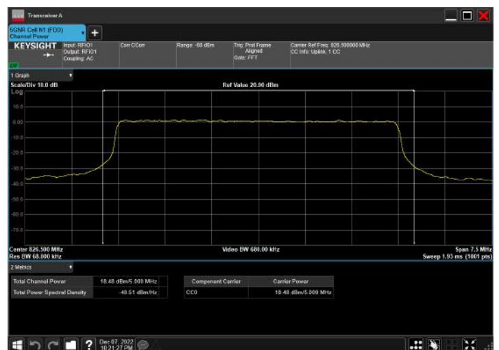
n5_5MHz_15kHz_826.5MHz_CP-OFDM 256 QAM_RB25@0
