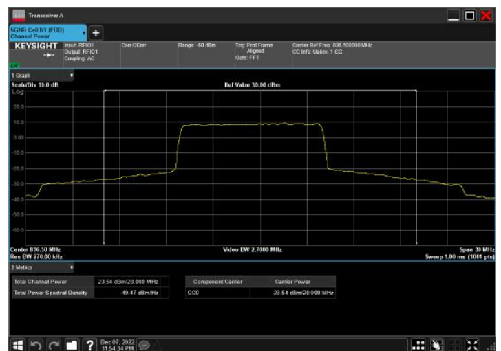
n5_20MHz_15kHz_836.5MHz_DFT-s-OFDM QPSK_RB50@25
