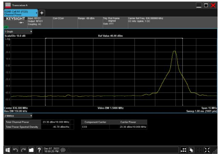
n5_10MHz_15kHz_836.5MHz_CP-OFDM 16 QAM_RB52@0
