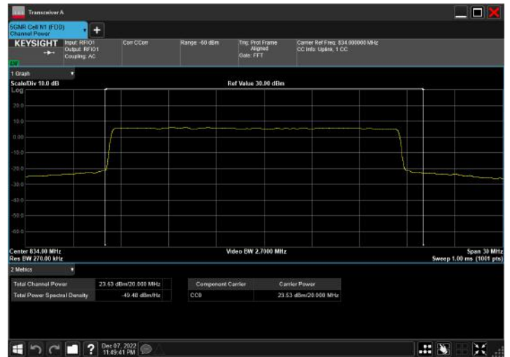
n5_20MHz_15kHz_834MHz_DFT-s-OFDM 64 QAM_RB100@0
