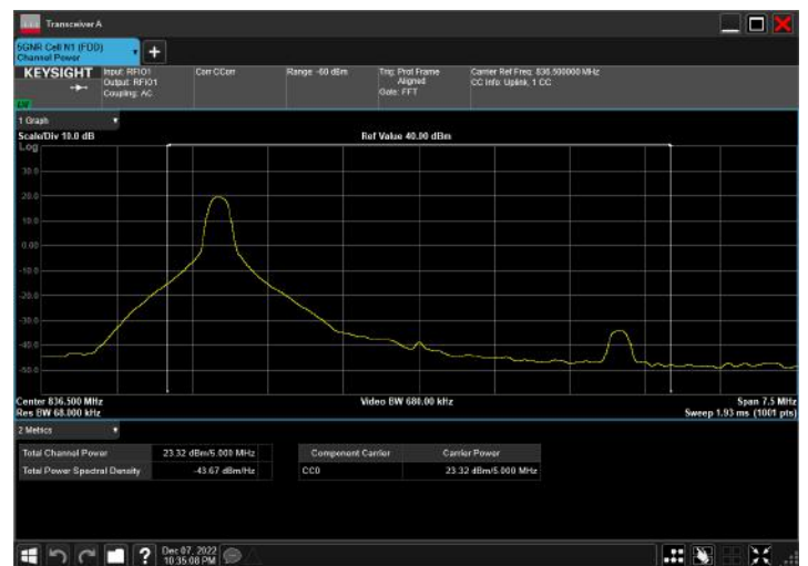
n5_5MHz_15kHz_836.5MHz_CP-OFDM QPSK_RB1@1
