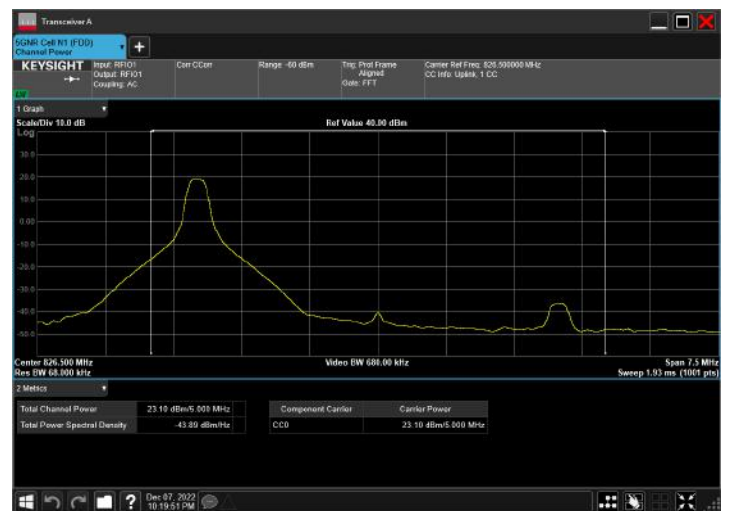
n5_5MHz_15kHz_826.5MHz_CP-OFDM QPSK_RB1@1
