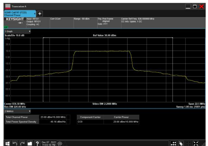
n5_15MHz_15kHz_836.5MHz_DFT-s-OFDM QPSK_RB36@18
