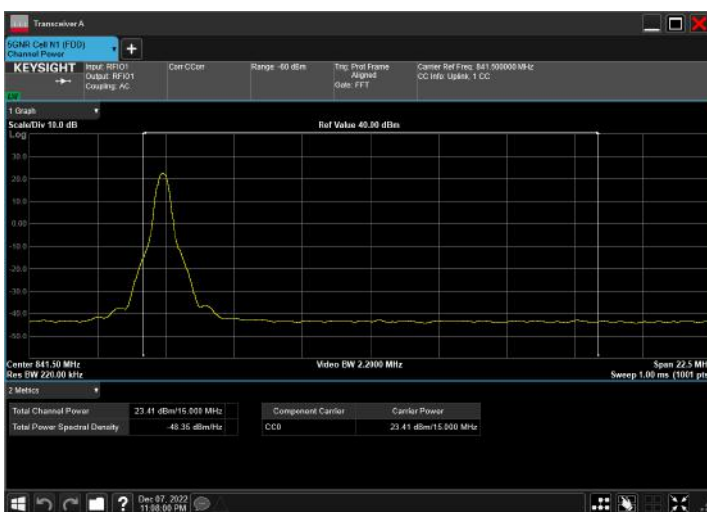
n5_15MHz_15kHz_841.5MHz_DFT-s-OFDM QPSK_RB1@1
