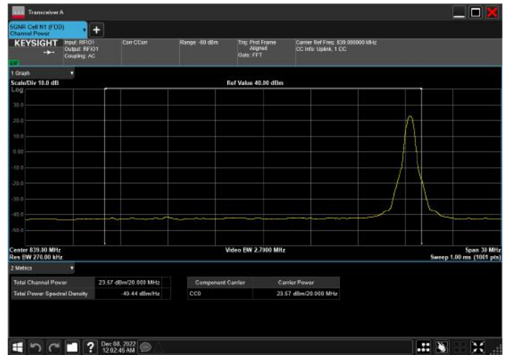
n5_20MHz_15kHz_839MHz_CP-OFDM 16 QAM_RB106@0
