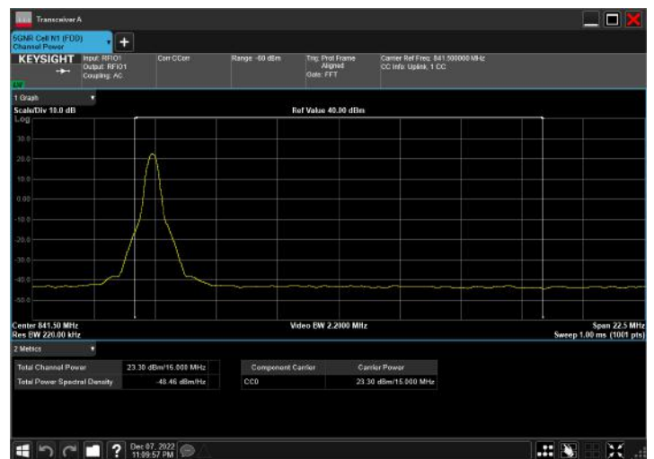
n5_15MHz_15kHz_841.5MHz_CP-OFDM QPSK_RB1@1
