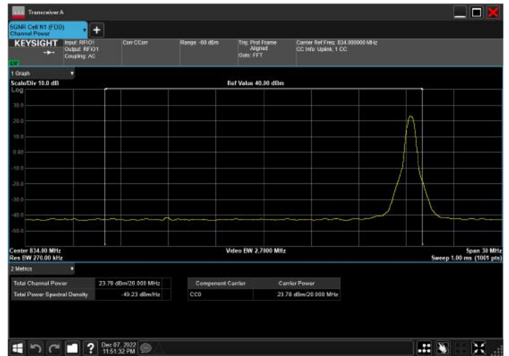
n5_20MHz_15kHz_834MHz_CP-OFDM 16 QAM_RB106@0
