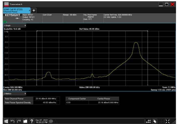
n5_5MHz_15kHz_826.5MHz_CP-OFDM 16 QAM_RB25@0
