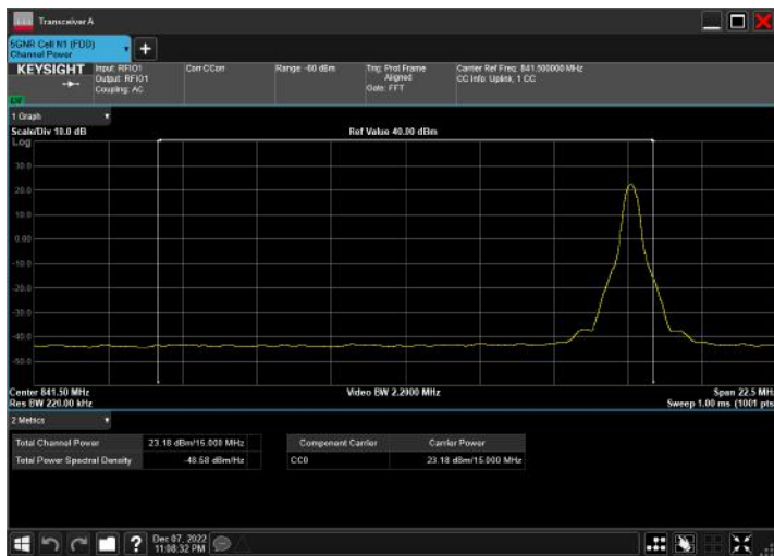
n5_15MHz_15kHz_841.5MHz_DFT-s-OFDM 16 QAM_RB75@0
