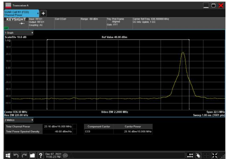
n5_15MHz_15kHz_836.5MHz_CP-OFDM 16 QAM_RB79@0
