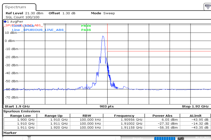
DC_5A_n2A_10MHz|10MHz_15kHz_836.5MHz|1905MHz_DF T-s-OFDM QPSK_RB0|RB1@51
