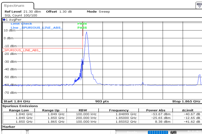
DC_66A_n2A_10MHz|15MHz_15kHz_1745MHz|1857.5MHz_ DFT-s-OFDM QPSK_RB0|RB1@0
