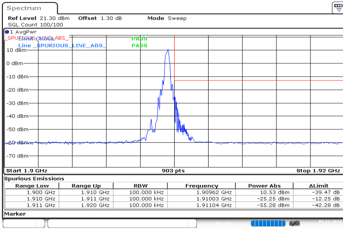
DC_66A_n2A_10MHz|10MHz_15kHz_1745MHz|1905MHz_D FT-s-OFDM QPSK_RB0|RB1@51
