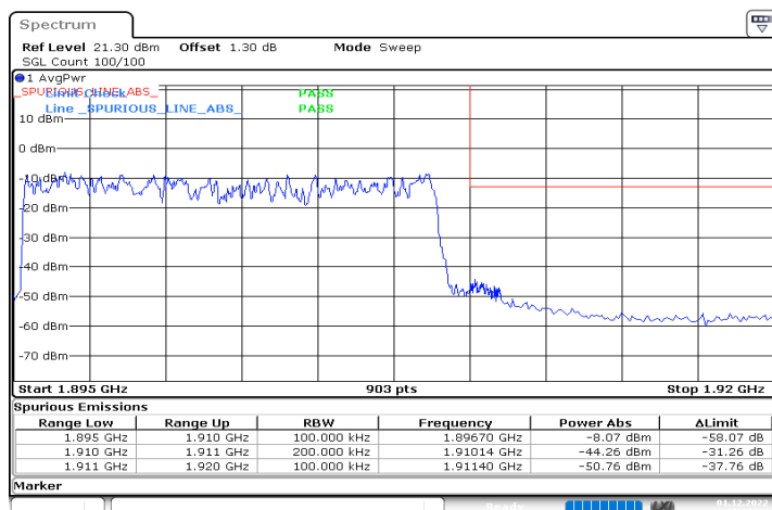
DC_5A_n2A_10MHz|15MHz_15kHz_836.5MHz|1902.5MHz_ DFT-s-OFDM QPSK_RB0|RB75@0
