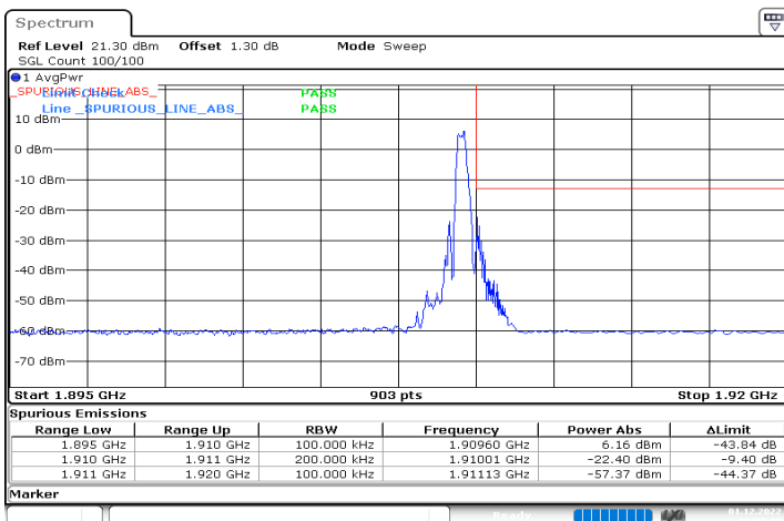
DC_66A_n2A_10MHz|15MHz_15kHz_1745MHz|1902.5MHz_ DFT-s-OFDM QPSK_RB0|RB1@78
