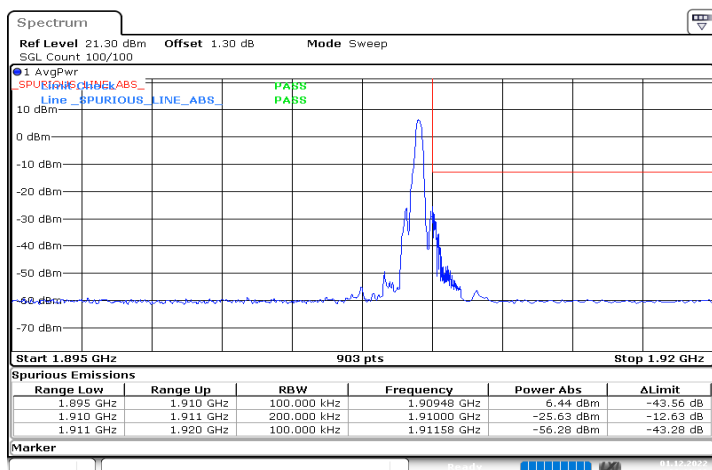
DC_5A_n2A_10MHz|15MHz_15kHz_836.5MHz|1902.5MHz_ DFT-s-OFDM QPSK_RB0|RB1@78
