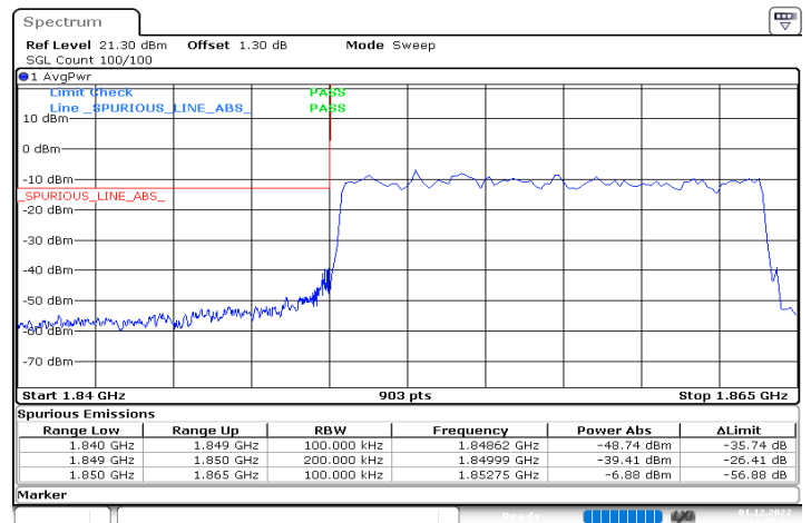
DC_66A_n2A_10MHz|15MHz_15kHz_1745MHz|1857.5MHz_ DFT-s-OFDM QPSK_RB0|RB75@0
