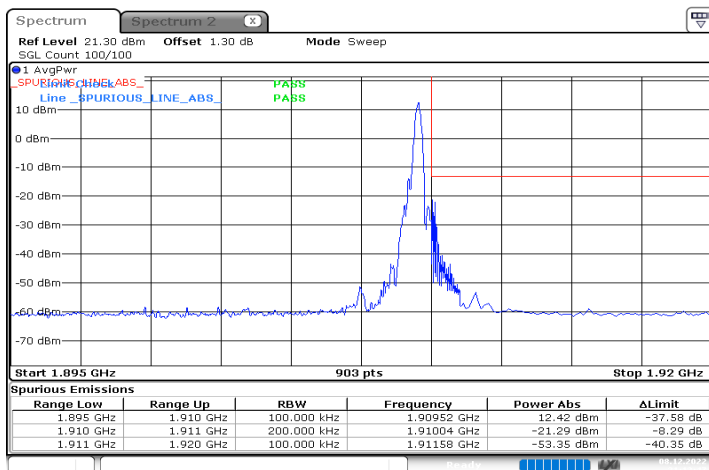
n2_15MHz_15kHz_1902.5MHz_DFT-s-OFDM QPSK_RB1@78
