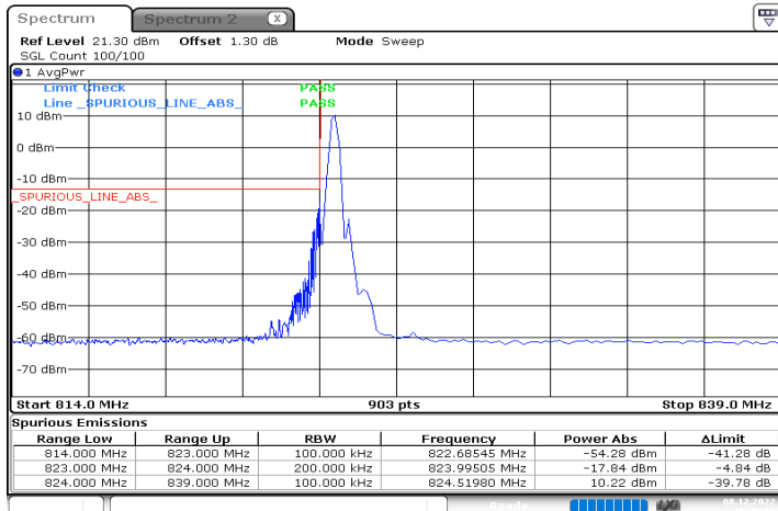
n5_15MHz_15kHz_831.5MHz_DFT-s-OFDM QPSK_RB1@0
