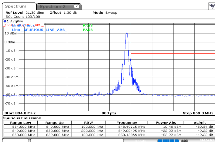
n5_15MHz_15kHz_841.5MHz_DFT-s-OFDM QPSK_RB1@78
