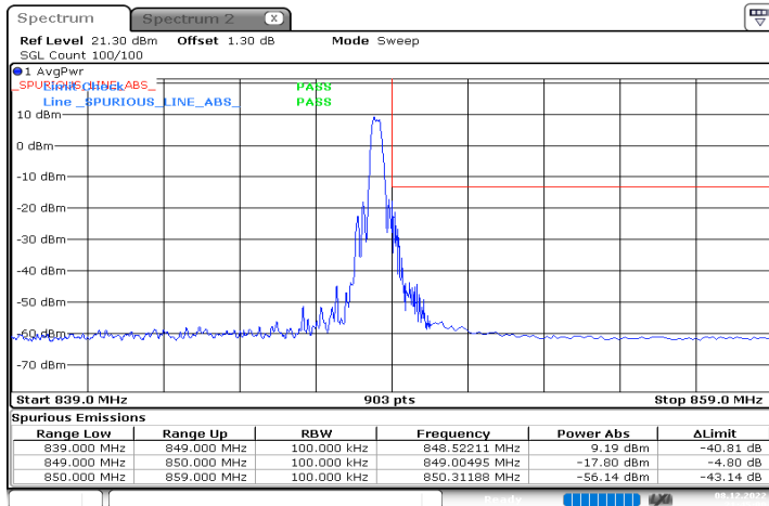
n5_10MHz_15kHz_844MHz_DFT-s-OFDM QPSK_RB1@51
