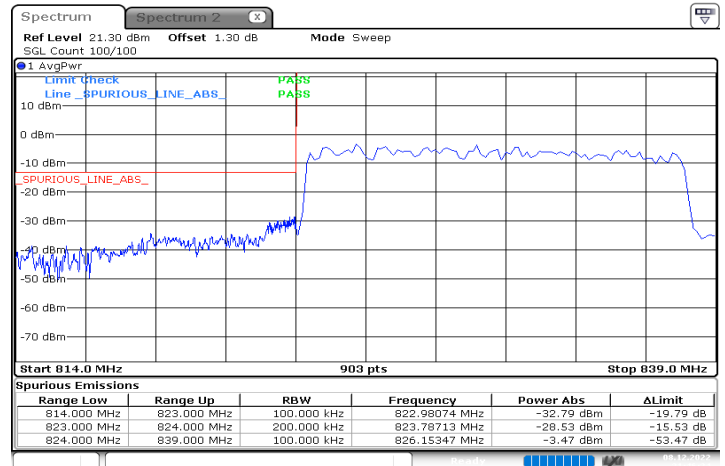
n5_15MHz_15kHz_831.5MHz_DFT-s-OFDM QPSK_RB75@0
