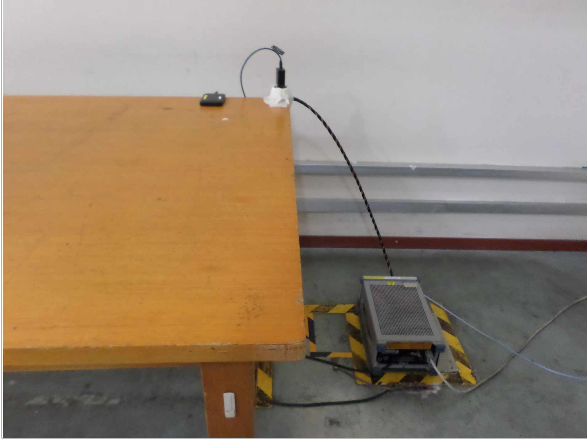
Conducted Emission_Front
