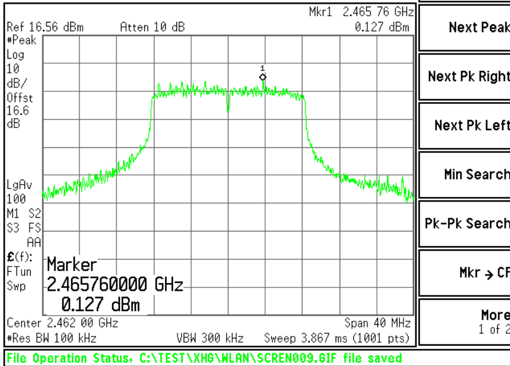
Plot #25 Band Edge {802.11g / 36 Mbps / 2 462 MHz}l
