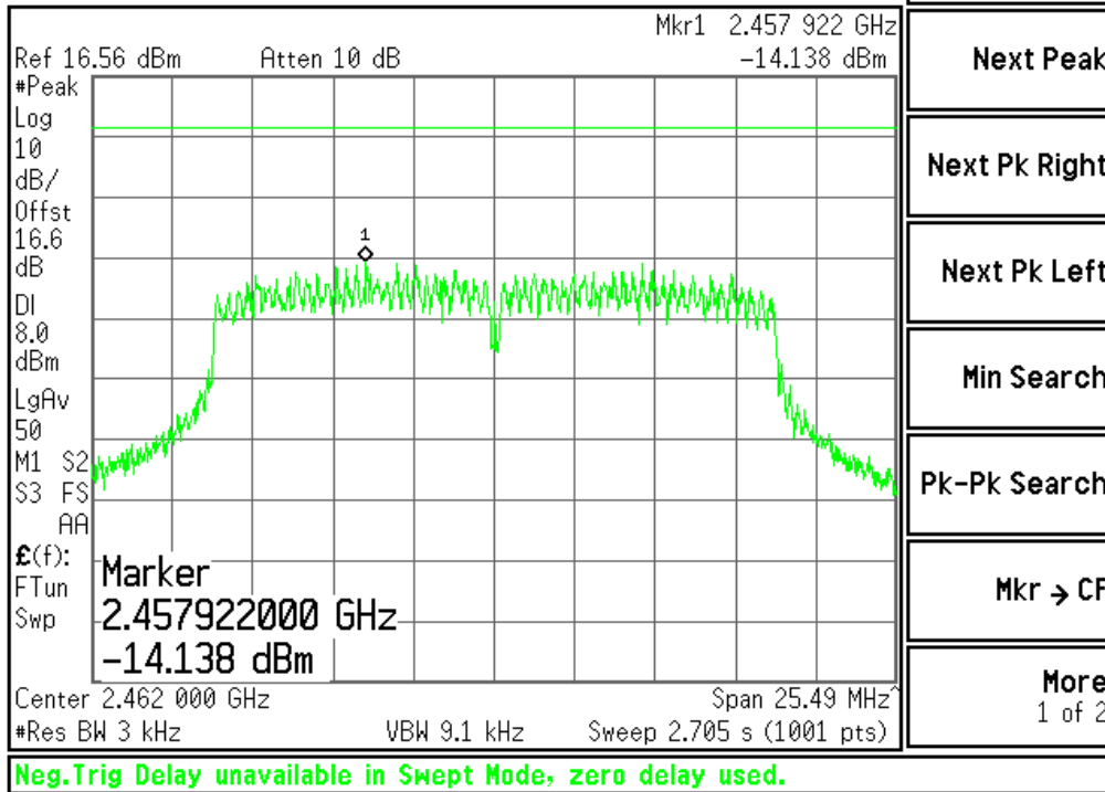
Plot #9 {802.11n / MCS6 / 2 462 MHz}
