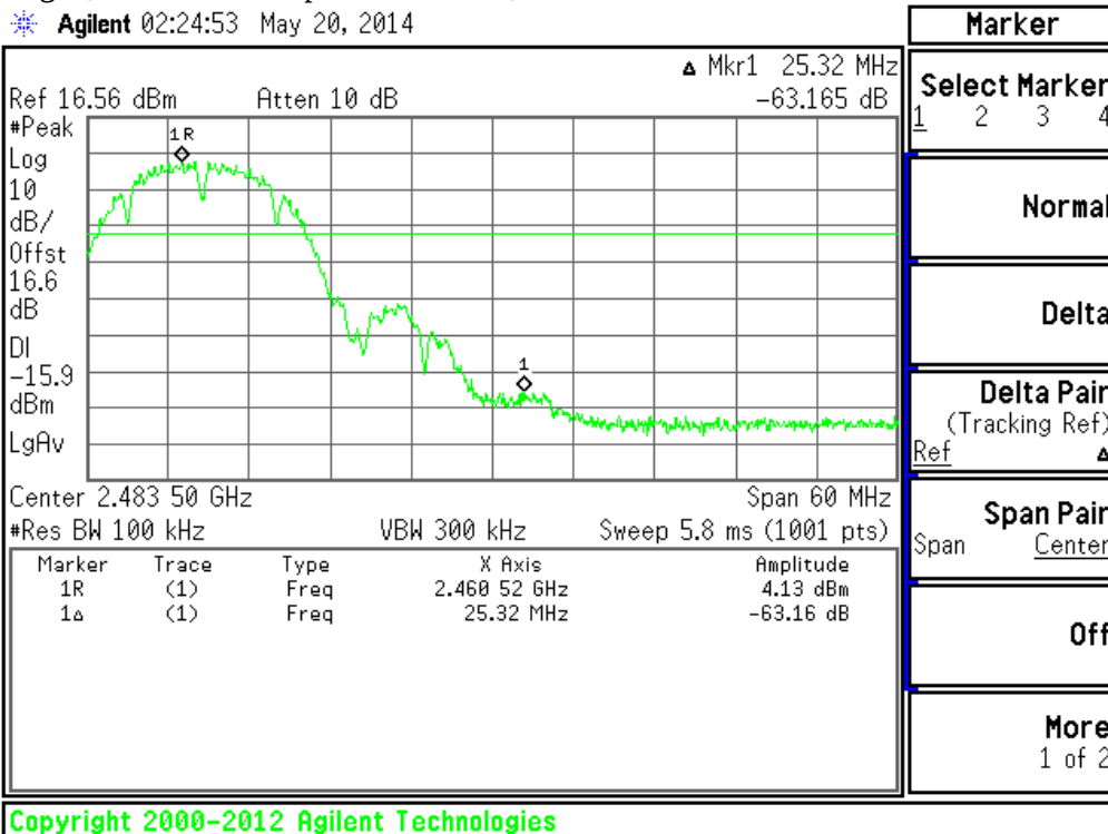
Plot #11 Band Edge {802.11b / 1 Mbps / 2 462 MHz}l
