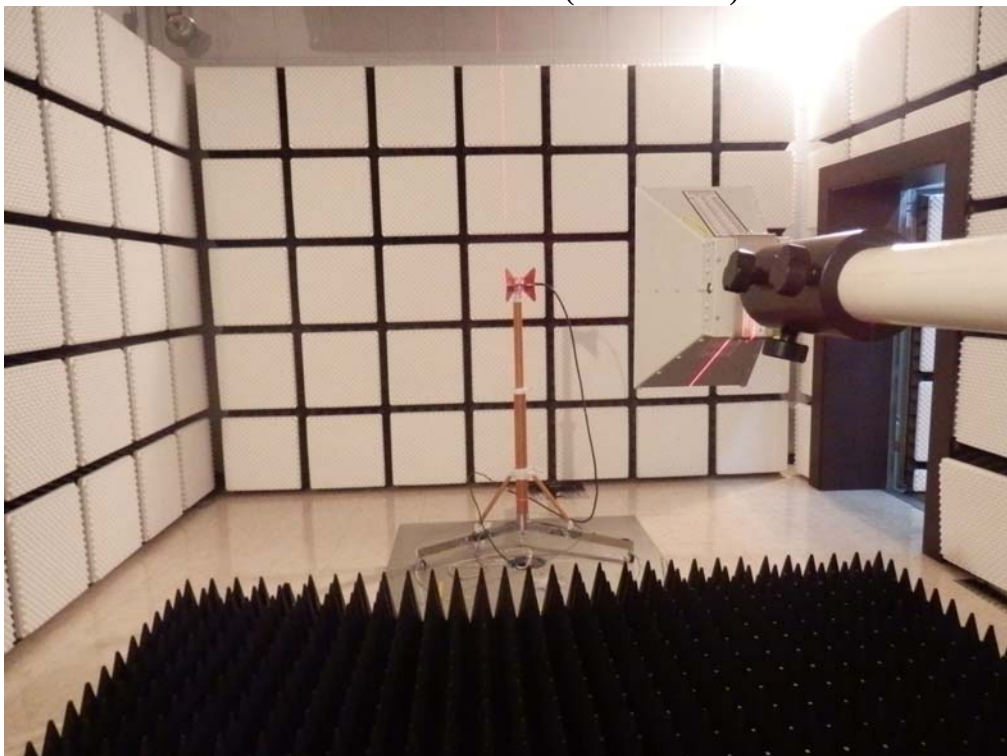
EIRP substitute method (1 GHz above)
