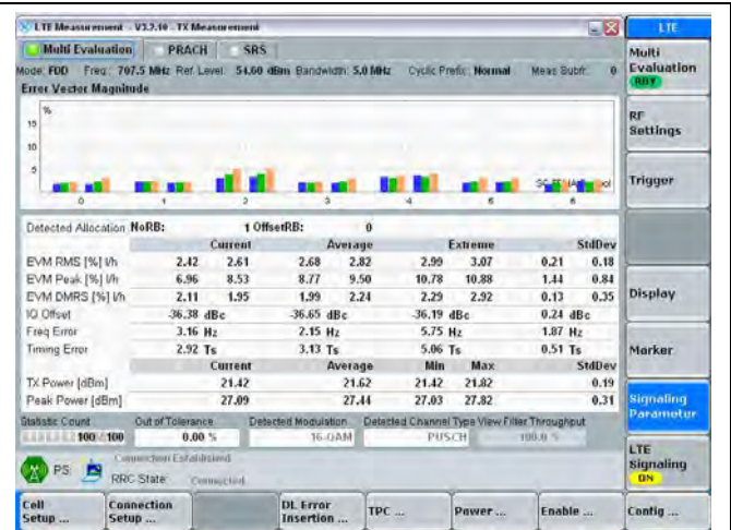
16QAM/RB1#0
