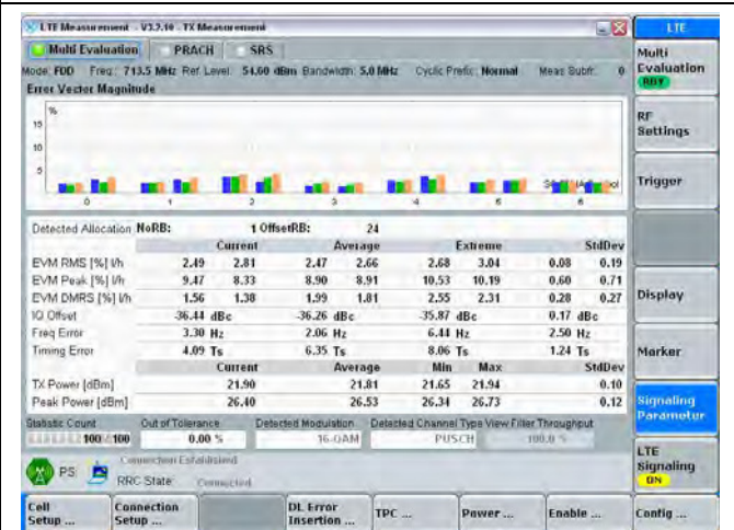
16QAM/RB1#24
