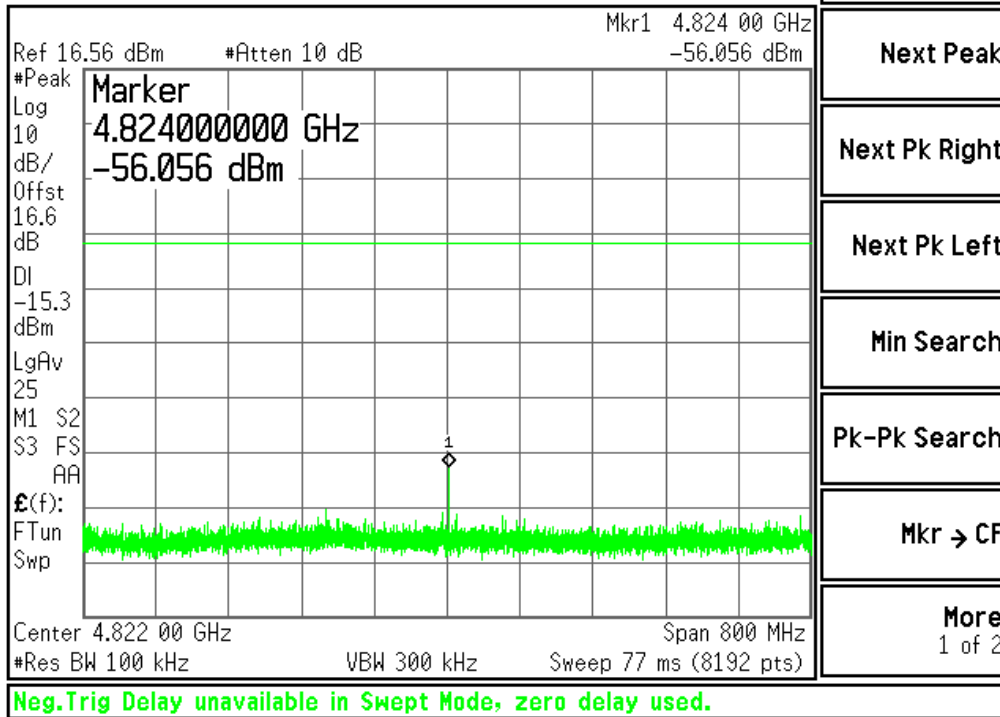
Plot #5 Out of Band Zoom{802.11b / 1 Mbps / 2 412 MHz}
