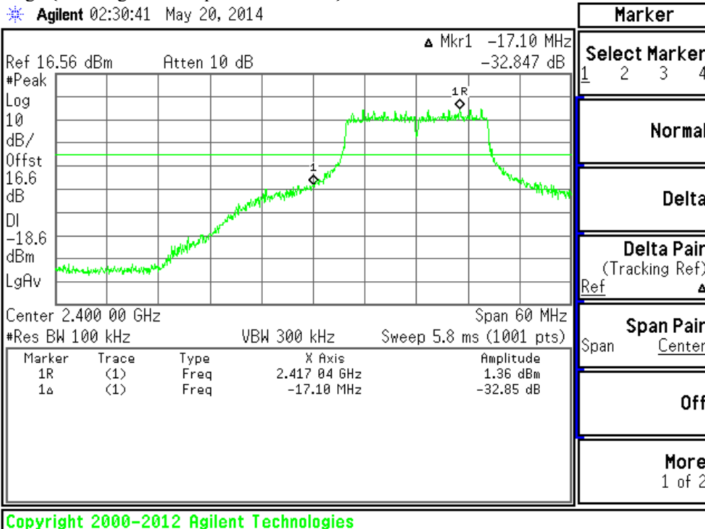
Plot #16 Band Edge {802.11g / 36 Mbps / 2 412 MHz}
