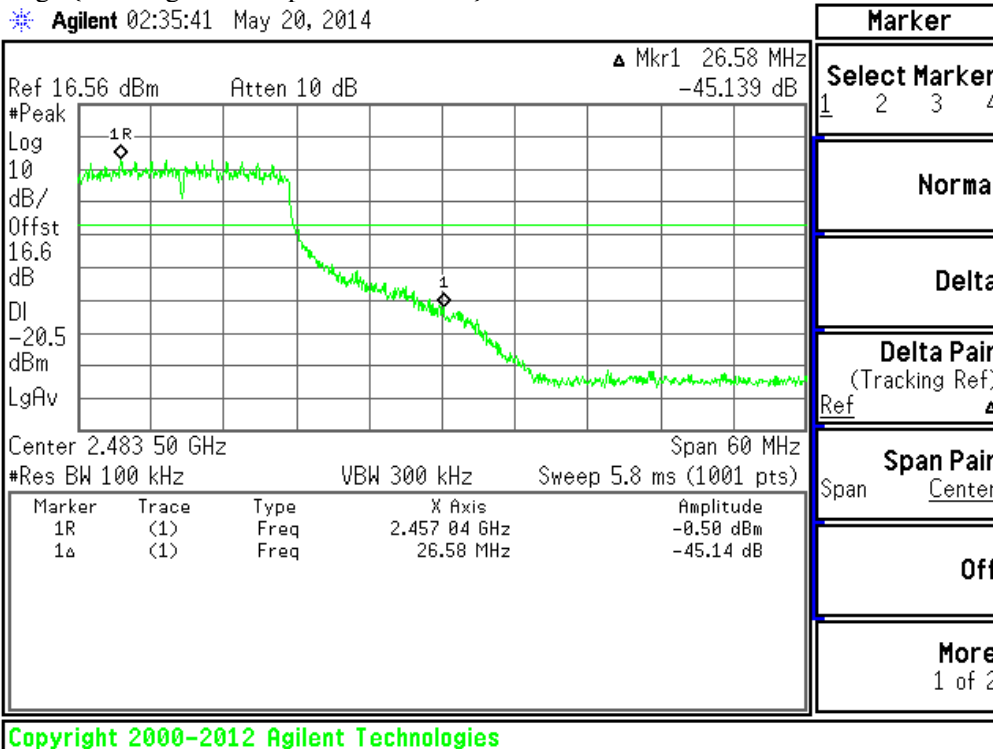
Plot #39 Band Edge {802.11g / 36 Mbps / 2 462 MHz}1
