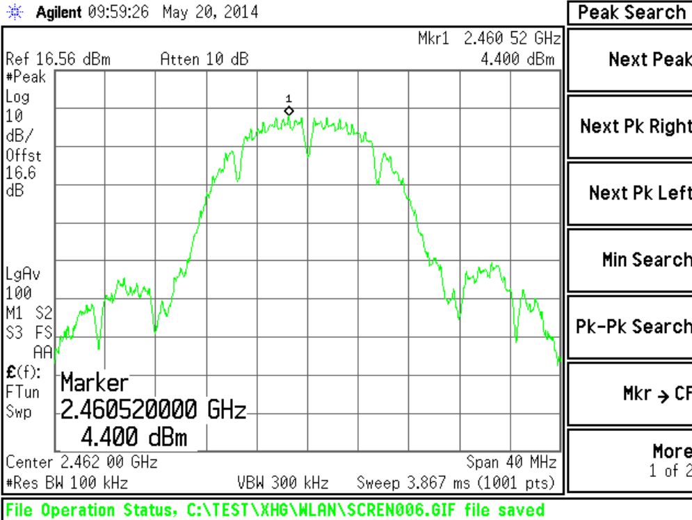
Plot #10 Reference Level {802.11b / 1 Mbps / 2 462 MHz}
