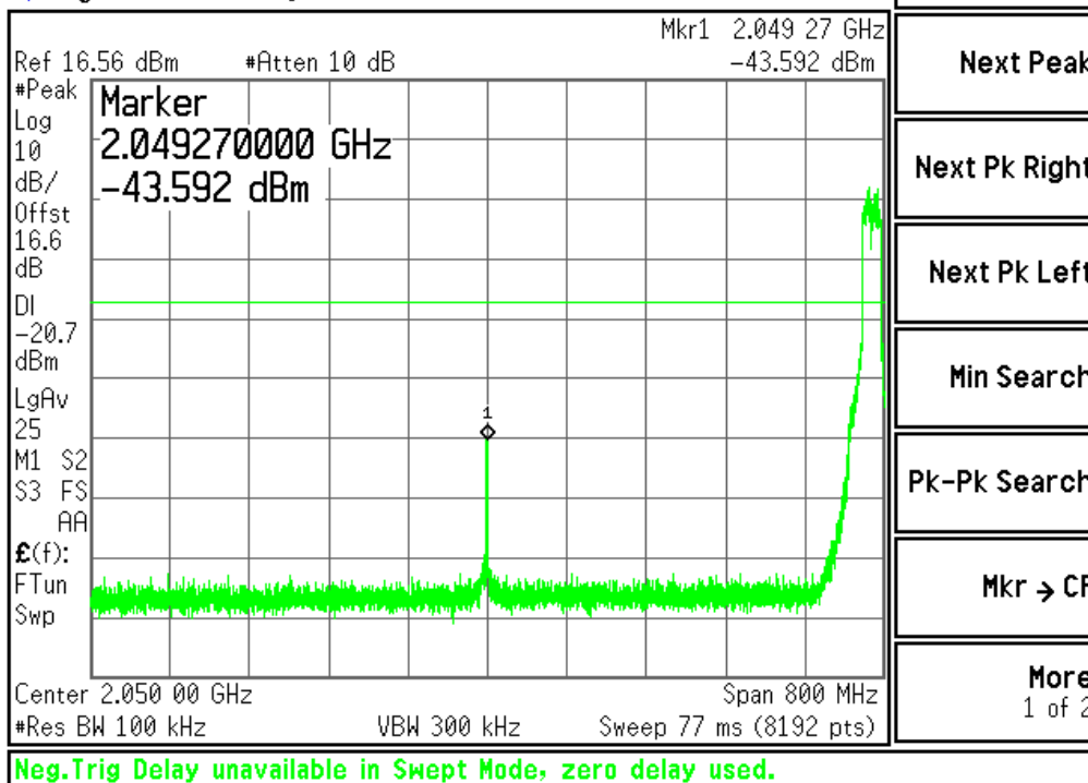
Plot #37 Out of Band Zoom{802.11g / 36 Mbps / 2 437 MHz}
