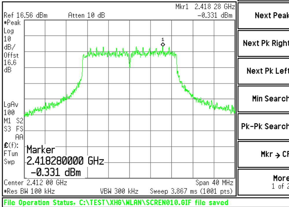
Plot #30 Band Edge {802.11g / 36 Mbps / 2 412 MHz}
