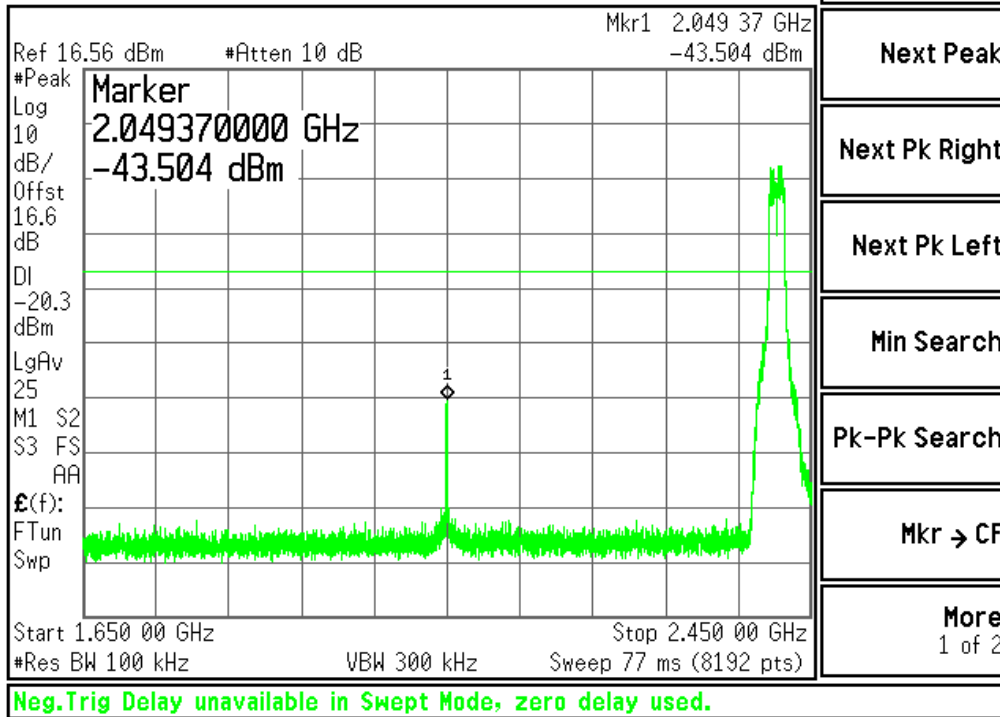
Plot #33 Out of Band Zoom{802.11g / 36 Mbps / 2 412 MHz}
