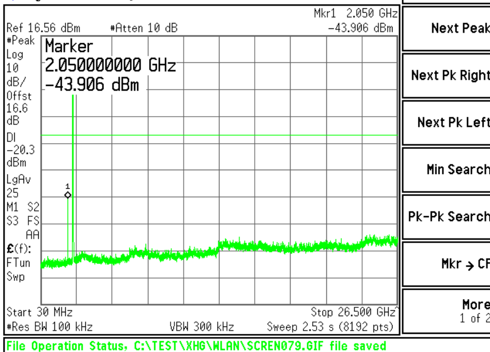
Plot #32 Out of Band 2{802.11g / 36 Mbps / 2 412 MHz}
