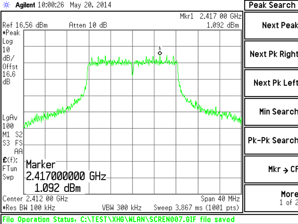
Plot #15 Reference Level {802.11g / 36 Mbps / 2 412 MHz}
