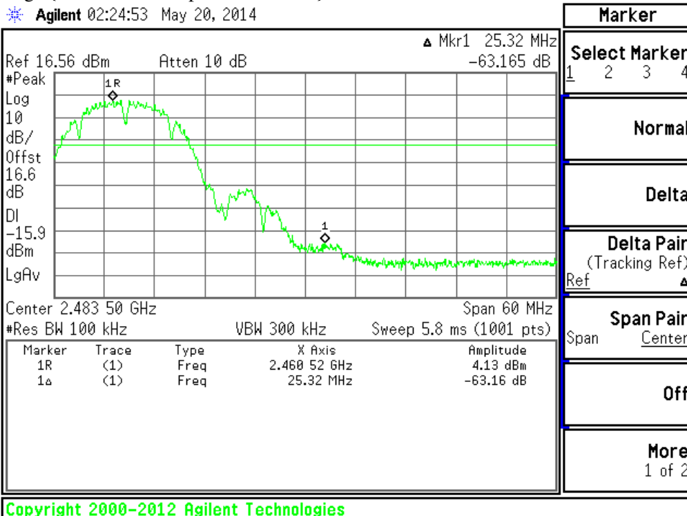
Plot #11 Band Edge {802.11b / 1 Mbps / 2 462 MHz}1
