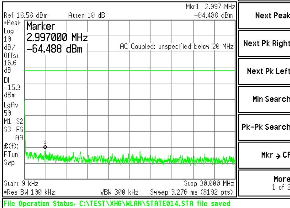
Plot #4 Out of Band 2{802.11b / 1 Mbps / 2 412 MHz}
