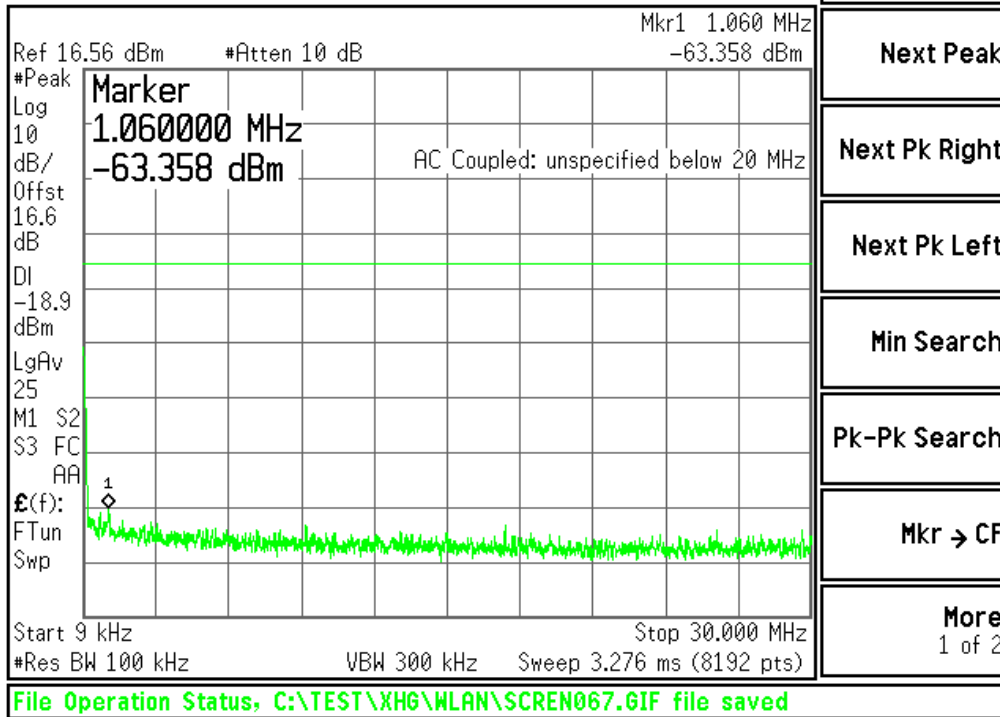
Plot #18 Out of Band 2{802.11g / 36 Mbps / 2 412 MHz}
