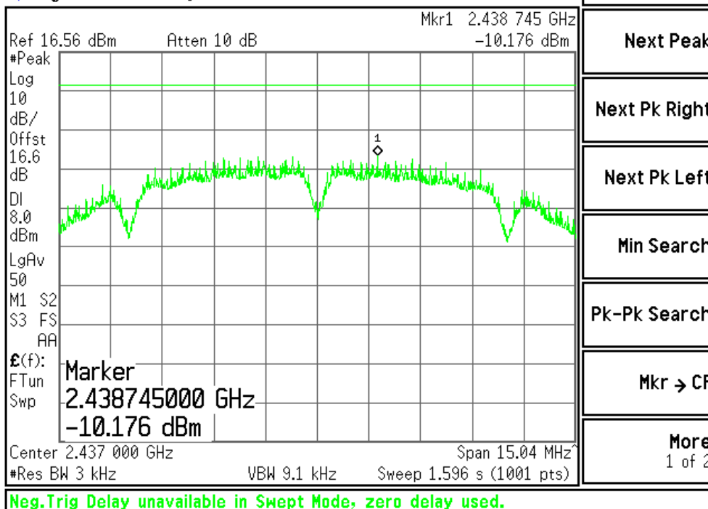
Plot #2 {802.11b / 1 Mbps / 2 437 MHz}
