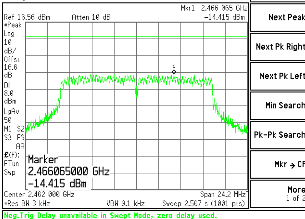
Plot #6 {802.11g / 36 Mbps / 2 462 MHz}
