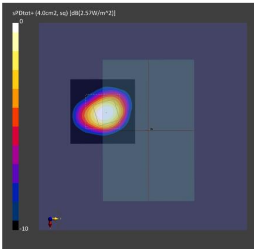
Figure 8-2: 4cm2-averaged power density distribution measured at input.power.limit of 4.64dBm on the Front for n260 beam 27
