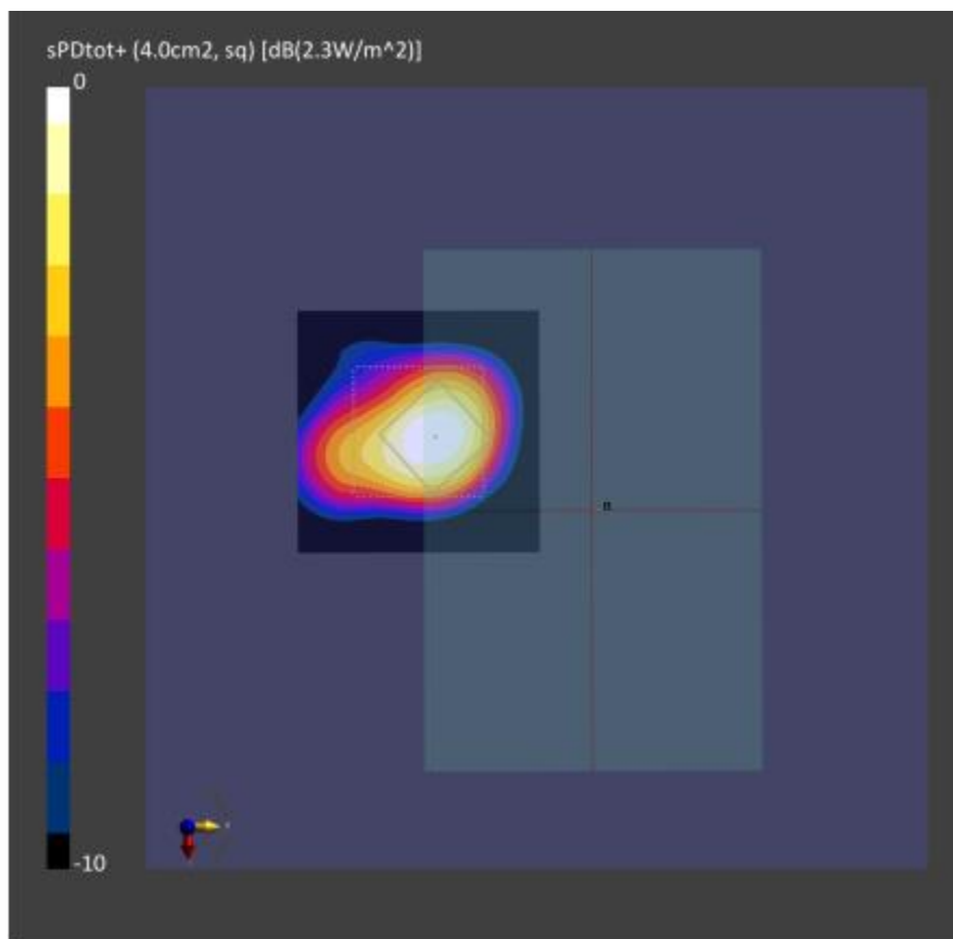
Figure 8-3: 4cm2-averaged power density distribution measured at input.power.limit of 4.81dBm on the Front for n261 beam 28
