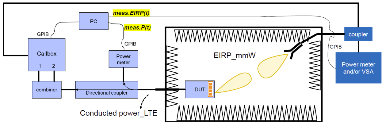
Figure 7-1 mmW NR radiated power measurement setup
