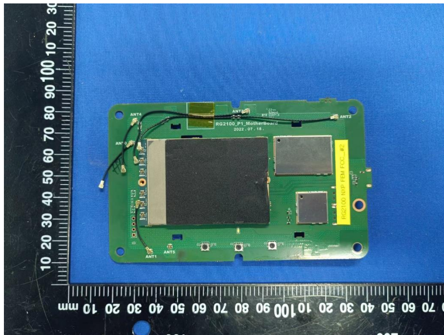
MAIN BOARD TOP VIEW 1 (WITH SHIELDING)
