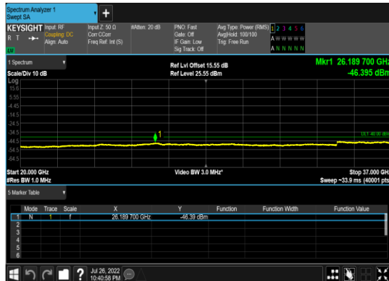
N48(20M)_DFT-s- OFDM_QPSK_Edge_1RB_Right_Low_CH
