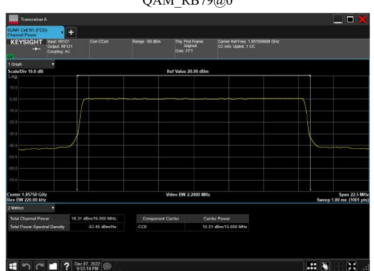
n2_15MHz_15kHz_1857.5MHz_CP-OFDM 256 QAM_RB79@0
