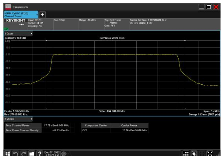
n2_5MHz_15kHz_1907.5MHz_CP-OFDM 256 QAM_RB25@0
