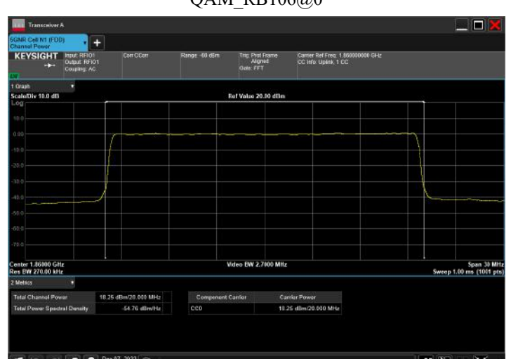
n2_20MHz_15kHz_1860MHz_CP-OFDM 256 QAM_RB106@0
