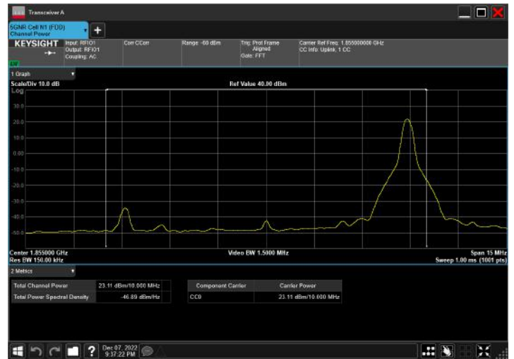
n2_10MHz_15kHz_1855MHz_CP-OFDM 16 QAM_RB52@0
