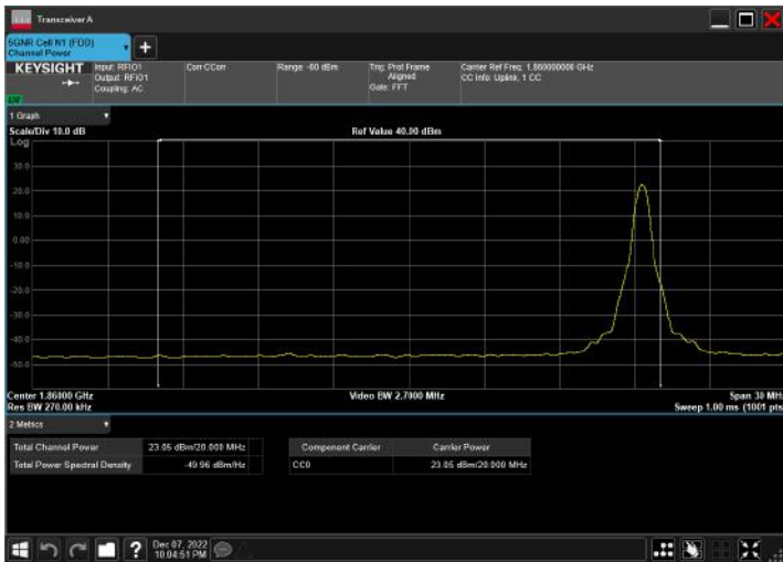
n2_20MHz_15kHz_1860MHz_DFT-s-OFDM 16 QAM_RB100@0
