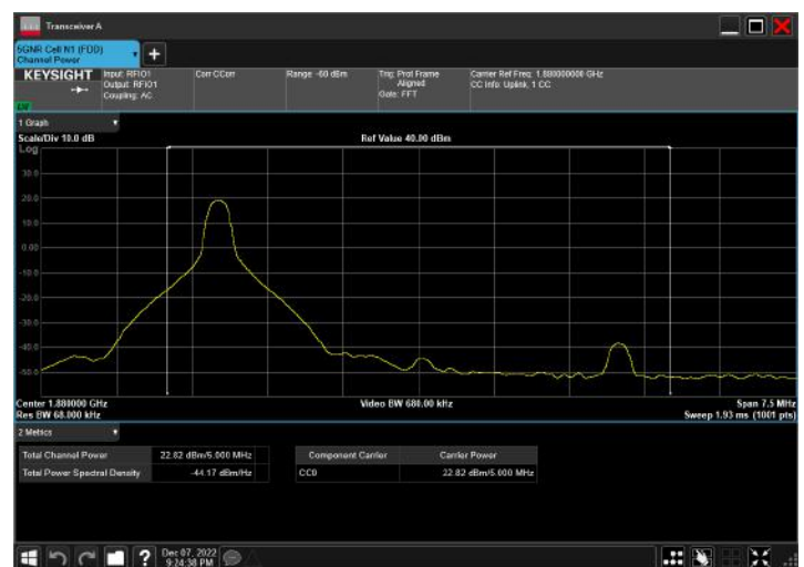
n2_5MHz_15kHz_1880MHz_DFT-s-OFDM QPSK_RB1@1
