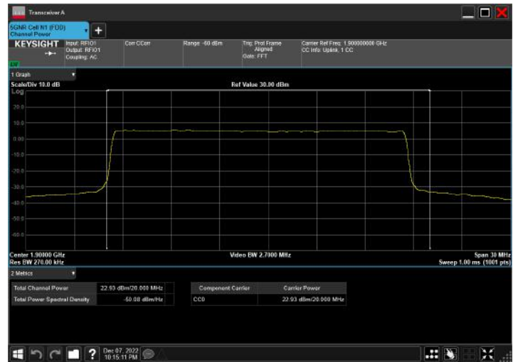
n2_20MHz_15kHz_1900MHz_DFT-s-OFDM 64 QAM_RB100@0
