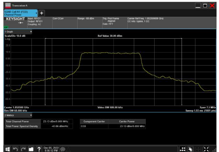
n2_5MHz_15kHz_1852.5MHz_DFT-s-OFDM PI/2 BPSK_RB12@6
