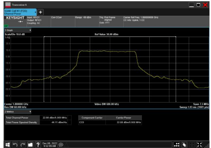
n2_5MHz_15kHz_1880MHz_CP-OFDM QPSK_RB1@1
