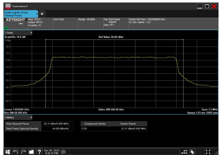
n2_5MHz_15kHz_1852.5MHz_DFT-s-OFDM 64 QAM_RB25@0
