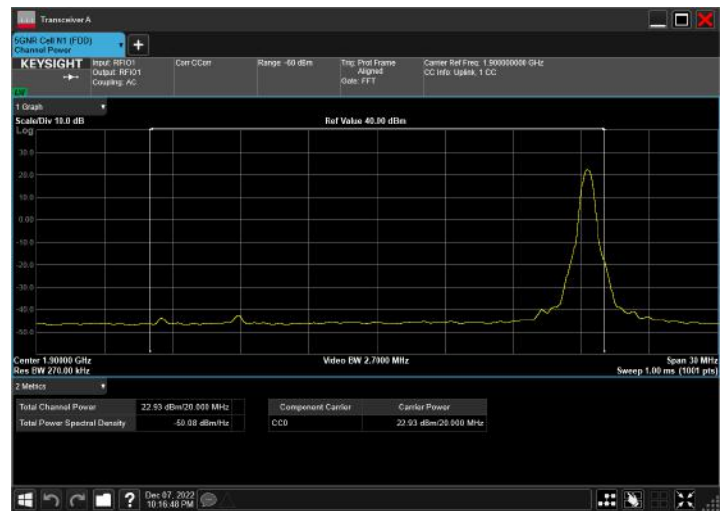
n2_20MHz_15kHz_1900MHz_CP-OFDM 16 QAM_RB106@0
