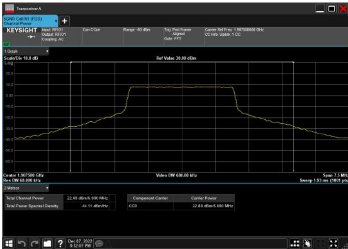
n2_5MHz_15kHz_1907.5MHz_CP-OFDM QPSK_RB25@0
