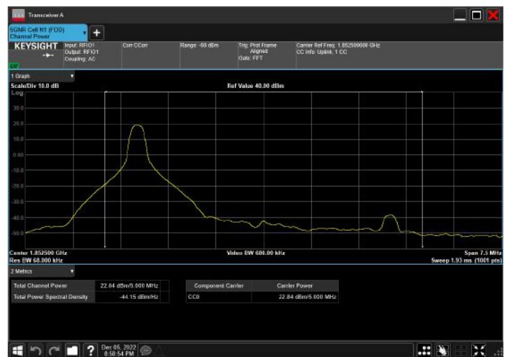
n2_5MHz_15kHz_1852.5MHz_CP-OFDM QPSK_RB1@1
