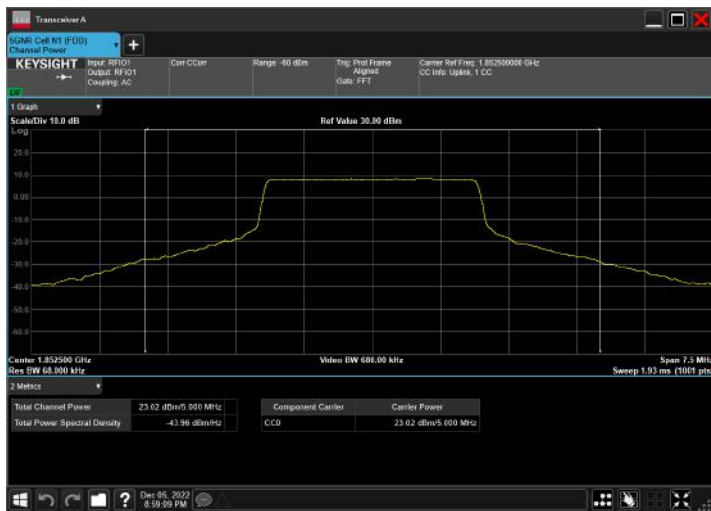
n2_5MHz_15kHz_1852.5MHz_CP-OFDM QPSK_RB25@0
