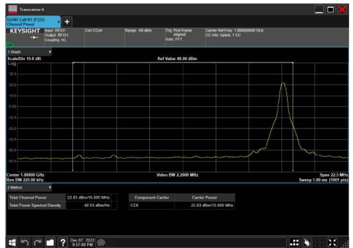
n2_15MHz_15kHz_1880MHz_CP-OFDM 16 QAM_RB79@0
