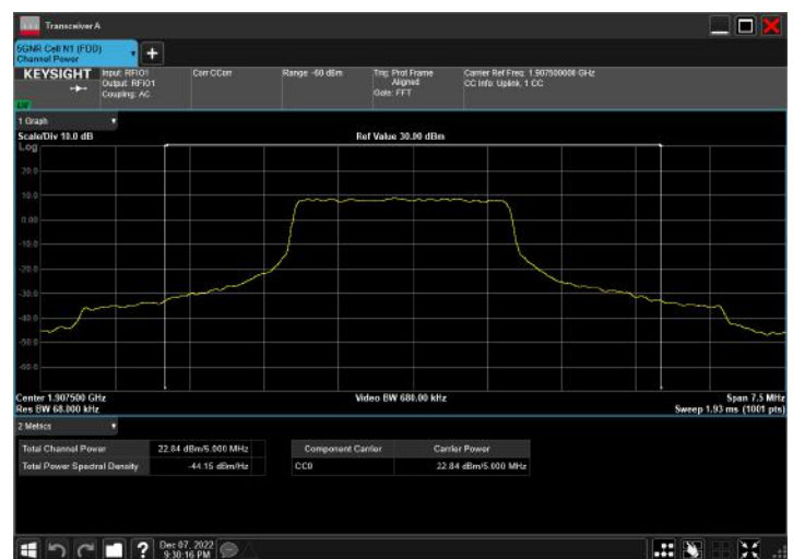
n2_5MHz_15kHz_1907.5MHz_DFT-s-OFDM QPSK_RB12@6
