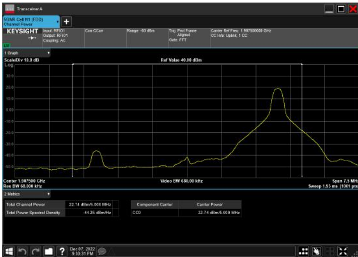
n2_5MHz_15kHz_1907.5MHz_DFT-s-OFDM 16 QAM_RB25@0
