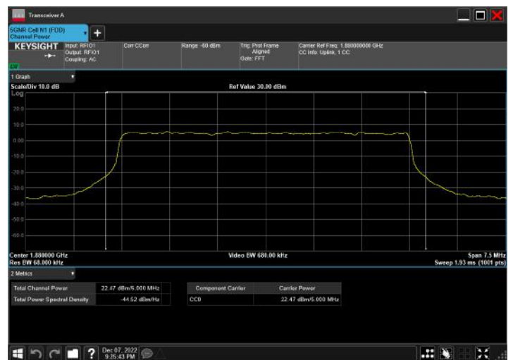
n2_5MHz_15kHz_1880MHz_DFT-s-OFDM 256 QAM_RB25@0
