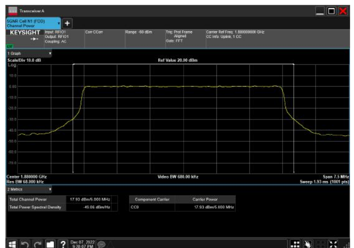
n2_5MHz_15kHz_1880MHz_CP-OFDM 256 QAM_RB25@0
