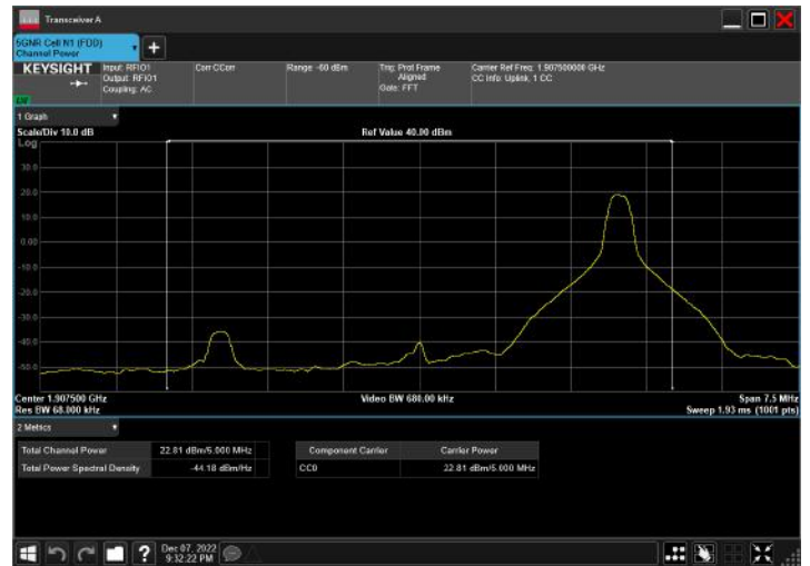
n2_5MHz_15kHz_1907.5MHz_CP-OFDM 16 QAM_RB25@0
