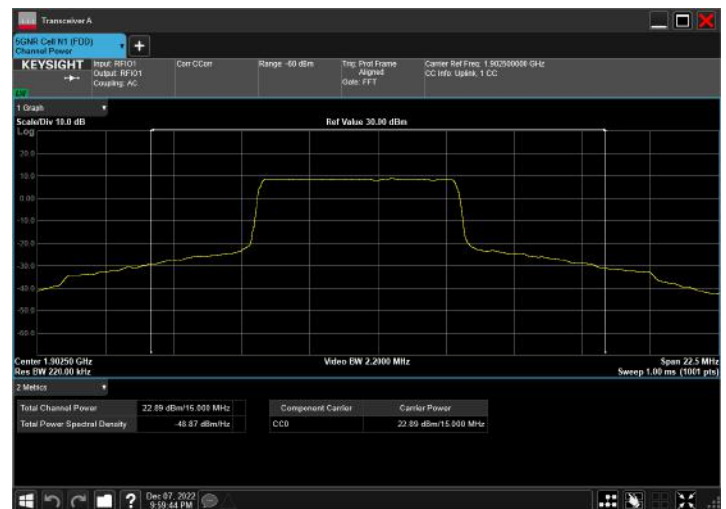
n2_15MHz_15kHz_1902.5MHz_DFT-s-OFDM QPSK_RB36@18
