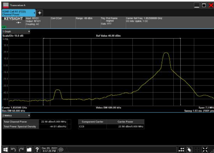
n2_5MHz_15kHz_1852.5MHz_DFT-s-OFDM 16 QAM_RB25@0
