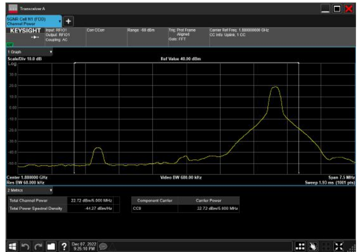
n2_5MHz_15kHz_1880MHz_DFT-s-OFDM 16 QAM_RB25@0
