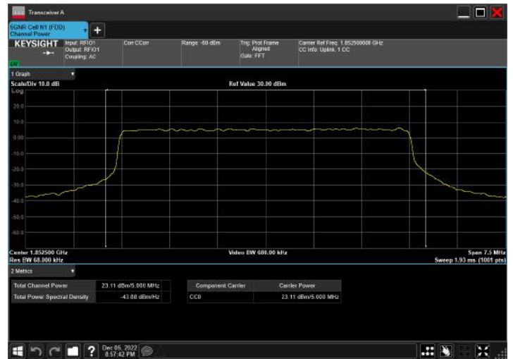
n2_5MHz_15kHz_1852.5MHz_DFT-s-OFDM 64 QAM_RB25@0
