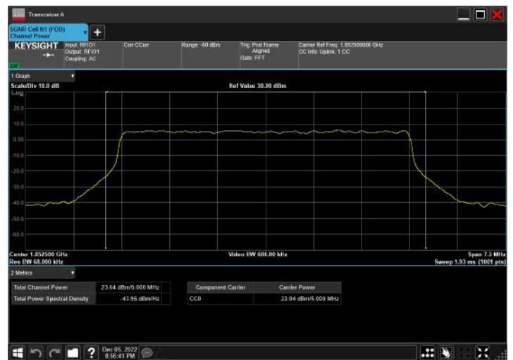
n2_5MHz_15kHz_1852.5MHz_DFT-s-OFDM QPSK_RB12@6
