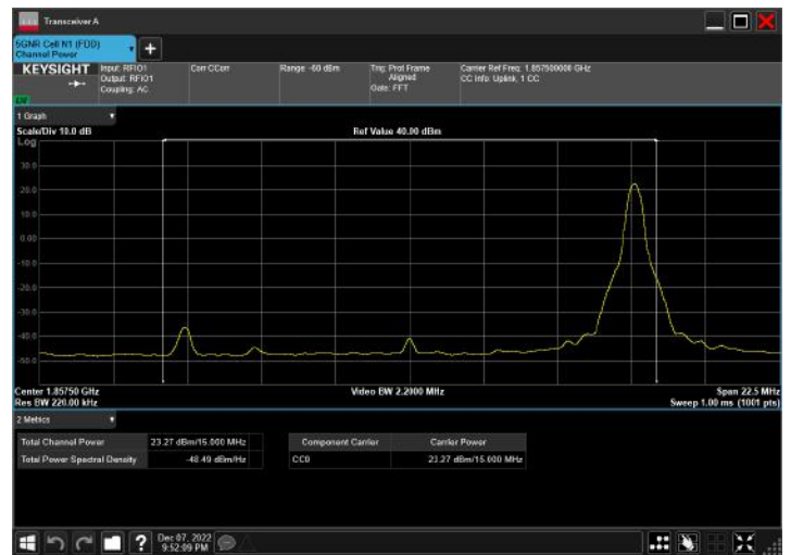
n2_15MHz_15kHz_1857.5MHz_CP-OFDM 16 QAM_RB79@0
