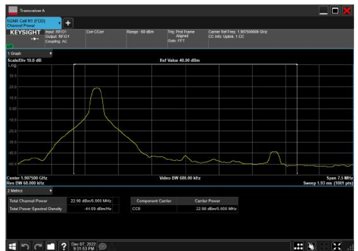
n2_5MHz_15kHz_1907.5MHz_CP-OFDM QPSK_RB1@1
