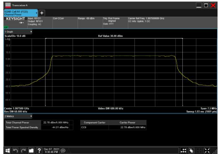
n2_5MHz_15kHz_1907.5MHz_DFT-s-OFDM 64 QAM_RB25@0
