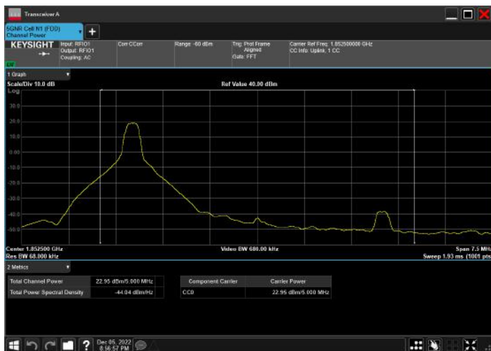
n2_5MHz_15kHz_1852.5MHz_DFT-s-OFDM QPSK_RB1@1
