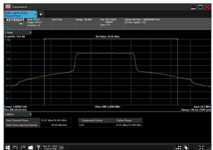
n2_15MHz_15kHz_1880MHz_DFT-s-OFDM QPSK_RB36@18
