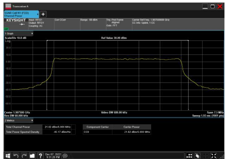
n2_5MHz_15kHz_1907.5MHz_DFT-s-OFDM 64 QAM_RB25@0
