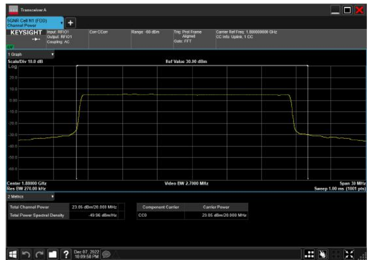
n2_20MHz_15kHz_1880MHz_DFT-s-OFDM 64 QAM_RB100@0
