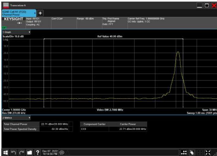
n2_20MHz_15kHz_1900MHz_DFT-s-OFDM 16 QAM_RB100@0
