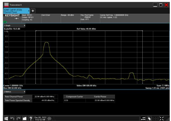
n2_5MHz_15kHz_1880MHz_CP-OFDM QPSK_RB1@1
