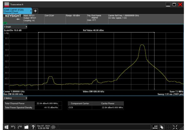
n2_5MHz_15kHz_1880MHz_CP-OFDM 16 QAM_RB25@0
