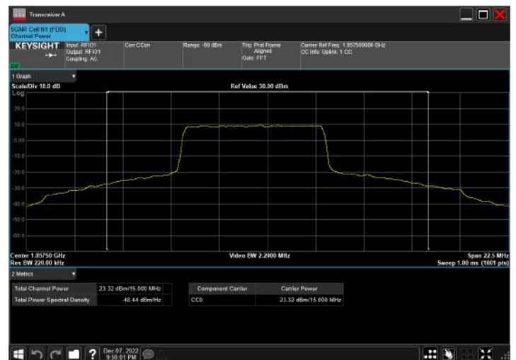
n2_15MHz_15kHz_1857.5MHz_DFT-s-OFDM QPSK_RB36@18
