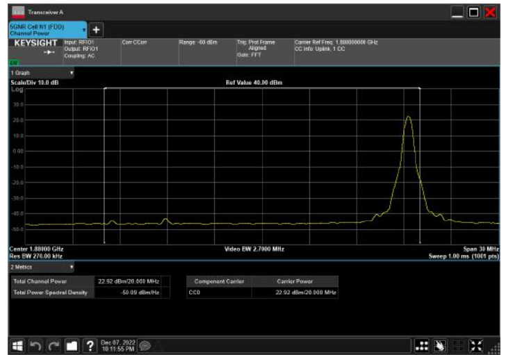
n2_20MHz_15kHz_1880MHz_CP-OFDM 16 QAM_RB106@0
