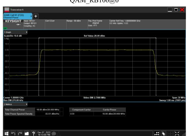
n2_20MHz_15kHz_1880MHz_CP-OFDM 256 QAM_RB106@0
