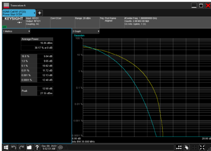
n2_15MHz_15kHz_1880MHz_CP-OFDM 256 QAM_RB79@0
