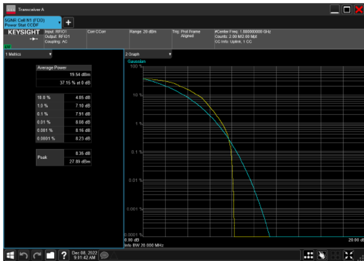
n2_15MHz_15kHz_1880MHz_DFT-s-OFDM 16 QAM_RB75@0
