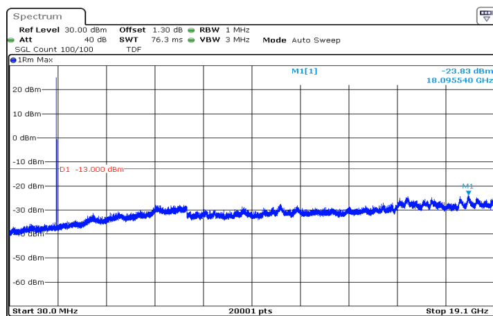
n2_10MHz_15kHz_1880MHz_DFT-s-OFDM QPSK_RB1@0|30MHz_19.1GHz
