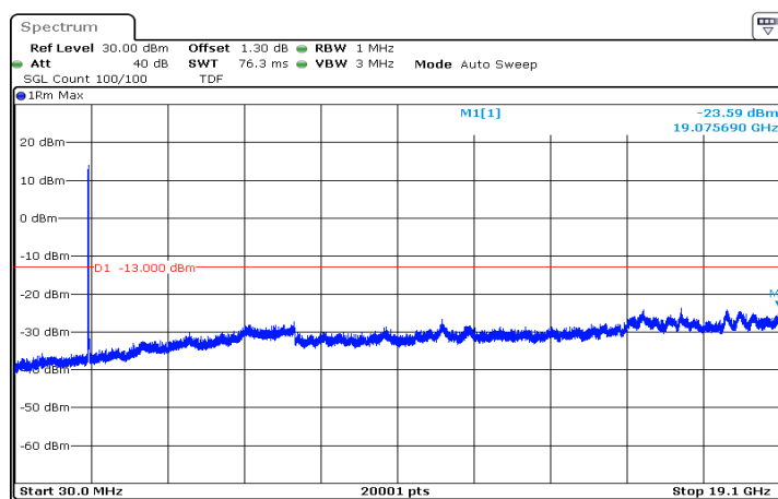
n2_15MHz_15kHz_1857.5MHz_DFT-s-OFDM QPSK_RB75@0|30MHz_19.1GHz
