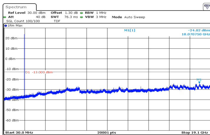
n2_15MHz_15kHz_1880MHz_DFT-s-OFDM QPSK_RB1@78|30MHz_19.1GHz
