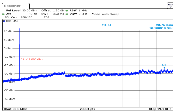
n2_10MHz_15kHz_1905MHz_DFT-s-OFDM QPSK_RB1@0|30MHz_19.1GHz
