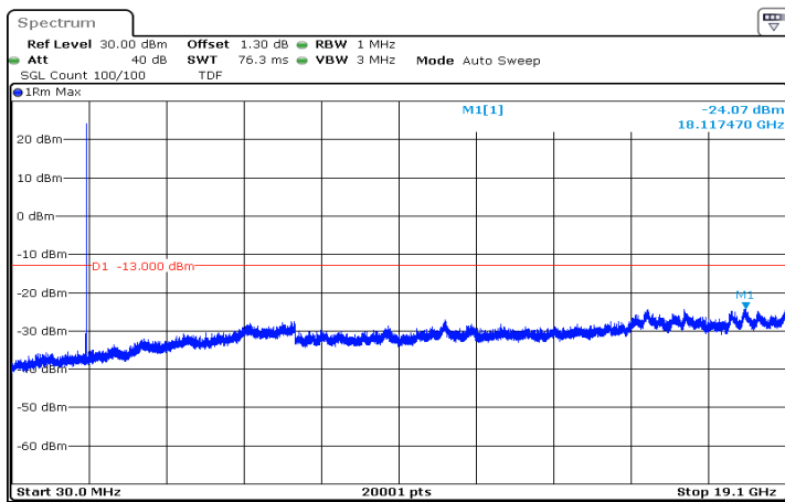
n2_10MHz_15kHz_1855MHz_DFT-s-OFDM QPSK_RB1@51|30MHz_19.1GHz
