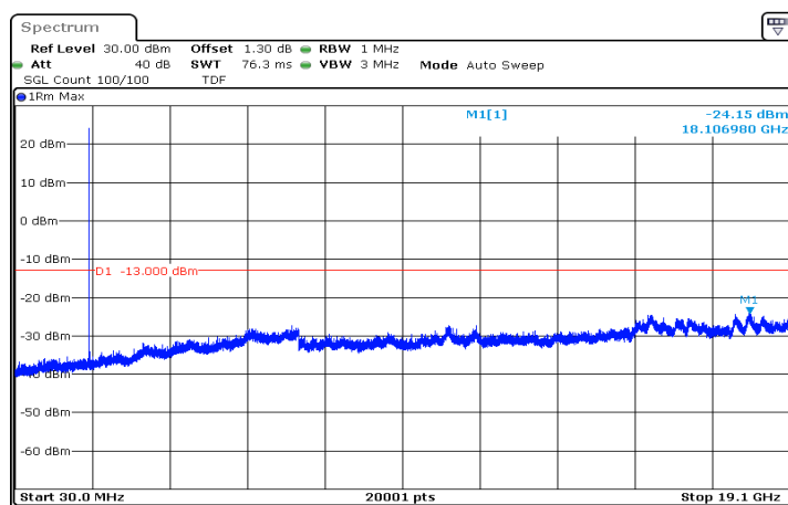
n2_20MHz_15kHz_1860MHz_DFT-s-OFDM QPSK_RB1@0|30MHz_19.1GHz
