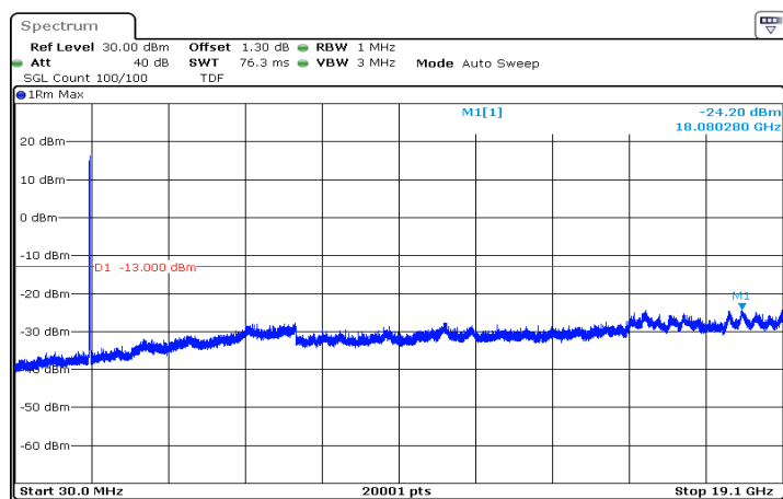
n2_15MHz_15kHz_1880MHz_DFT-s-OFDM QPSK_RB75@0|30MHz_19.1GHz
