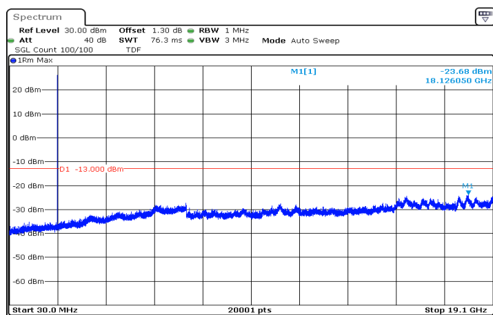
n2_15MHz_15kHz_1902.5MHz_DFT-s-OFDM QPSK_RB1@78|30MHz_19.1GHz
