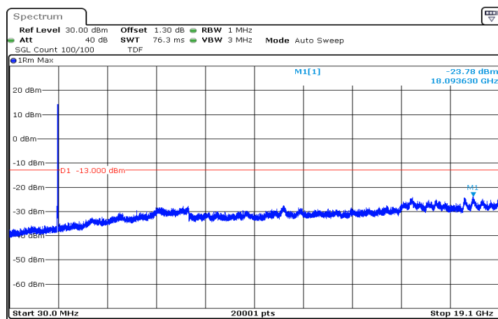
n2_20MHz_15kHz_1900MHz_DFT-s-OFDM QPSK_RB100@0|30MHz_19.1GHz
