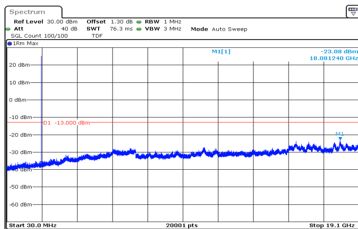
n2_15MHz_15kHz_1902.5MHz_DFT-s-OFDM QPSK_RB1@0|30MHz_19.1GHz
