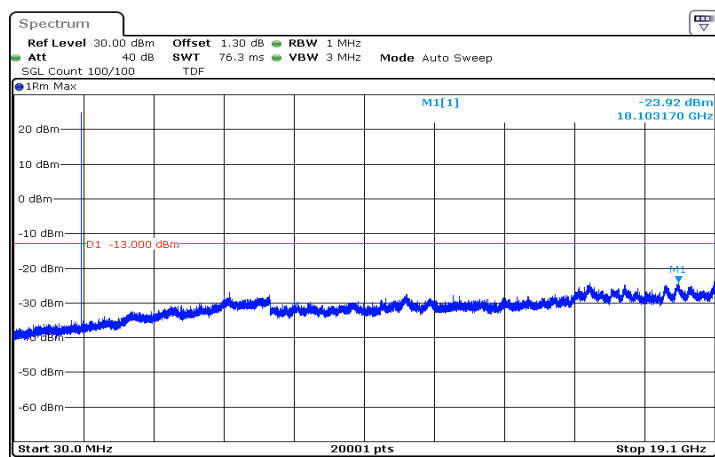
n2_15MHz_15kHz_1880MHz_DFT-s-OFDM QPSK_RB1@0|30MHz_19.1GHz
