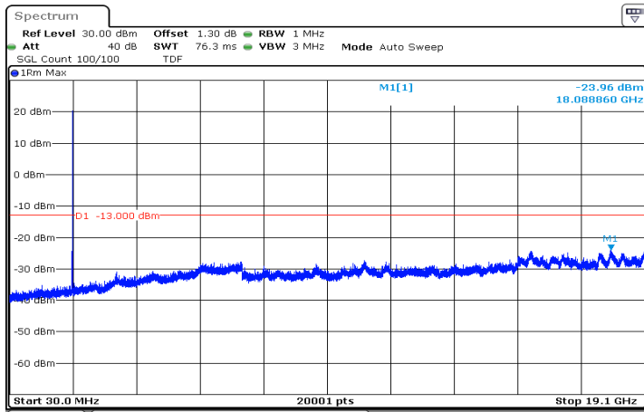
n2_5MHz_15kHz_1907.5MHz_DFT-s-OFDM QPSK_RB25@0|30MHz_19.1GHz
