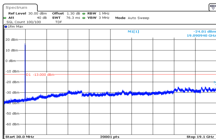
n2_15MHz_15kHz_1902.5MHz_DFT-s-OFDM QPSK_RB75@0|30MHz_19.1GHz
