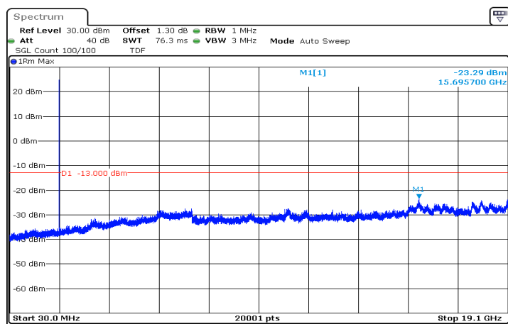
n2_20MHz_15kHz_1900MHz_DFT-s-OFDM QPSK_RB1@105|30MHz_19.1GHz
