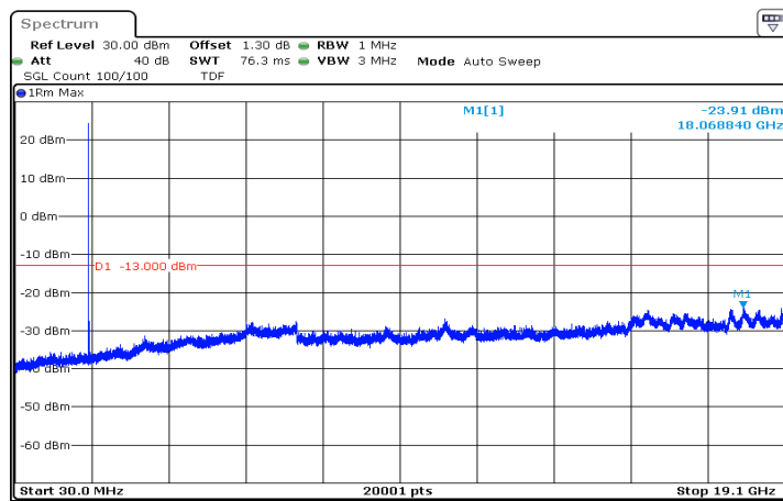
n2_15MHz_15kHz_1857.5MHz_DFT-s-OFDM QPSK_RB1@0|30MHz_19.1GHz
