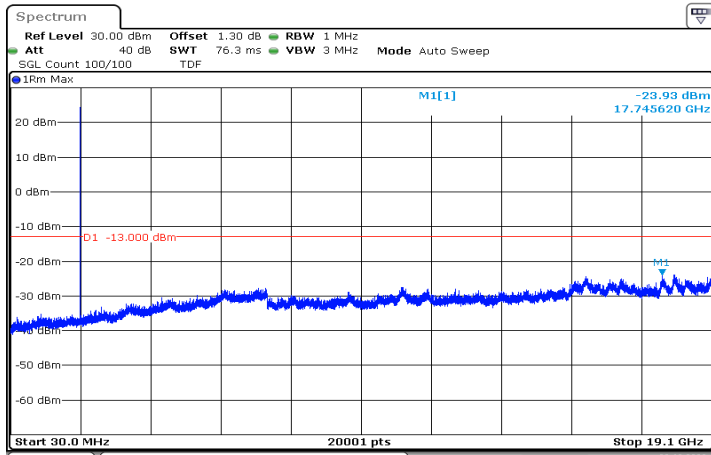
n2_5MHz_15kHz_1907.5MHz_DFT-s-OFDM QPSK_RB1@0|30MHz_19.1GHz
