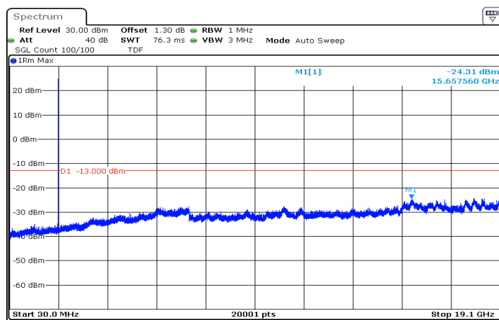
n2_10MHz_15kHz_1905MHz_DFT-s-OFDM QPSK_RB1@51|30MHz_19.1GHz
