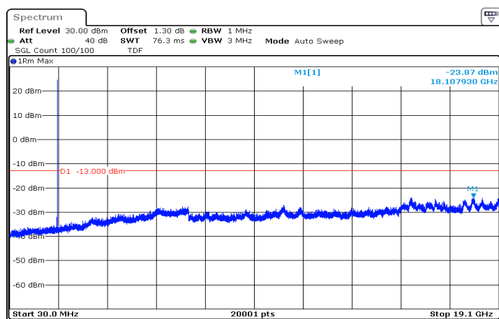
n2_10MHz_15kHz_1880MHz_DFT-s-OFDM QPSK_RB1@51|30MHz_19.1GHz
