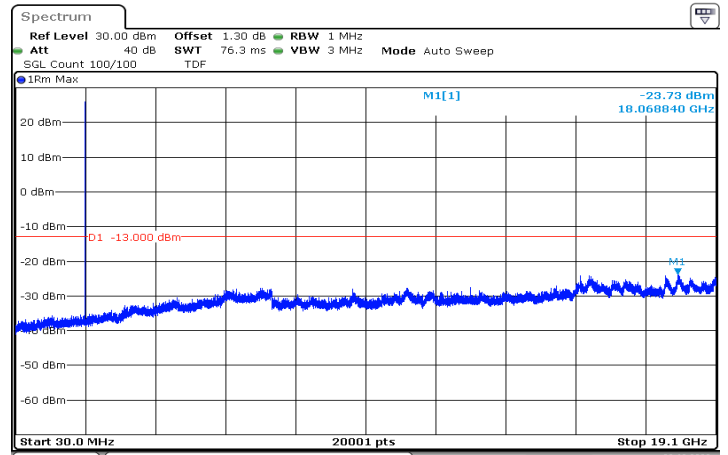
n2_5MHz_15kHz_1907.5MHz_DFT-s-OFDM QPSK_RB1@24|30MHz_19.1GHz
