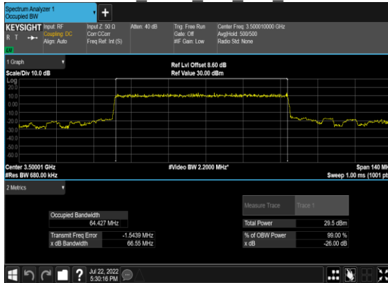
N77(70M)_DFT-s-OFDM_PI_2- BPSK Outer Full Mid CH
