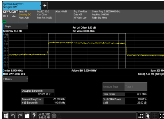
N77(100M)_CP-OFDM_256 QAM_Outer_Full_Mid_CH
