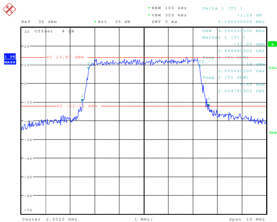
Band 7_5 MHz_Low_16QAM_RB25#0
