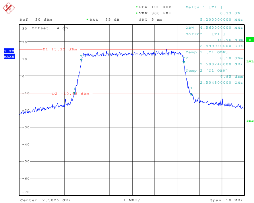
Band 7_5 MHz_Low_QPSK_RB25#0
