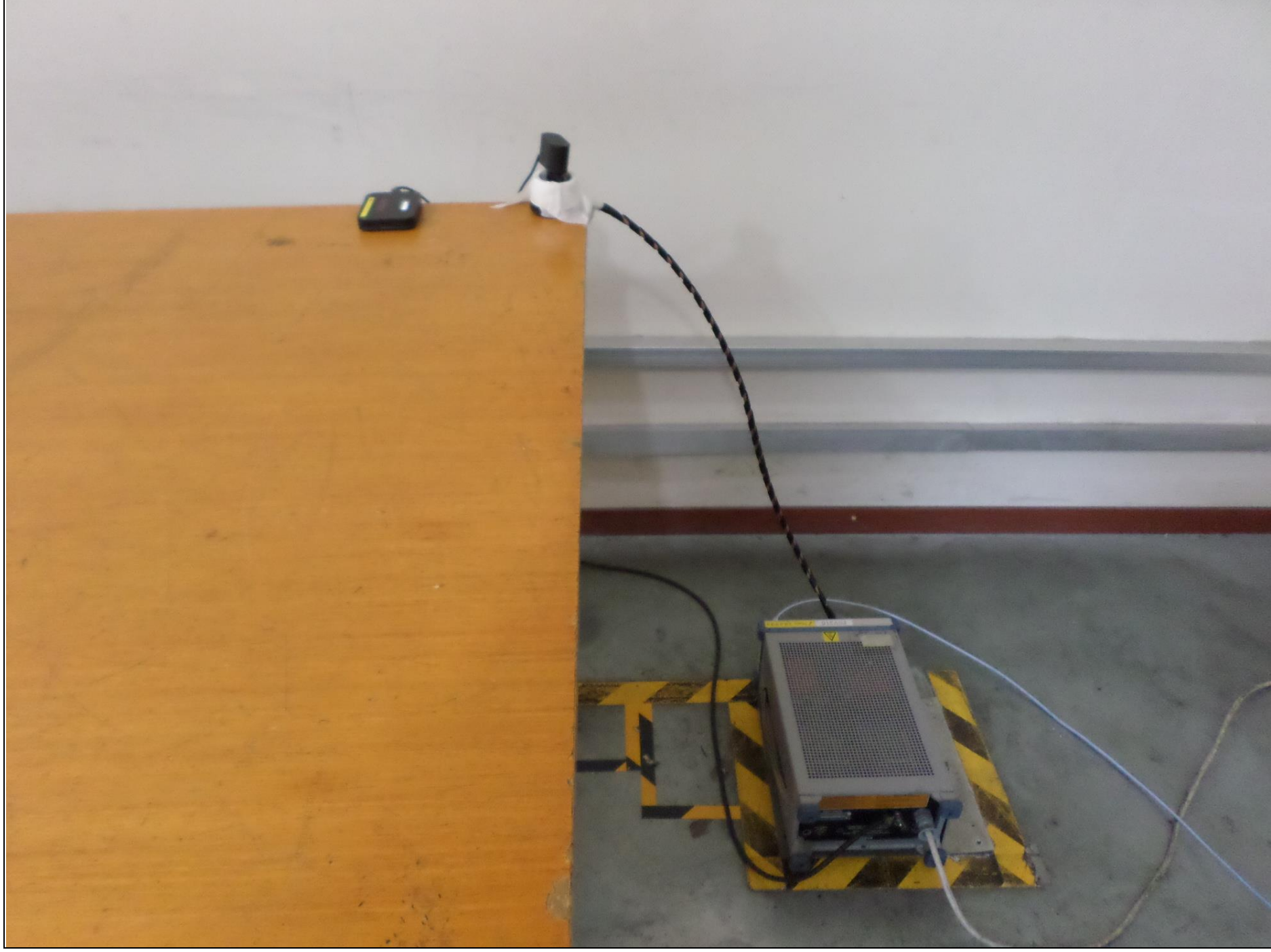
Conducted Emission_Front
