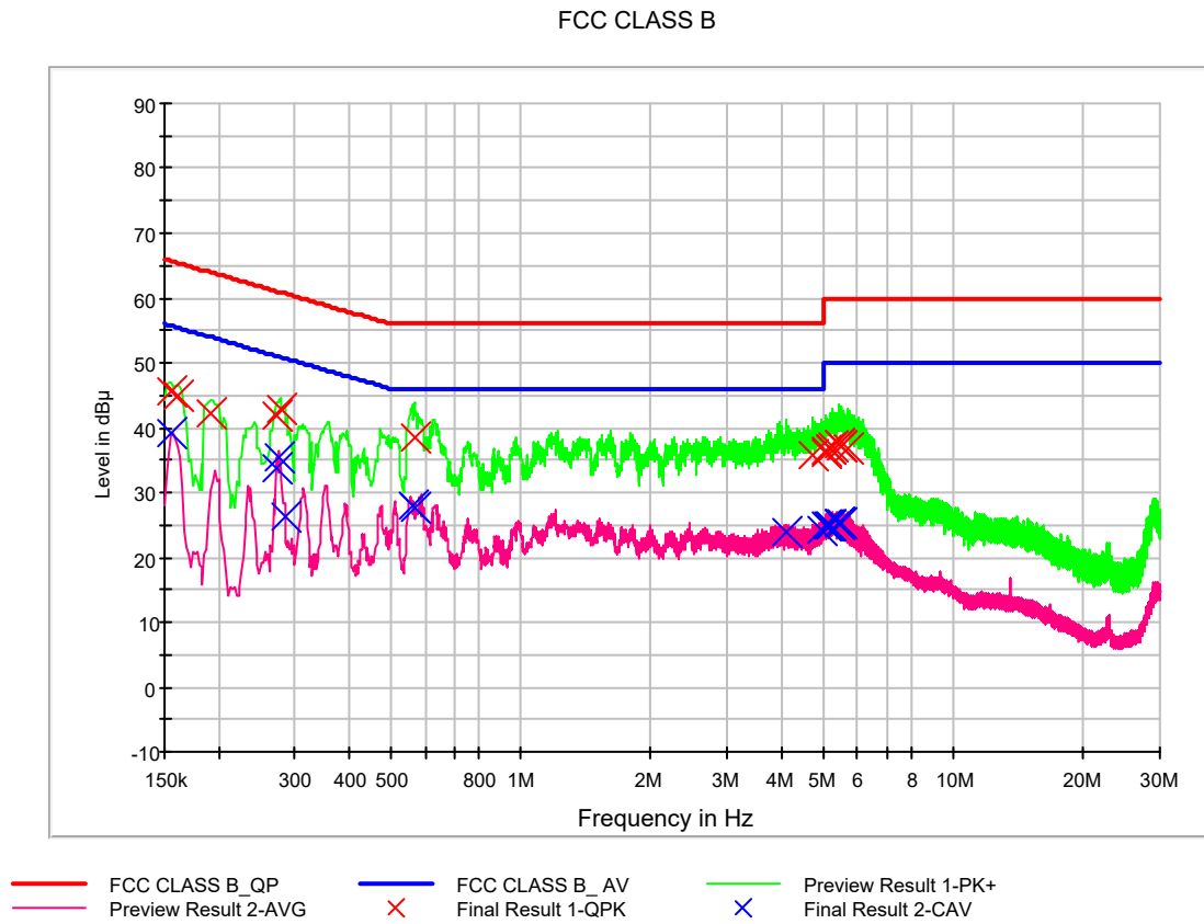
Figure 9: Conducted Emission, Charging + LTE BAND 25 RX Receiving mode, Line (L1)
