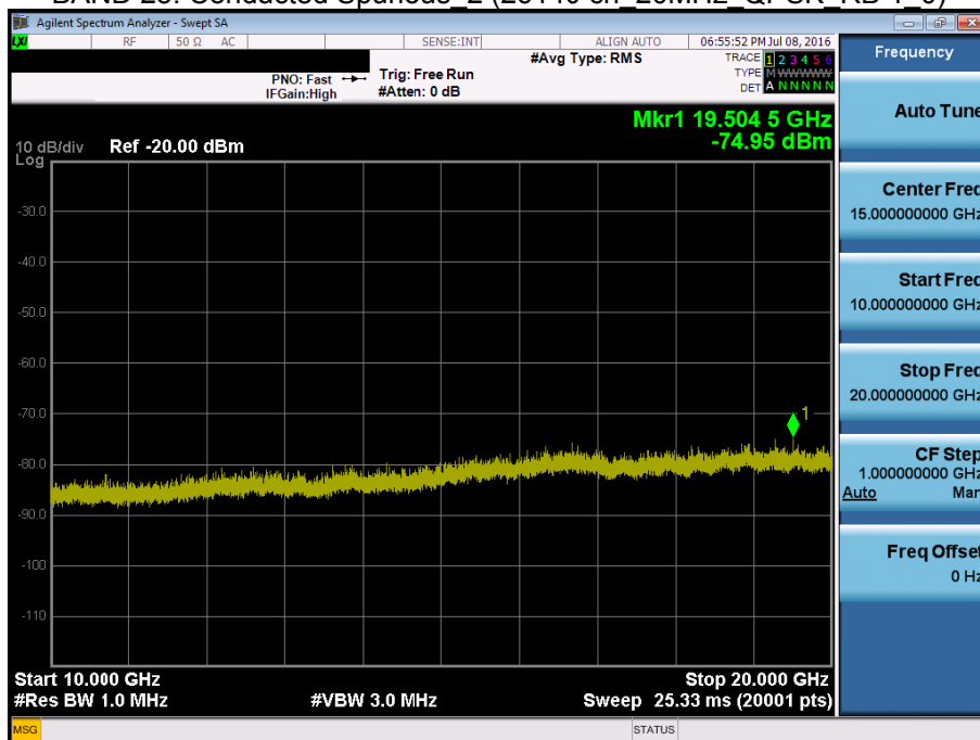
BAND 25. Conducted Spurious_2 (26140 ch_20MHz_QPSK_RB 1_0)
