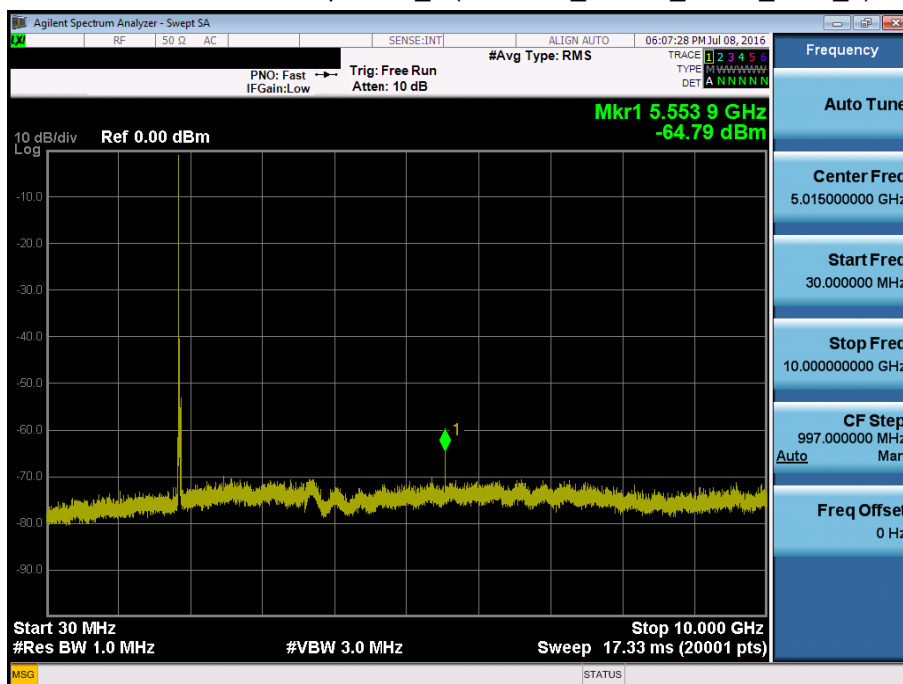
BAND 25. Conducted Spurious_1 (26140 ch_20MHz_QPSK_RB 1_0)
