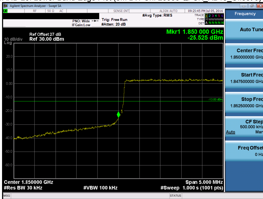
BAND 25. Lower Band Edge Plot (3M BW Ch. 26055 QPSK_RB15_Offset 0) -2
