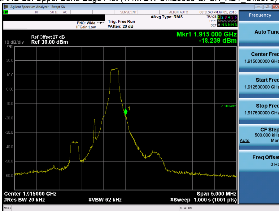
BAND 25. Upper Band Edge Plot (1.4M BW Ch.26683 QPSK_RB1_Offset 5) -1
