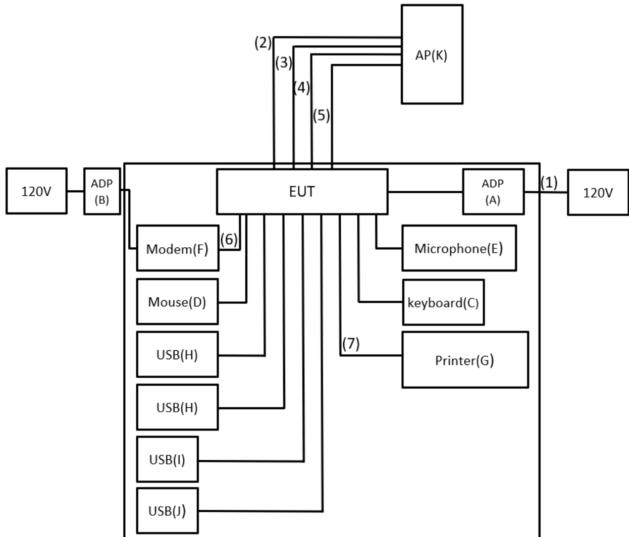
AC Power Line Conducted Emissions Test
