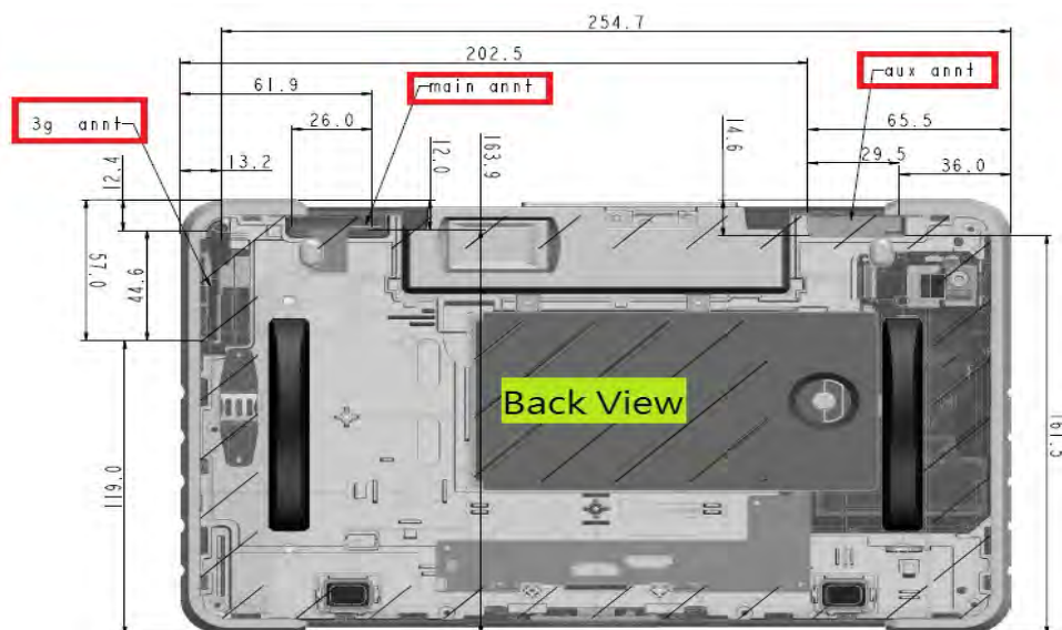
Antenna location
