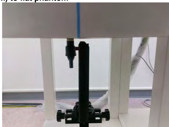
Fig.8 EUT Left side (10mm) to flat phantom
