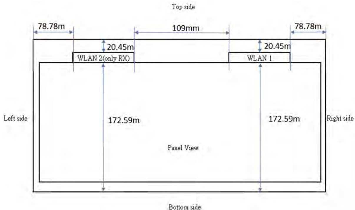
Fig.9 Antenna location of EUT
