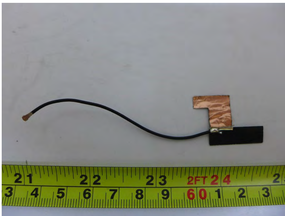
WLAN/BT Antenna
