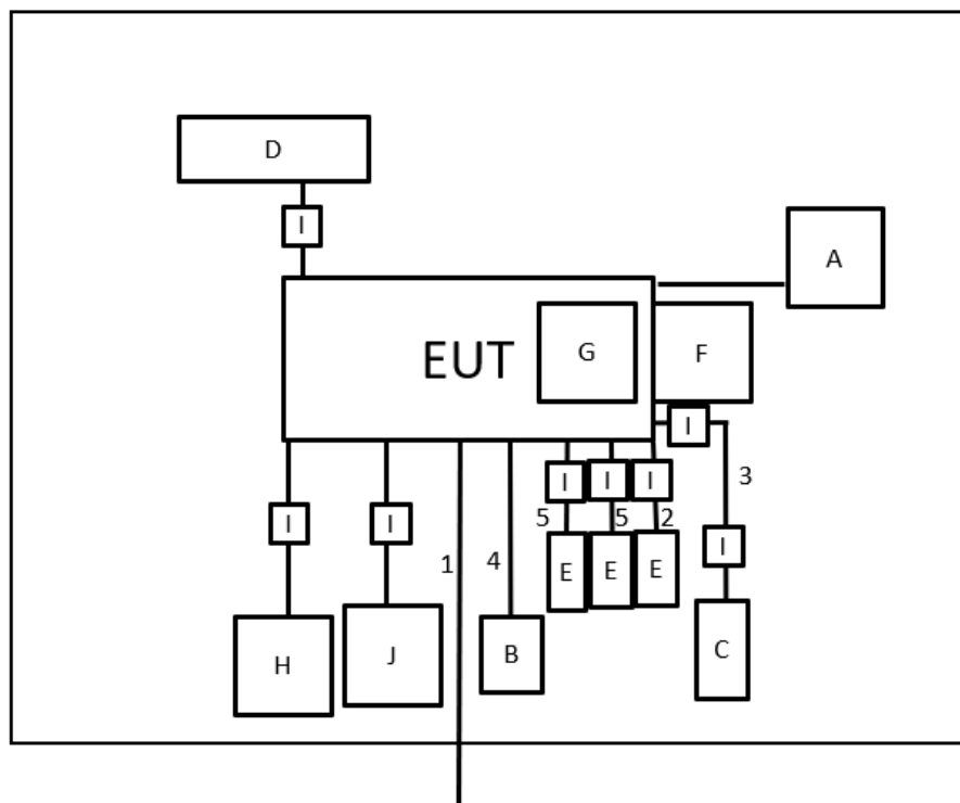
Radiated Emissions Test
