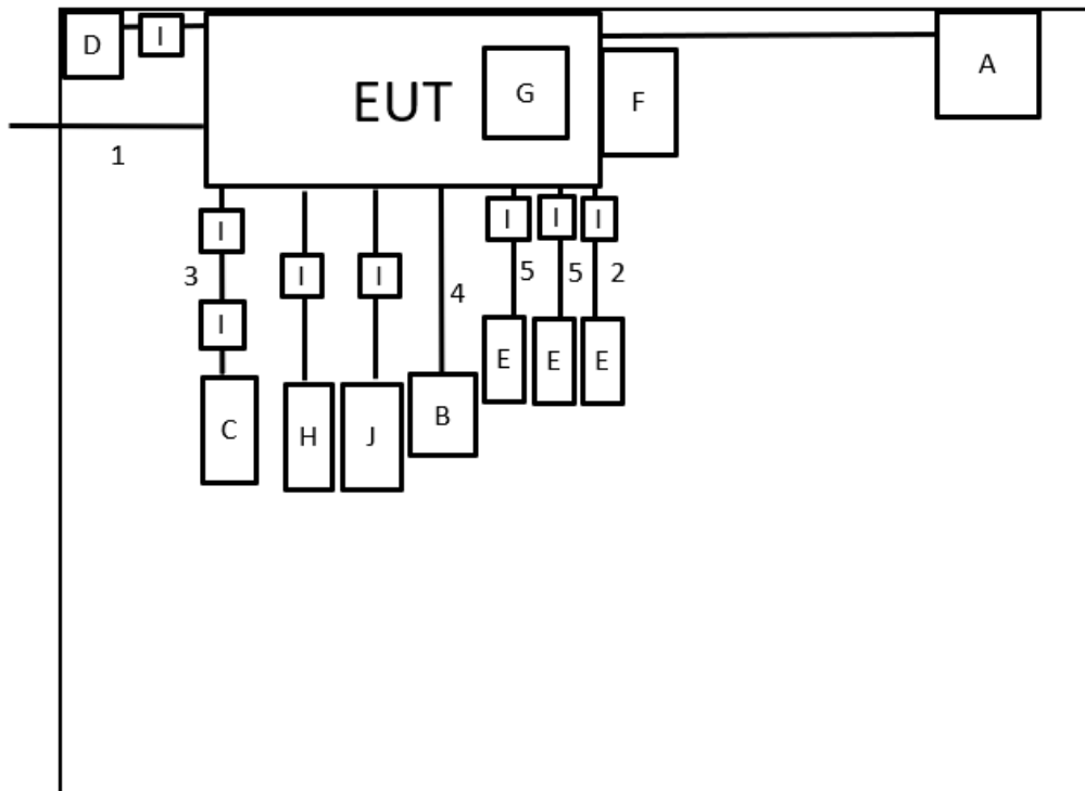
AC Power Line Conducted Emissions Test
