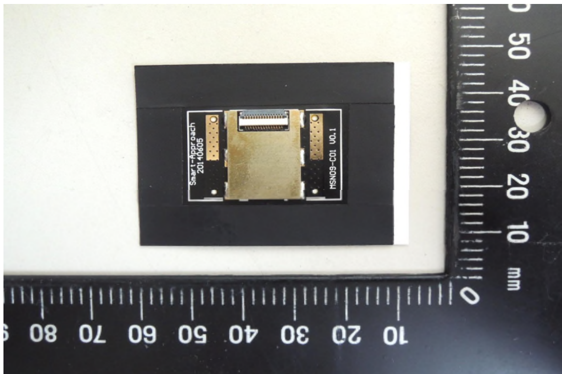
Internal View of EUT – 26
